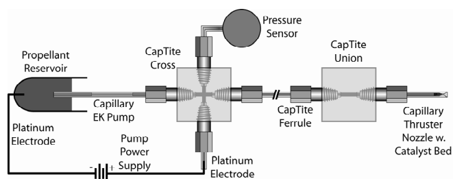
Fig. 4 Complete microthruster system assembly with CapTite™ fluidic interconnects, packed-bed capillary EK pump, and capillary thruster nozzle.
