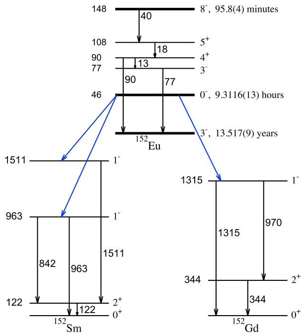
Figure 1. (Color online) Partial decay schemes of ^{152m1}\text{Eu} and ^{152m2}\text{Eu} . \gamma -ray energies and excitation energies are in keV.
