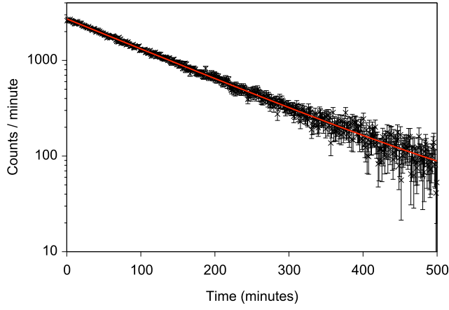
Figure 3. (Color online) The decay in intensity of the 90 keV \gamma ray which originates from the decay of ^{152m2}\text{Eu} . The red line shows an exponential fit to the data.
