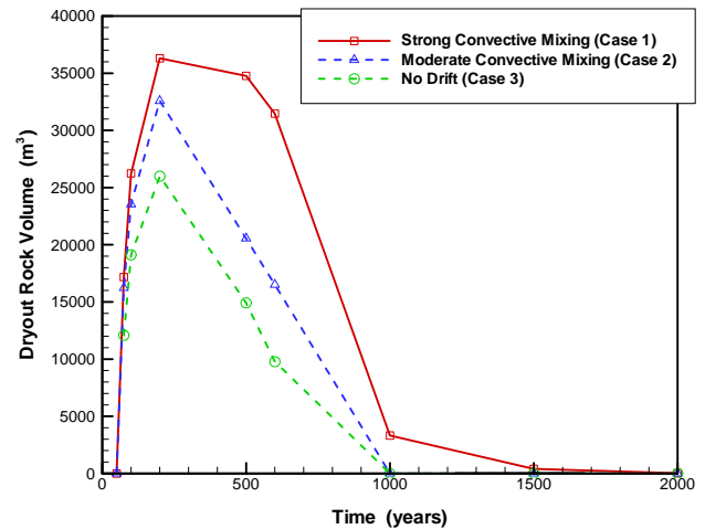
Fig. 6. Evolution of dryout volume of rock mass along heated drift section
