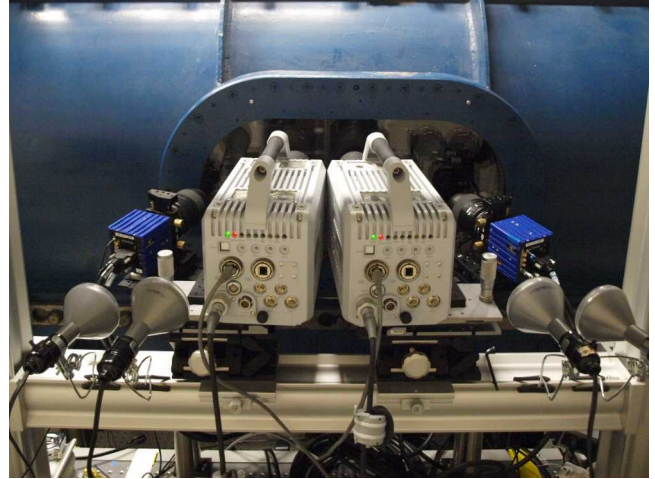
Figure 2: Two high-speed cameras aligned side-by-side for imaging an extended field of view, flanked by two sCMOS cameras for stereoscopic 10-Hz PIV.
