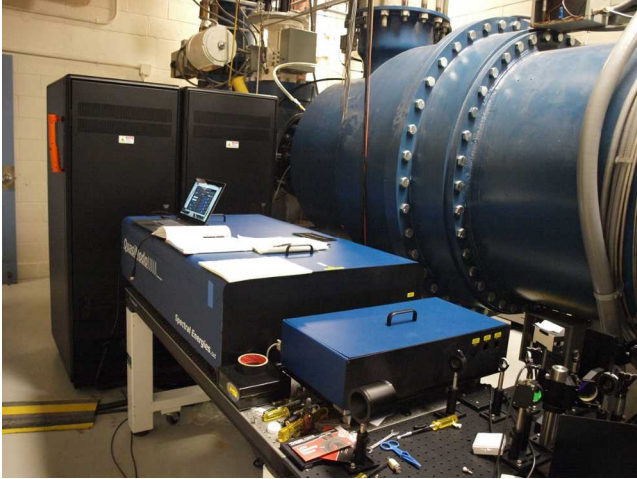
Figure 1: The pulse-burst laser installed adjacent to the Trisonic Wind Tunnel.
