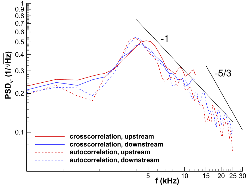
Figure 6: Power spectra of vertical velocity fluctuations found in the jet in crossflow, measured at an upstream location in the field of view ( x=258 mm, y=89 mm) and a downstream location ( x=313 mm, y=93 mm). Includes cross-correlation data at 25 kHz and auto-correlation data at 50 kHz.
