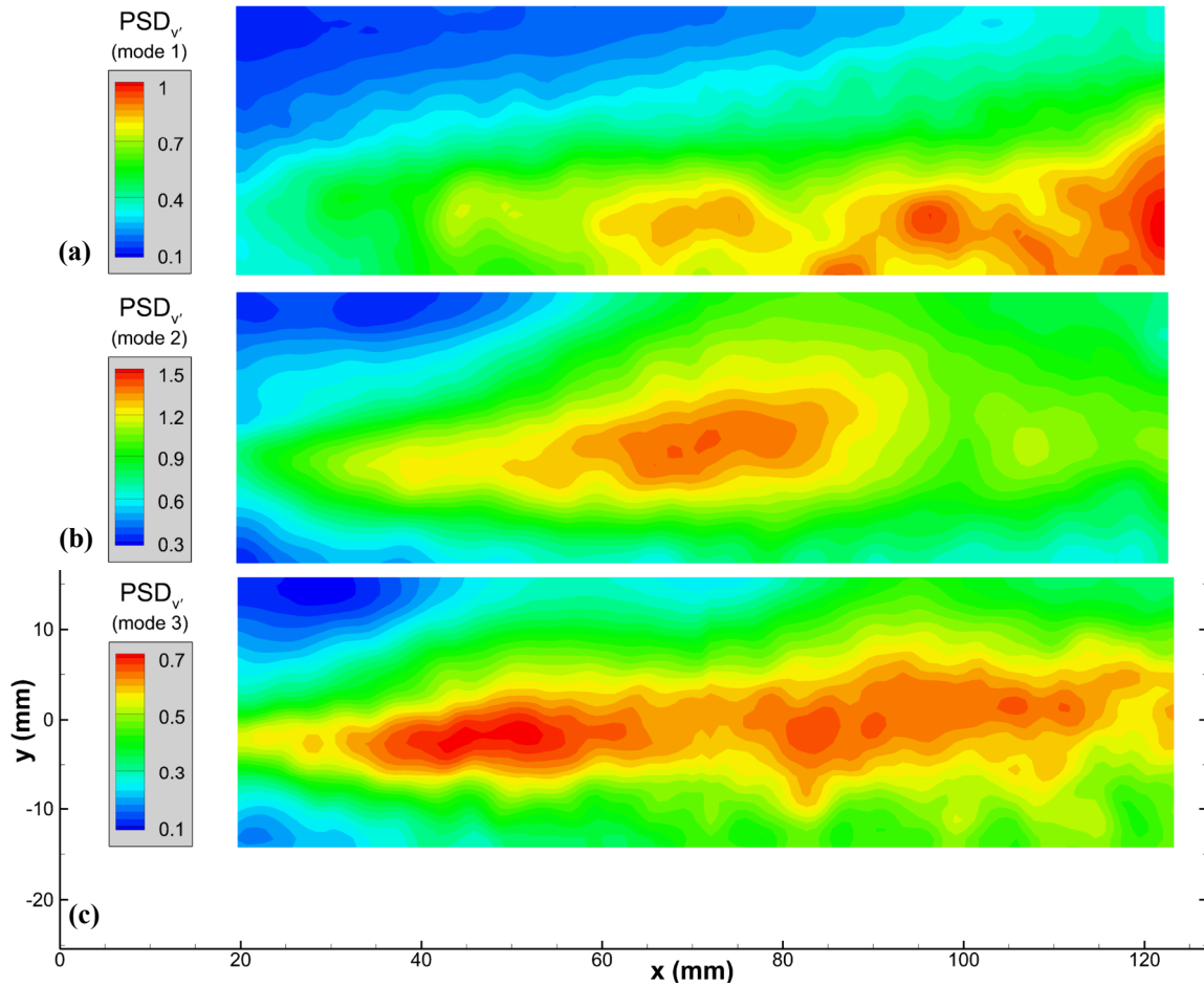
Figure 10: Spatial distribution of power spectral density amplitudes of vertical velocity fluctuations at specific frequencies corresponding to acoustic tones; (a) mode 1 ( f=620 Hz); (b) mode 2 ( f=1510 Hz); (c) mode 3 ( f=2380 Hz).
