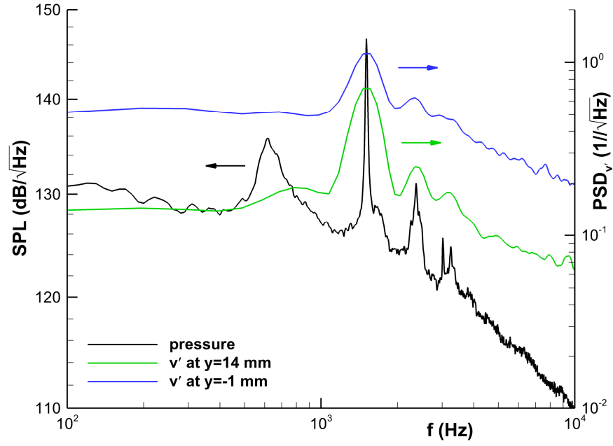
Figure 9: Power spectra of vertical velocity fluctuations found in the cavity flow, measured above the shear layer ( x=76.8 mm, y=14 mm) and within the shear layer ( x=76.8 mm, y=-1 mm). Also shown is a PSD of the pressure data measured by a sensor in the aft cavity wall at the spanwise center.
