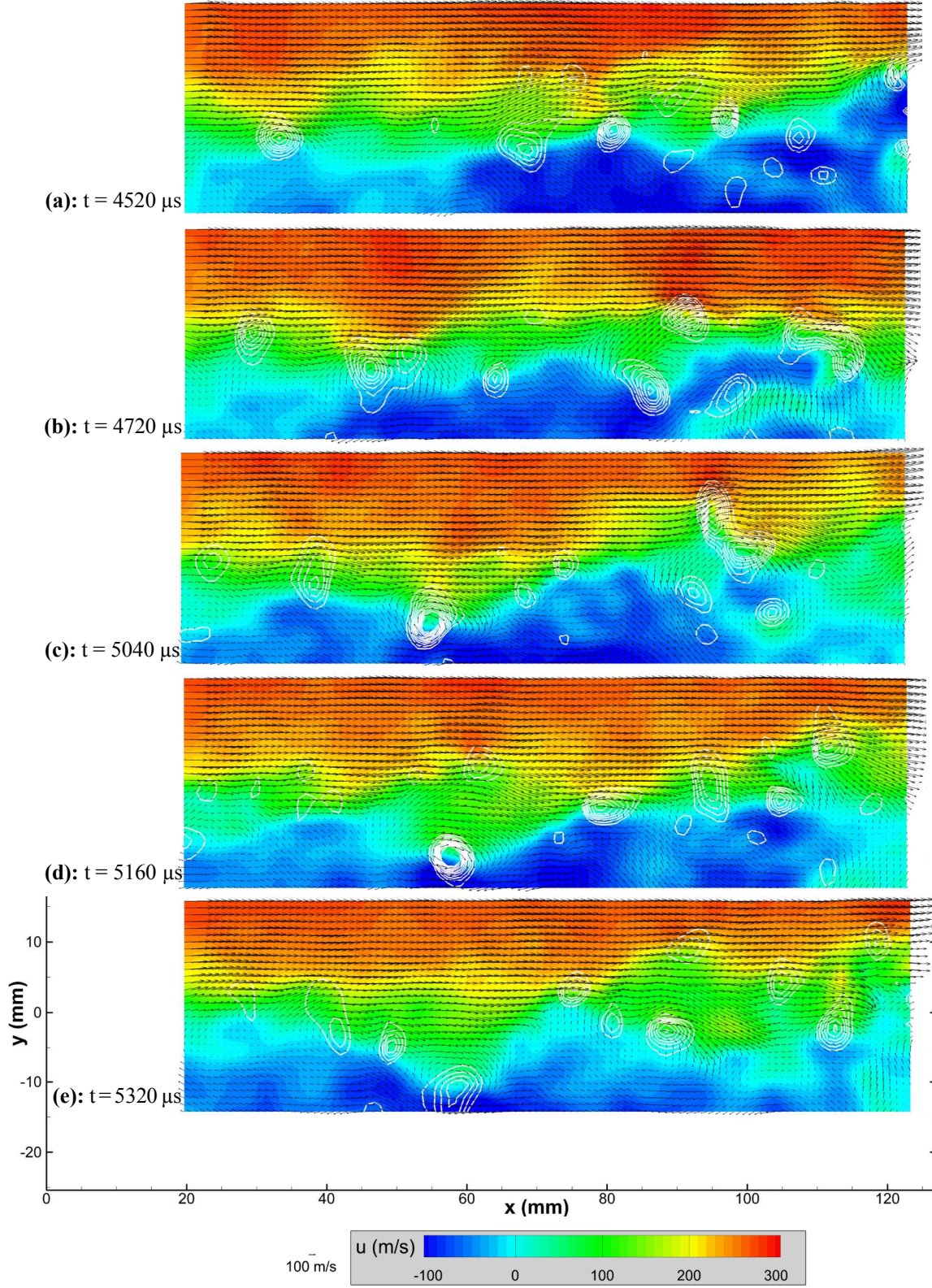
Figure 8: Sequence of velocity fields extracted from a 10.2 ms burst of 256 velocity fields acquired at 25 kHz, measuring flow over a rectangular cavity at Mach 0.8. Vectors show the in-plane velocity fluctuations superposed on a color contour plot of the streamwise velocity component and white line contours of the swirl field. The axes in (e) coincide with the positions of the cavity walls. Note that snapshots do not follow a uniform progression in time.
