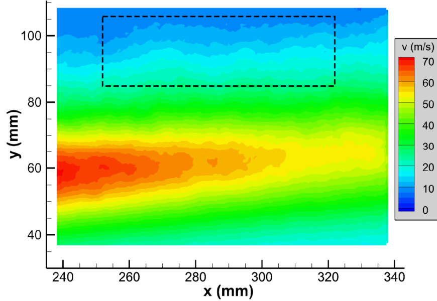
Figure 3: Mean vertical velocity component of the jet in crossflow at Mach 0.8 acquired using a traditional 10-Hz PIV system. The dashed rectangular box illustrates the field of view of the pulse-burst PIV.
