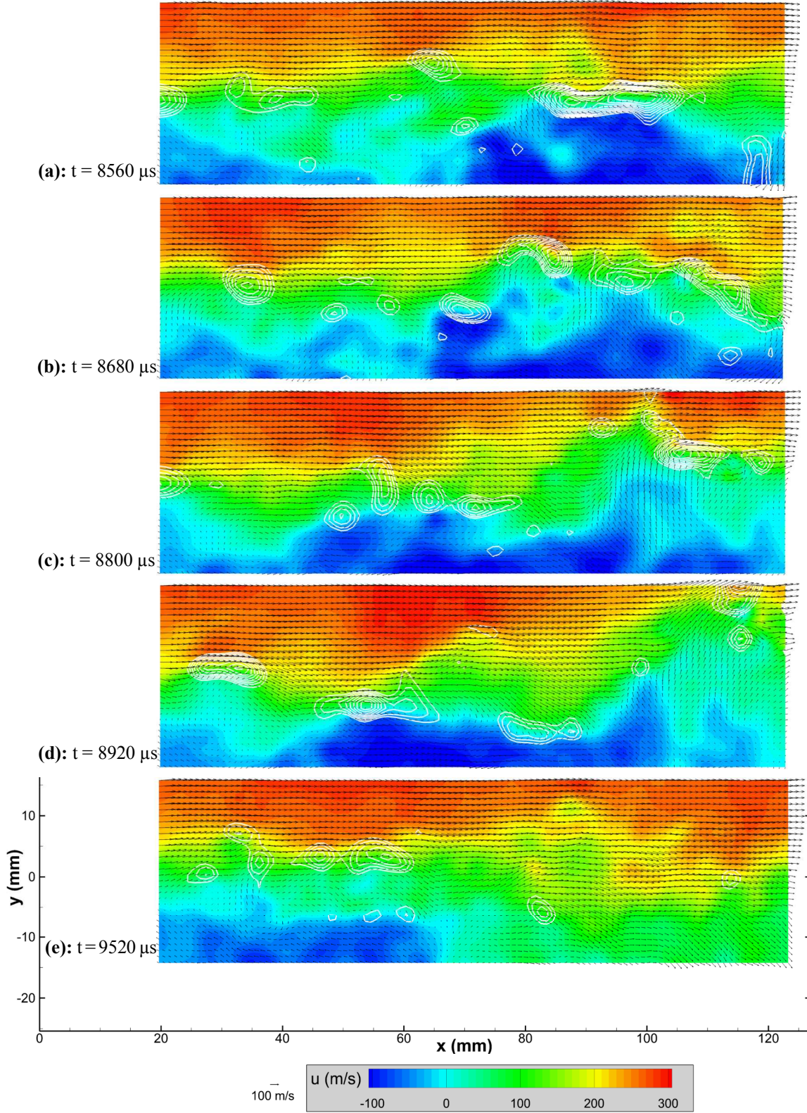
Figure 7: Sequence of velocity fields extracted from a 10.2 ms burst of 256 velocity fields acquired at 25 kHz, measuring flow over a rectangular cavity at Mach 0.8. Vectors show the in-plane velocity fluctuations superposed on a color contour plot of the streamwise velocity component and white line contours of the vorticity magnitude exceeding a minimum threshold. The axes in (e) coincide with the positions of the cavity walls. Note that (e) is a later-time snapshot out of progression with (a) – (d).
