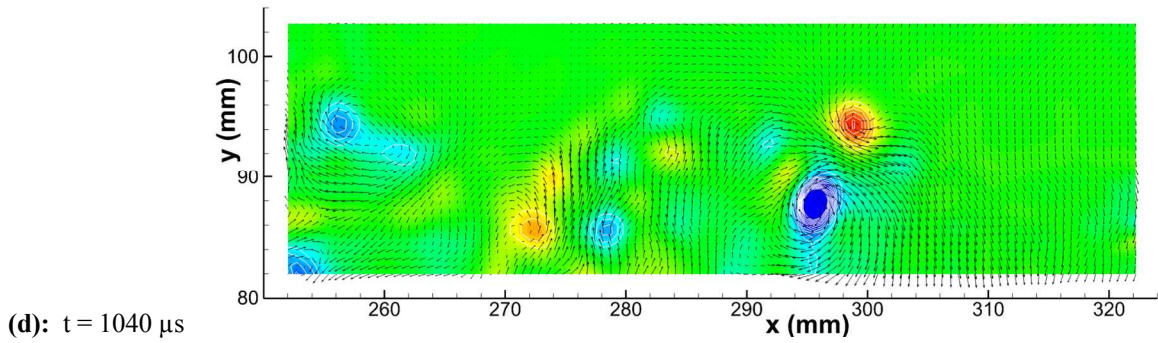
Figure 4: Sequence of eight velocity fields extracted from a 2.5 ms burst of 58 velocity fields acquired at 25 kHz, measuring a Mach 3.7 jet issuing into a Mach 0.8 crossflow at J=8.1 . Vectors show the in-plane velocity fluctuations superposed on a color contour plot of the derived vorticity field and white line contours of the swirl field. Continued on next page.
