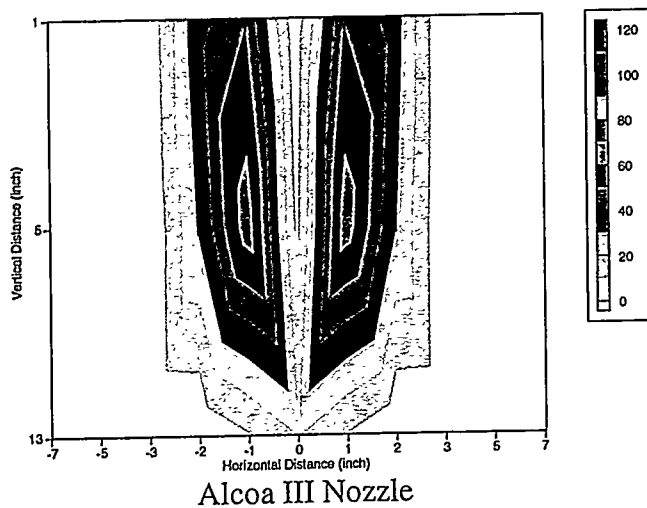
Figure 14 Dynamic Pressure Profiles
