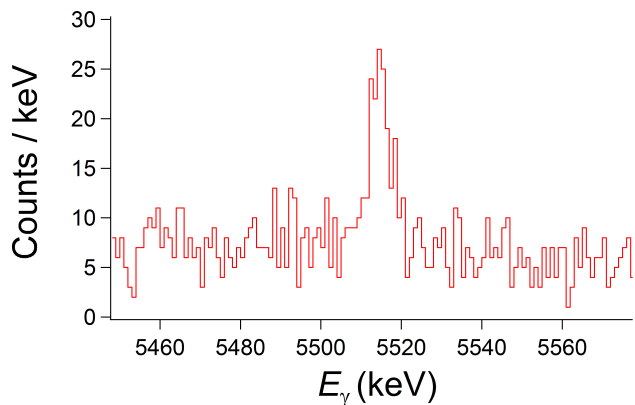
FIG. 3. (Color online) ^{20}\text{Mg} beta delayed gamma ray spectrum, with coincidence gating condition on the 984-keV ^{20}\text{Na} gamma ray peak (Figure 4), focusing on the 5514-keV peak.
