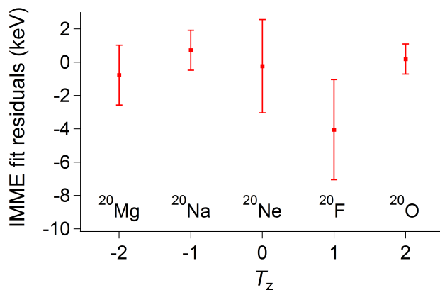
FIG. 5. (Color online) Residuals for the quadratic IMME fit (Equation 1) of the A = 20 , T = 2 quintet from the present work (Tables I and II). Previously, the uncertainty associated with the T_z = -1 member, ^{20}\text{Na} , was \pm 14 keV [3].
