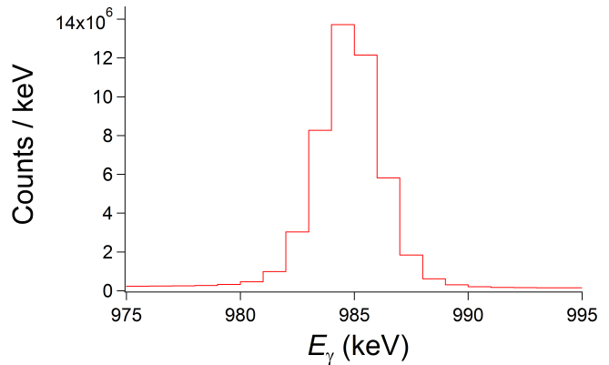
FIG. 4. (Color online) ^{20}\text{Mg} beta delayed gamma ray spectrum focusing on the 984-keV peak.
