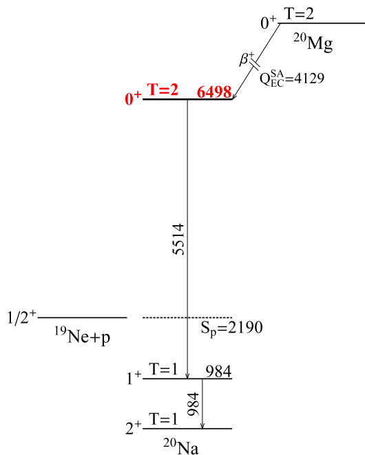
FIG. 1. (Color online) Simplified ^{20}\text{Mg} beta decay scheme focusing on the transitions relevant to the present work. Energies are shown in units of keV.
