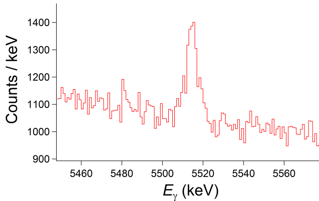
FIG. 2. (Color online) ^{20}\text{Mg} beta delayed gamma ray spectrum focusing on the 5514-keV peak.
