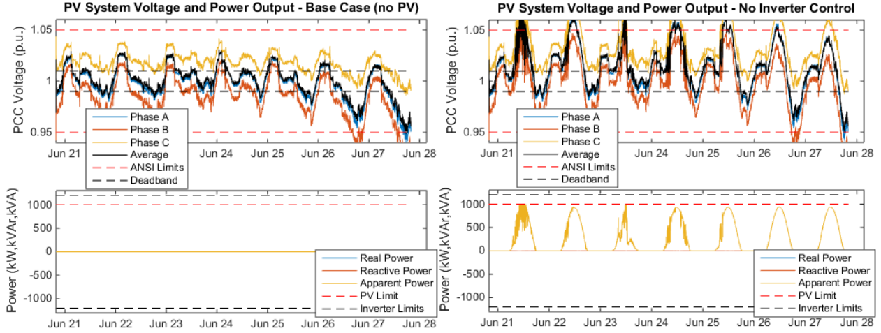
Figure 4. (left) Weekly simulation of end-of-feeder bus voltage and PV generation in the case of no PV and (right) with 1MW PV.
