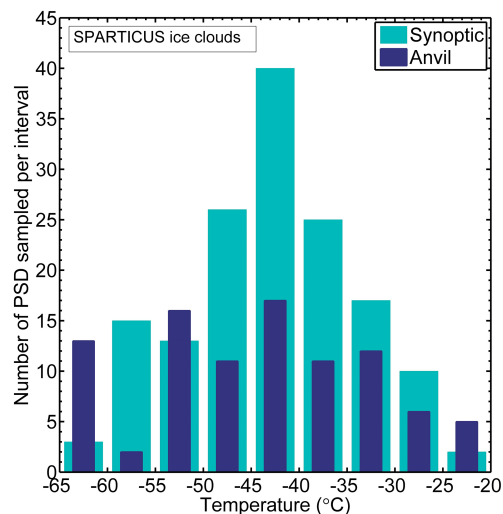
Figure 2. SPARTICUS PSD sampling statistics for synoptic and anvil cirrus clouds where the PSDs have been grouped into temperature intervals of 5^{\circ}\text{C} .
