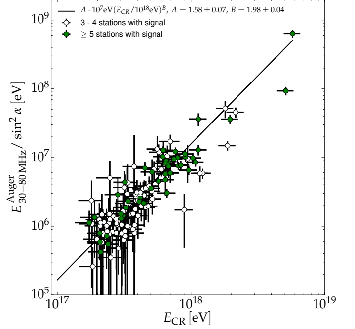
FIG. 2. Correlation between the normalized radiation energy and the cosmic-ray energy E_{\text{CR}} as determined by the Auger surface detector. Open circles represent air showers with radio signals detected in three or four radio detectors. Filled circles denote showers with five or more detected radio signals.
