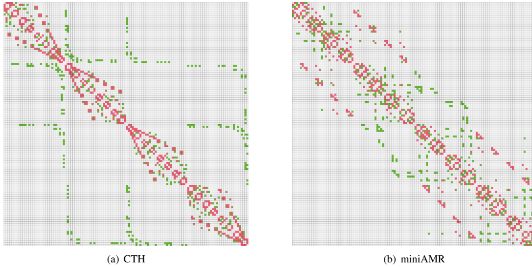
Fig. 6. Four spheres communication matrices
