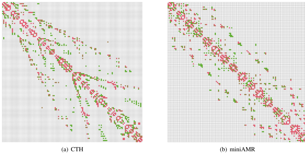
Fig. 7. Sphere hits block communication matrices
