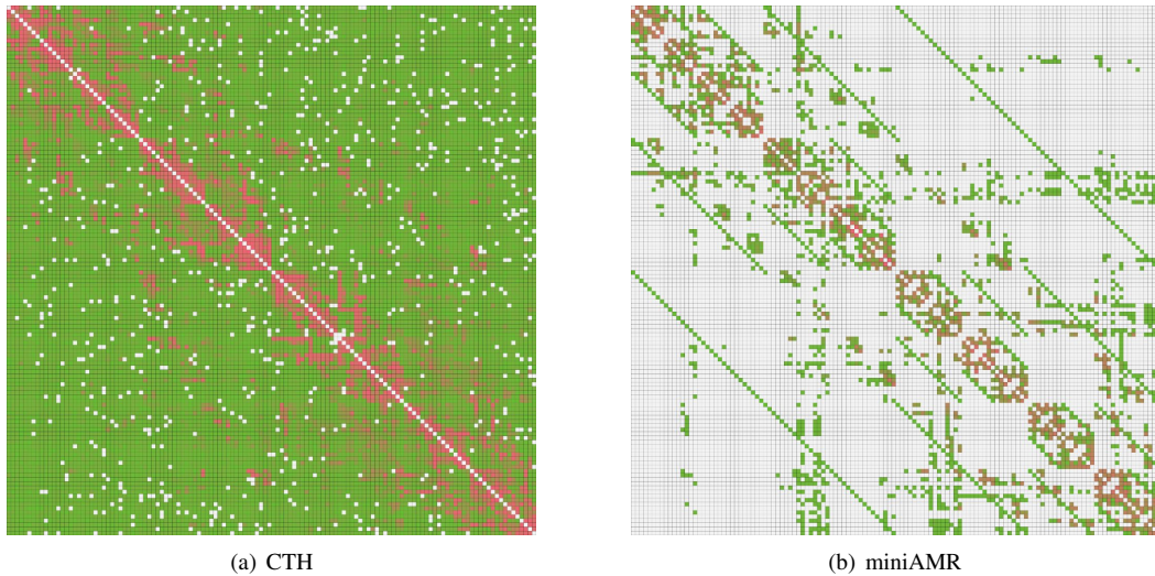
Fig. 9. Communication matrices for refinement
