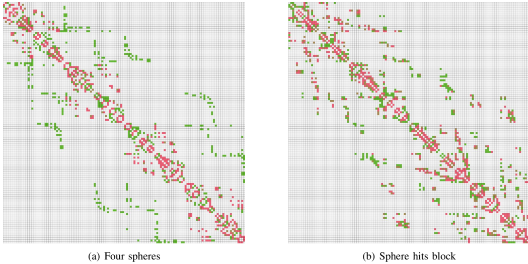
Fig. 8. Modified communication matrices miniAMR
