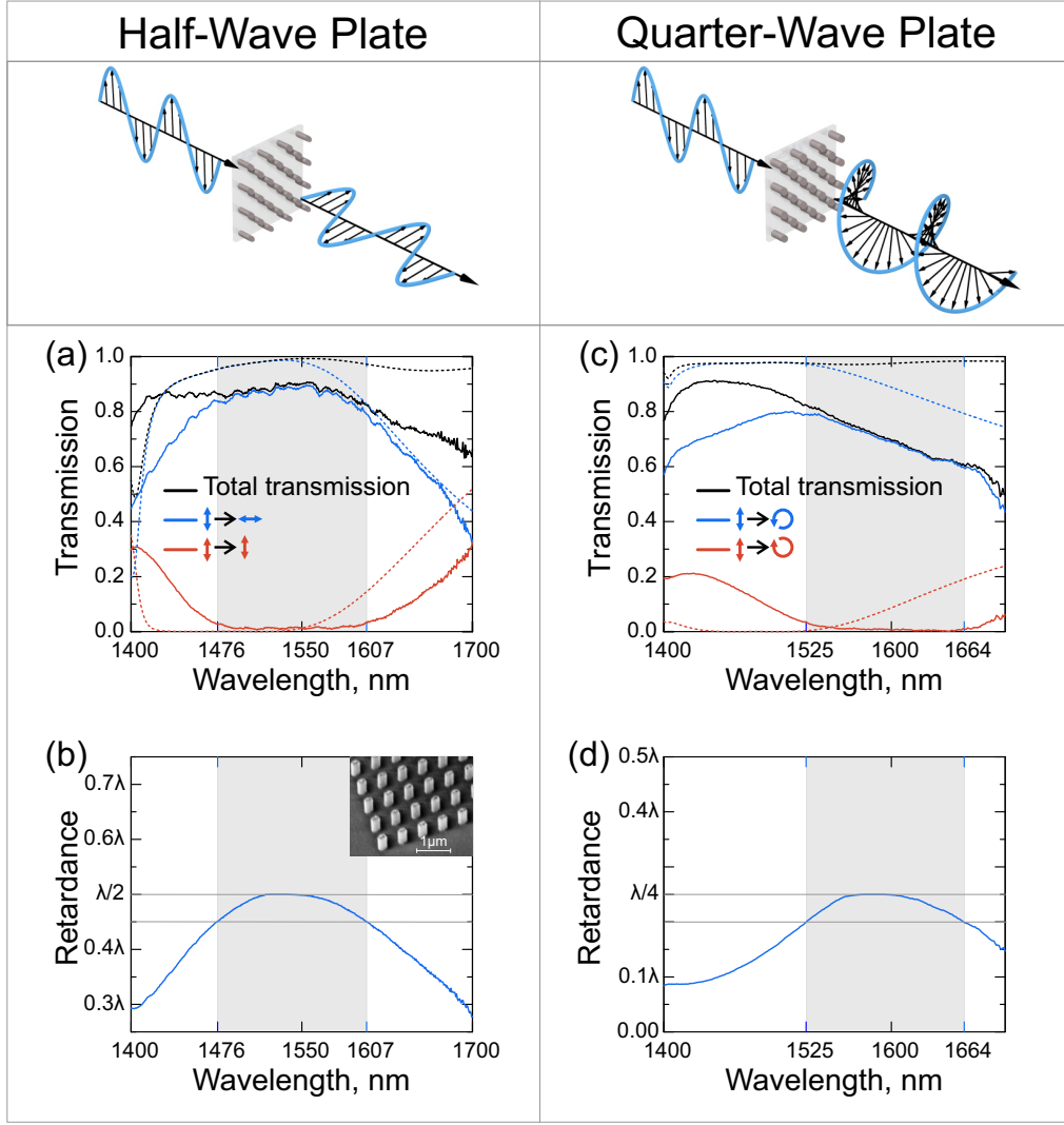
FIG. 4. Experimental demonstration of half- and quarter-wave plates. (a) Experimental and theoretical transmission spectra of the half-wave plate. Black line – total transmission. Red line – transmission through a metasurface positioned between a pair of linear parallel polarizer and analyzer with polarization axis oriented at 45^\circ to metasurface’s anisotropy axis. Blue line – transmission through a metasurface positioned between a pair of linear crossed polarizer and analyzer with polarization axis oriented at \pm 45^\circ to metasurface’s anisotropy axis. Solid lines – experimental data, dashed lines – theoretical results. (b) Experimentally retrieved retardance of the half-wave plate. Highlighted region shows the spectral range, with a deviation from \lambda/2 by no more than 10%, or \lambda/20 . Inset shows a scanning electron micrograph of the fabricated half-wave plate. (c) Experimental and theoretical transmission spectra of the quarter-wave plate. Black line – total transmission. Red line – transmission through a metasurface positioned between a pair of linear polarizer with polarization axis oriented at 45^\circ to metasurface’s anisotropy axis and a right-circular analyzer. Blue line – transmission through a pair of linear polarizer with polarization axis oriented at 45^\circ to metasurface’s anisotropy axis and a left-circular analyzer. Solid lines – experimental data, dashed lines – theoretical results. (d) Experimentally retrieved retardance of the quarter-wave plate. Highlighted region show the spectral range, with retardance deviation from \lambda/4 by no more than \lambda/20 .
