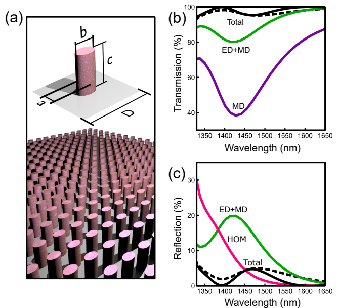
FIG. 2. (a) Schematic of our broadband metadvice. The spectra in (b) and (c) show the transmission and reflection of the metadvice and their dependence on the multipoles (ED = electric dipole, MD = magnetic dipole, and HOM = sum of higher-order multipoles). The black dashed curves in (b) and (c) show transmission and reflection from a complete set of multipoles, which neglects reflection off the glass substrate, and the black solid curves show the direct numerical transmission and reflection. Dimensions are a = 285 nm, b = 450 nm, c = 860 nm and D = 750 nm, and the incident polarization is parallel to the short axis of the nanopillars.
