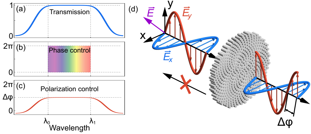
FIG. 1. Concept of a broadband highly-efficient metadvice. (a) Near-unity energy efficiency over a broad spectral region. (b) Phase coverage in the range [0 - 2\pi] . (c) Phase difference for two orthogonal polarizations in the range [0 - \pi] . (d) Schematic of a metadvice for spatially-variant polarization control operating in a broad spectral range.
