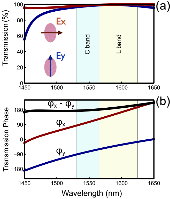
FIG. 3. (a) Transmission spectrum of the metadevice shown in Fig. 2, for polarizations parallel to the two axes of the nanopillar. (b) Phase of the transmitted waves with respect to the incident field for both orthogonal polarizations. The phase difference \varphi_x - \varphi_y shows a constant value of \pi over a broad spectral range, as required for a broadband half-wave plate.
