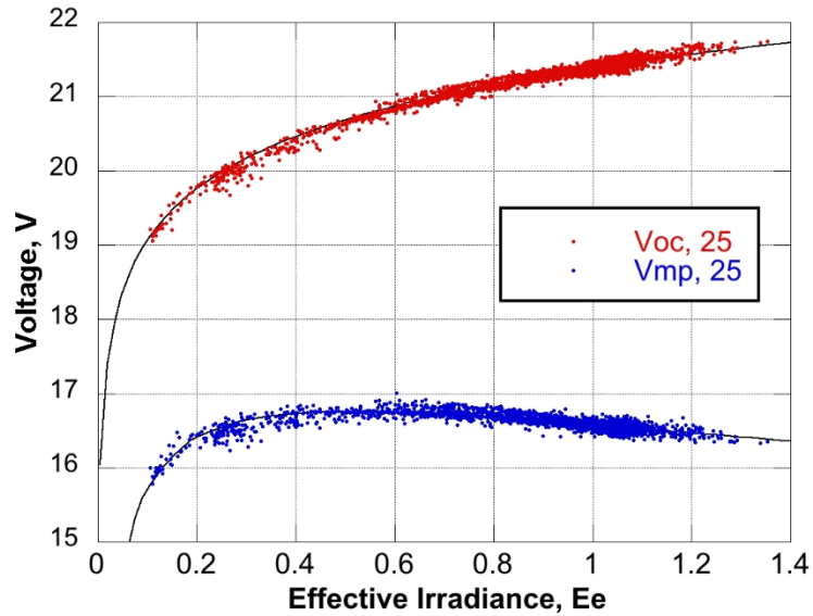
Figure 21. Voltages adjusted to 25°C as a function of Effective Irradiance.
