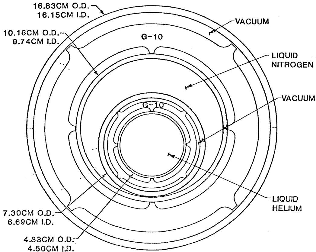
Figure 1. Transfer Line Cross-Section
