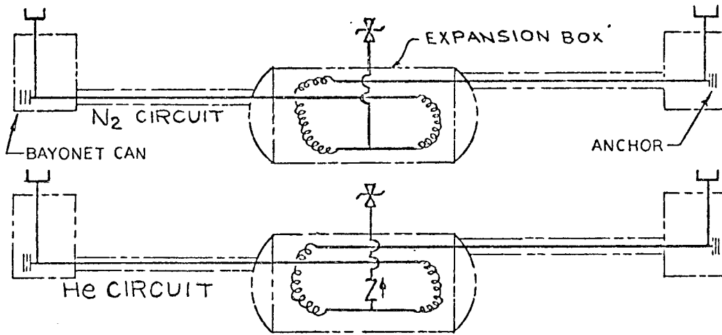
Figure 2. One Section Tevetron Feed Line(1/25 Ring)
