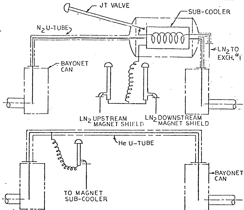
Figure 3. One Pair Tevetron U-Tubes
