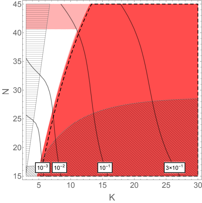
FIG. 5. Bounds on multiple PQ field model for m_{\tilde{S}}^2 = 10^{-12}M_P^2 . All curves are the same as in Fig. 4.
