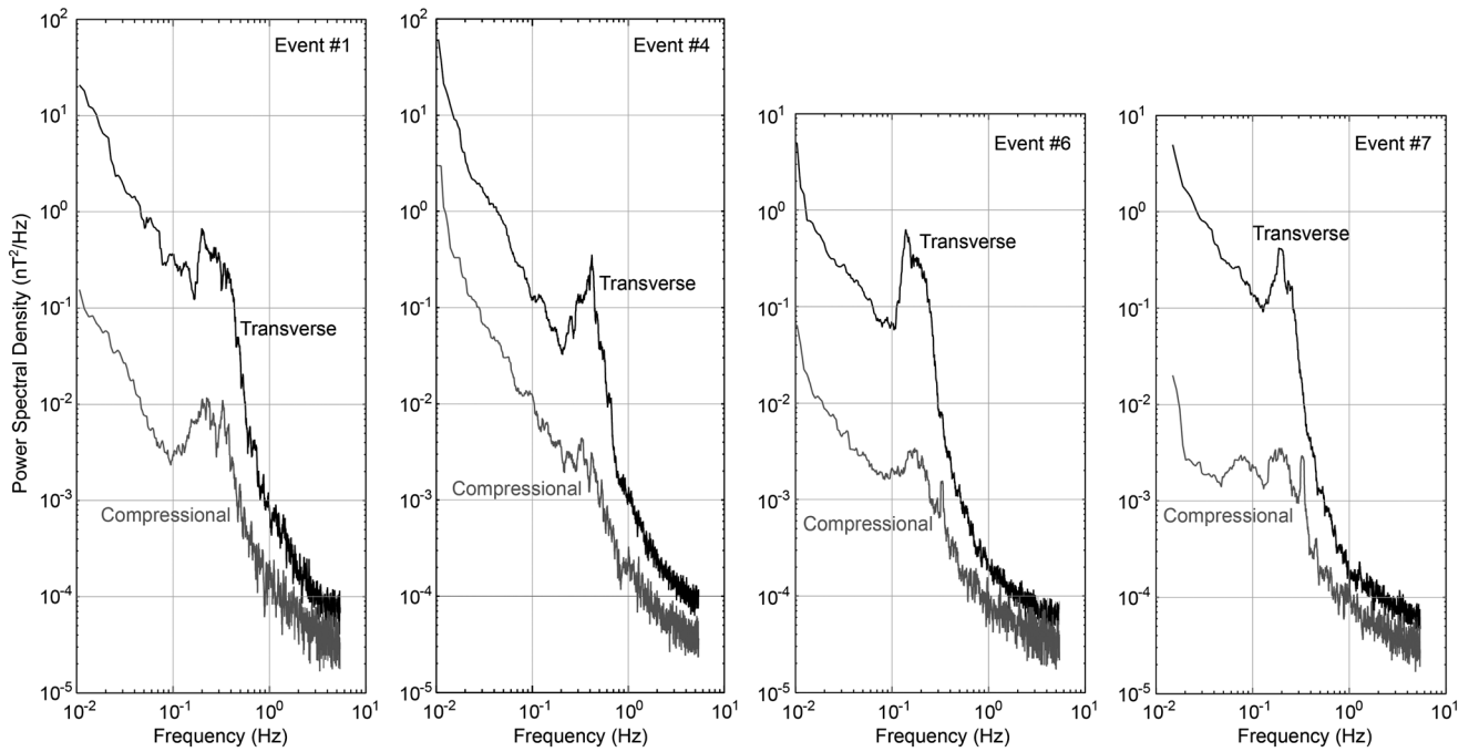
Figure 3. The magnetic fluctuation power spectra during Events #1, #4, #6, and #7 observed from the Wind spacecraft on 19 March 2005.
