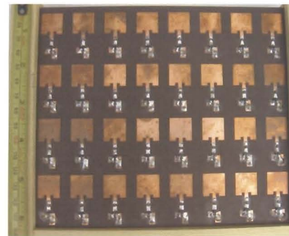
Figure 7 Thirty-two element, 5.8 GHz rectenna array designed at LANL
