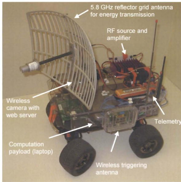
Figure 10 The mobile-host RC vehicle and its component
