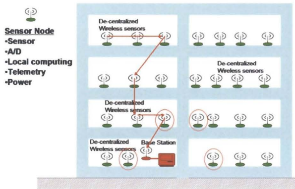
Figure 2 De-centralized wireless SHM system with Hopping connection
