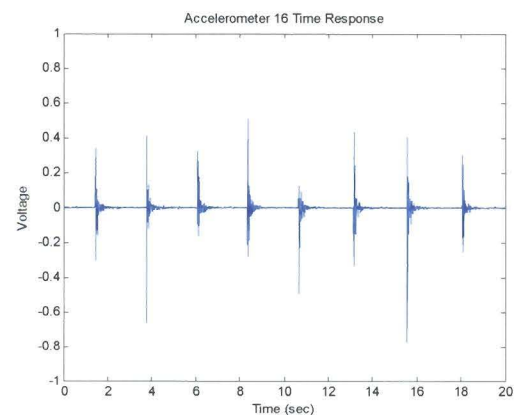
Figure 23. Time response measured by an accelerometer under the impact loading
