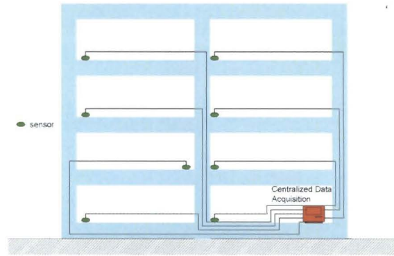
Figure 1. The wired sensing network
