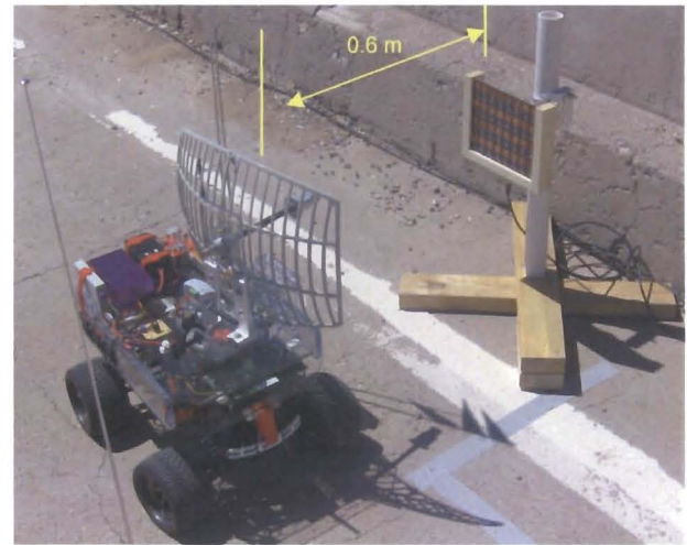
Figure 17 Setup of RF transmission at the bridge.
