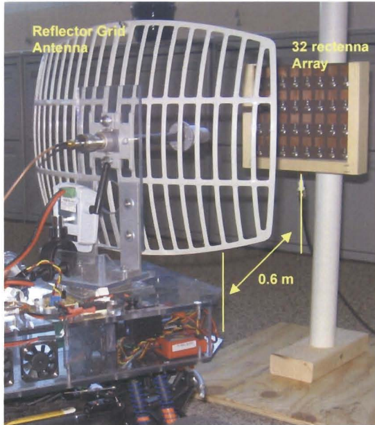
Figure 8 Laboratory experiment designed to test the thirty-two element rectennas
