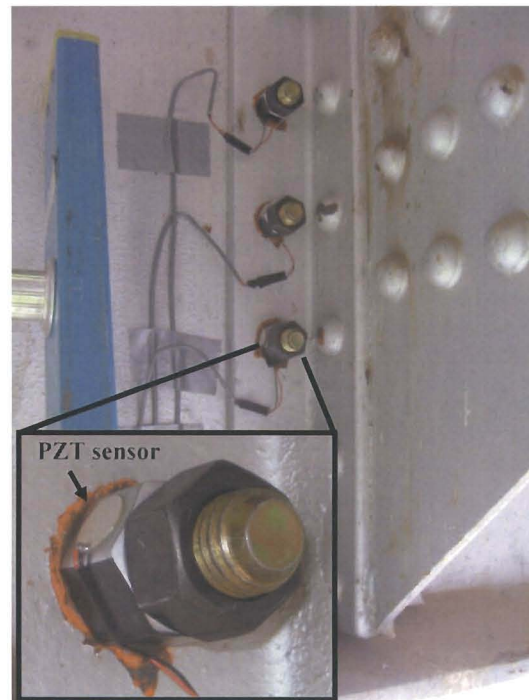
Figure 13. Instrumented bolts mounted to the girder of the Alamosa Canyon Bridge. Preload was monitored with the PZT sensors using WID sensor nodes.
