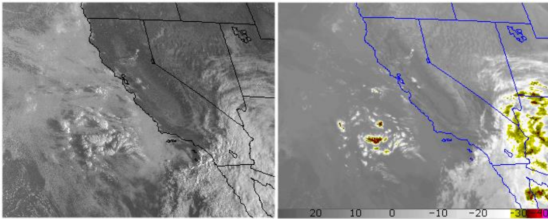
Figure 10: Example GOES visible (left) and infrared (IR) (right) satellite images from 10/7/2014 at 06:45 LST. The IR channel enhanced temperature (°C) scale is shown on the bottom of the IR image. Lower, warmer marine layer clouds are clearly observed in the visible GOES imagery but are hard to distinguish in the IR GOES imagery. Higher, colder clouds are better discernable in IR satellite images due to the thermal contrast present between the colder cloud tops and the warmer land surface.
