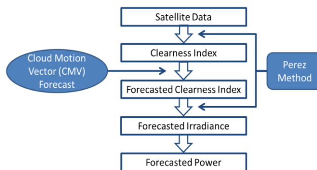
Figure 4: SolarAnywhere satellite-based power forecasting process flowchart.
