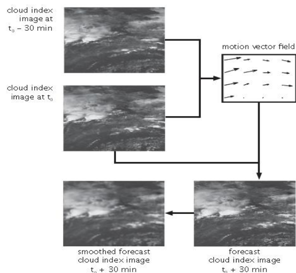
Figure 3: Example CMV technique derived from two consecutive visible satellite images (from Lorenz et al., 2004). Infrared-based CMV forecasts are derived in a similar fashion from consecutive IR satellite images.
