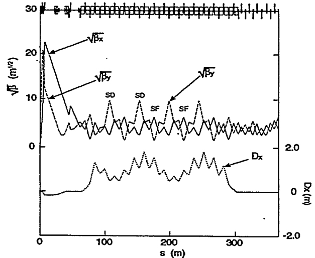
Figure 4. Lattice functions for sextant 2-4 showing the perturbed beta functions in arc 3.
