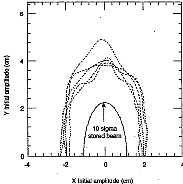
Figure 5. Dynamic aperture of the HER using 5 seeds for alignment and multipole errors. Particles are stable for initial amplitudes within the curves shown.
