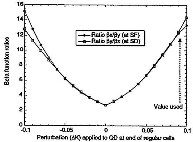
Figure 3. The ratio of the vertical and horizontal beta functions as a function of the quadrupole perturbations.
