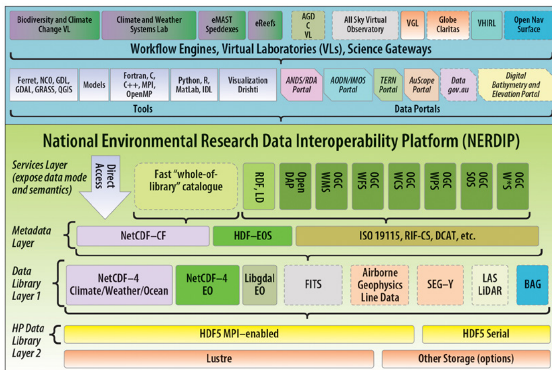
Fig. 7. NERDIP architecture.
