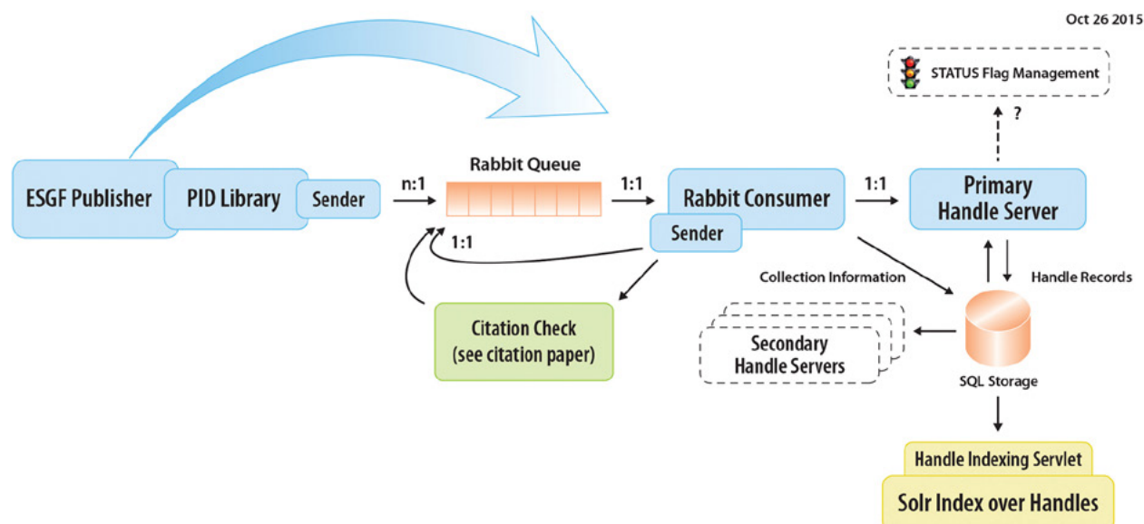
Fig. 26. Basic architecture of ESGF PID services with queueing system and Handle server.
