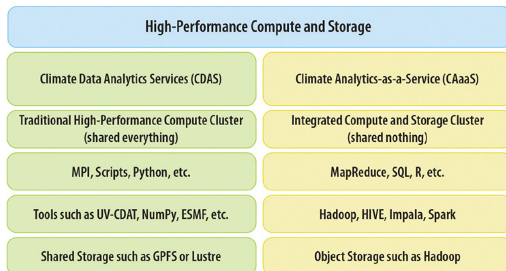
Fig. 17. Comparison of back-end implementations.
