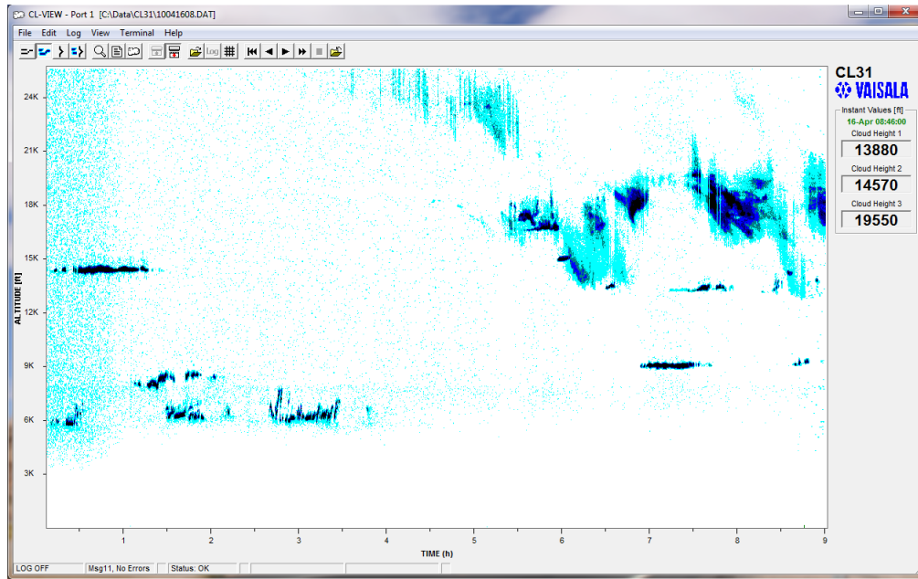
Figure 1. CL-View cloud intensity graph (0 – 25500 ft AGL).
