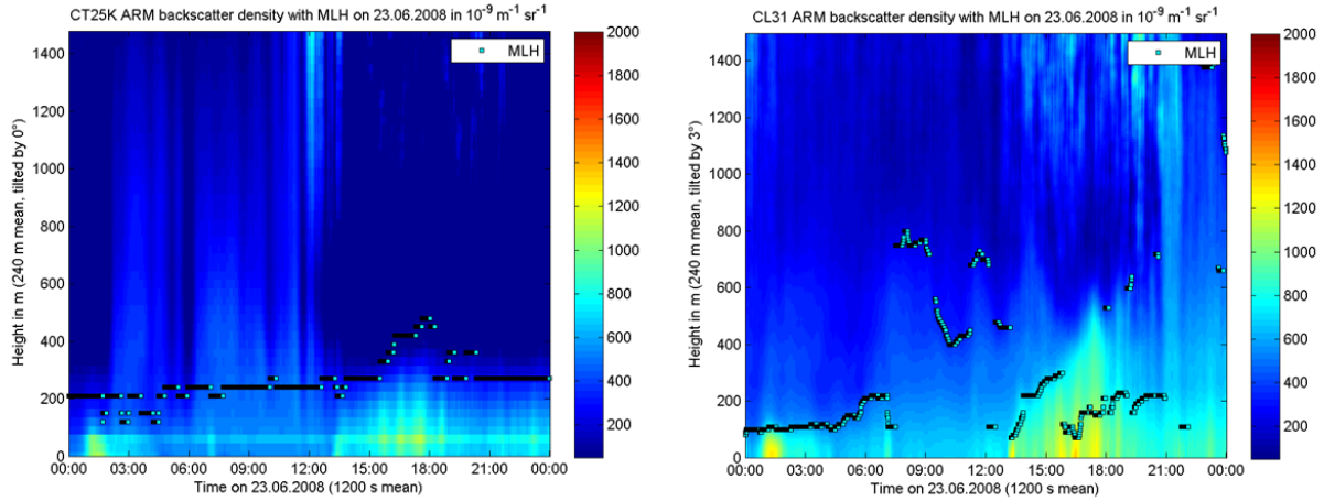
Figure 3. Backscatter density in 10^{-9} \text{ m}^{-1} \text{ sr}^{-1} with mixing-layer-height in m from Vaisala CT25K and CL31 Ceilometers on 06/23/2008 at SGP.
