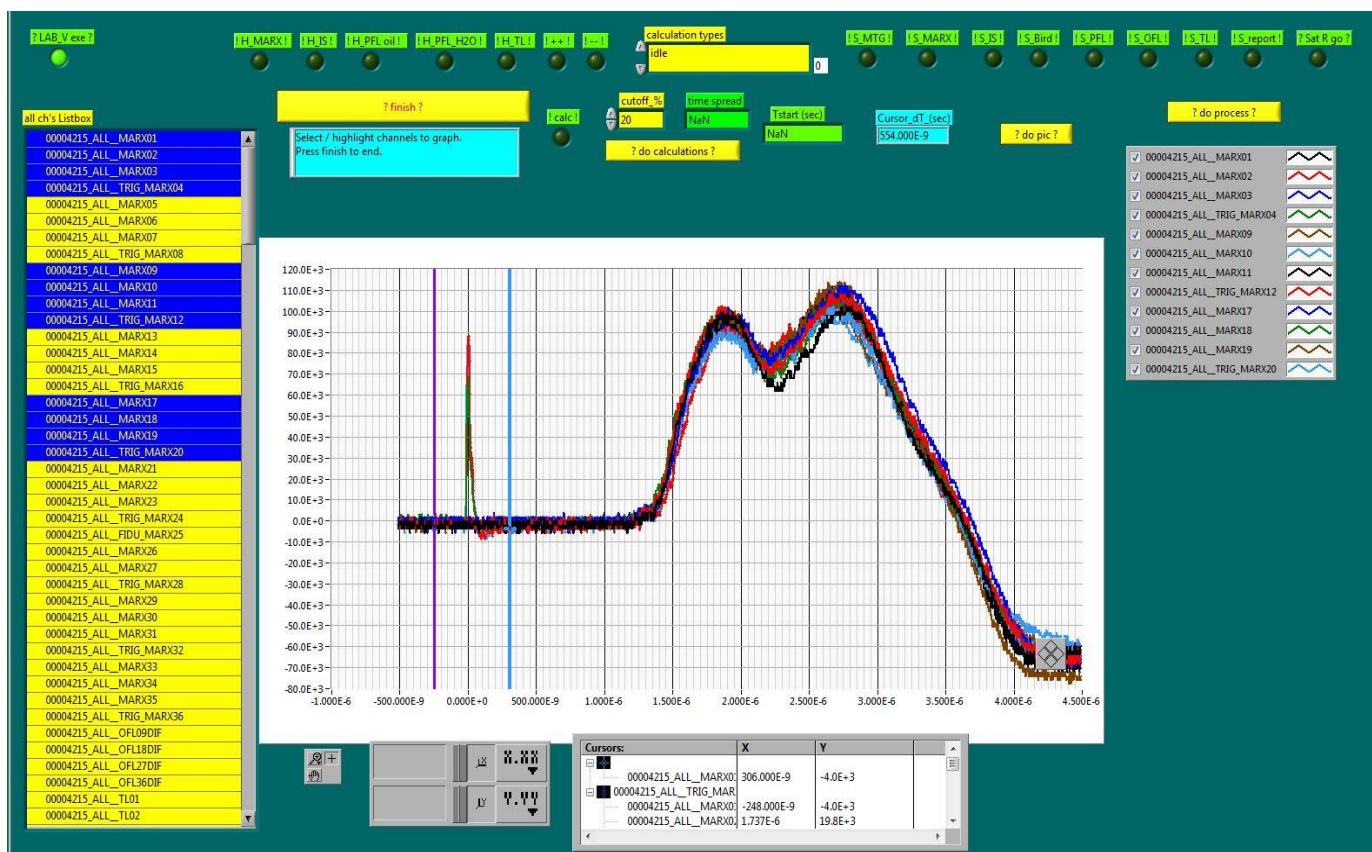
Fig. 5 Screen shot of data viewer with automatic time correction. The main image display is for data plotting, shown here are some Marx CVR probe signals from Saturn # 4215.
