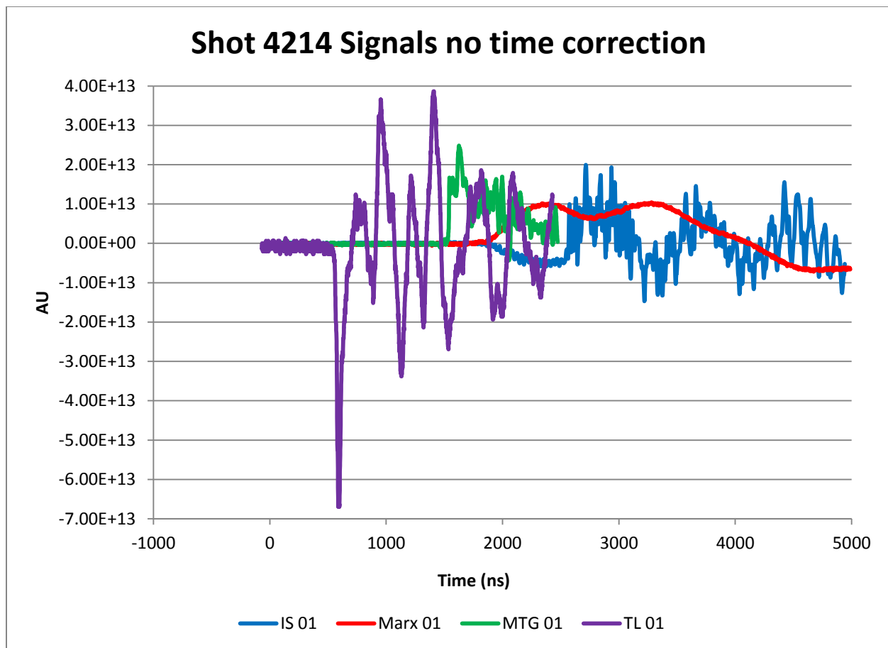
Fig. 3 Saturn shot 4214 module 1 signals, no time correction.
