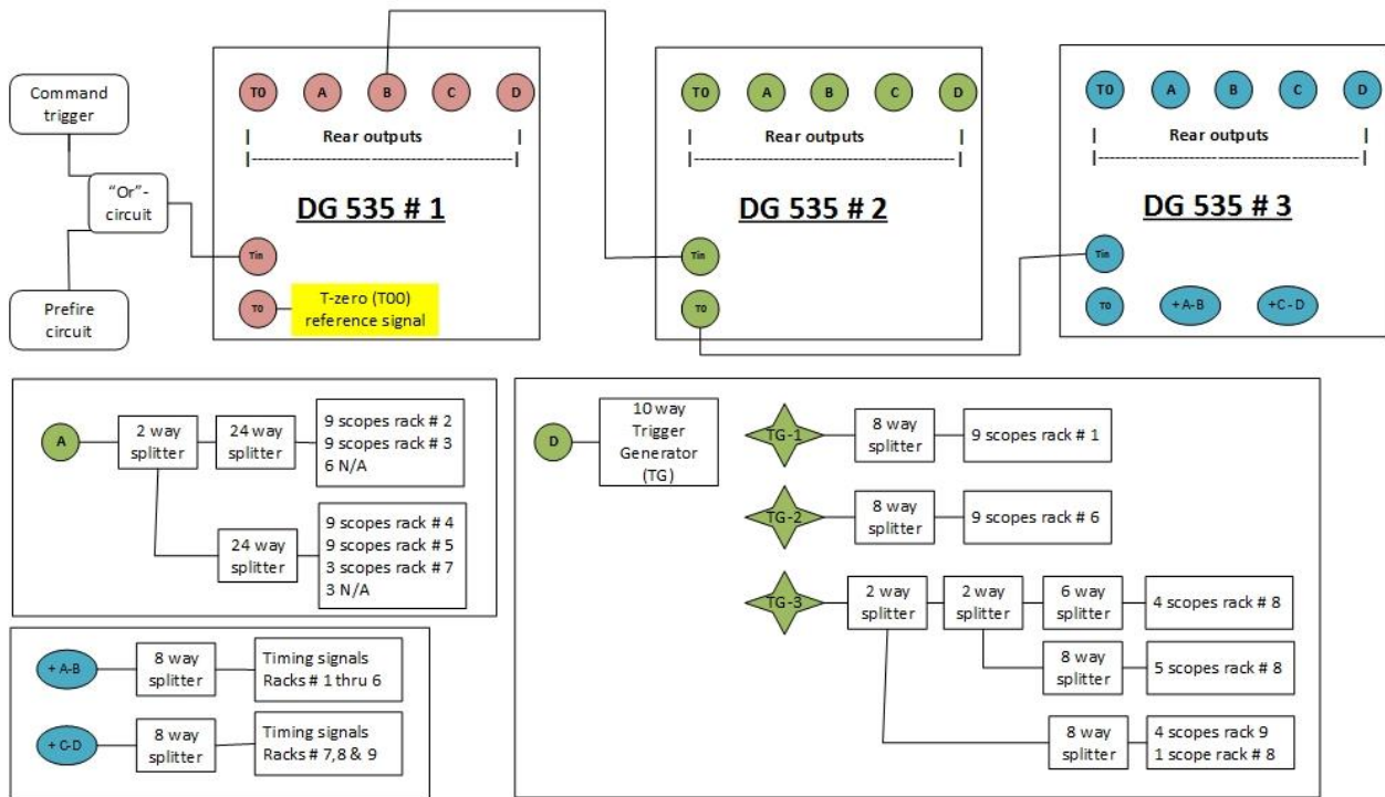
Fig. 2 Saturn Main DAQ scope trigger circuit.
