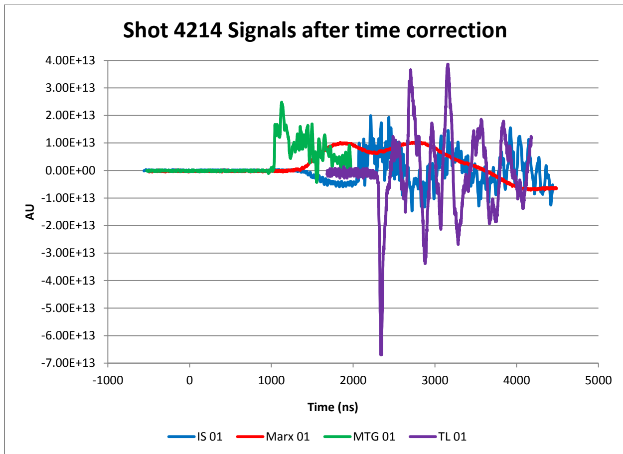
Fig. 4 Saturn shot 4214 module 1 signals after time correction.
