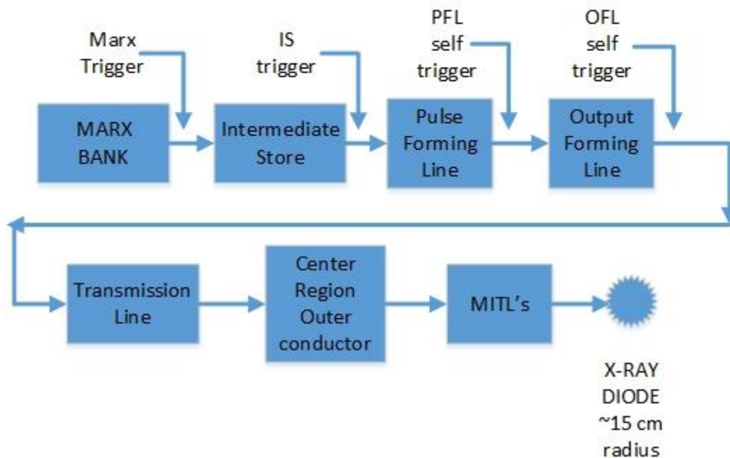
Fig. 1 Block diagram of Saturn module (1 of 36).
