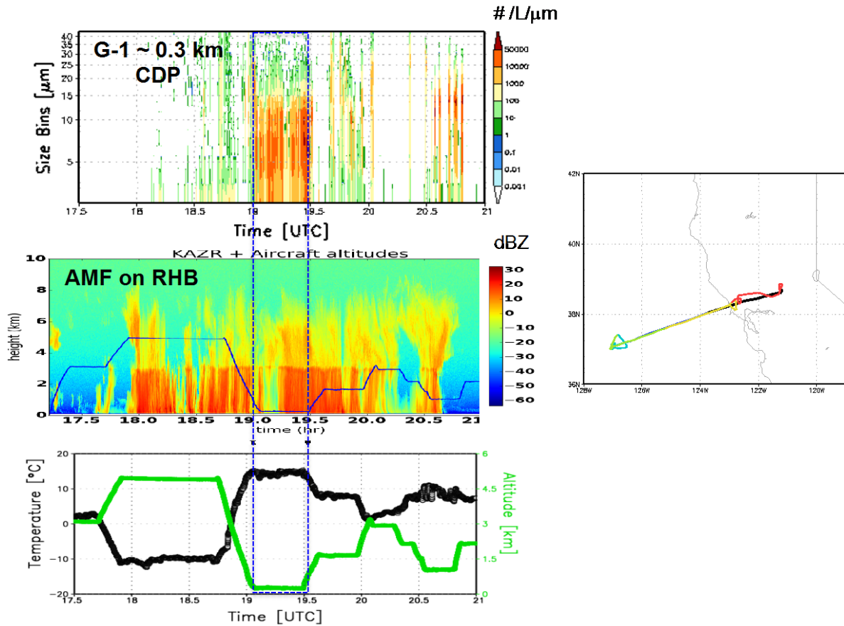
Figure 4. Data from G-1 and AMF2 during the rendezvous on 5 February, 2015. Top left: Cloud drop size distribution in \#/L/\mu m from CDP on G-1 at an altitude of about 0.3 km above Ron Brown . Middle left: KAZR cloud radar reflectivity in dBZ on AMF2 located on Ron Brown . Bottom left: Altitude (green) (in km) and temperature (in ^{\circ}C ) along the G-1 flight path. Right: the G-1 flight path for the coordinated flight, with a triangular path above Ron Brown .
