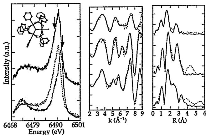
Figure 2. Left: K β emission spectra of Mn 3 O(O 2 CC 6 H 5 ) 6 (py) 2 (H 2 O) (top, structure in inset), Mn(OAc) 3 ·2H 2 O (bottom, —) and MnF 2 (bottom, ---). Middle: Preliminary EXAFS spectra of Mn 3 O(O 2 CC 6 H 5 ) 6 (py) 2 (H 2 O): transmission (top), site-selective K β fluorescence spectrum recorded with monitoring at 6492.6 eV (middle) and at 6488.9 eV (bottom). Right: Fourier transforms of EXAFS spectra in middle figure.
