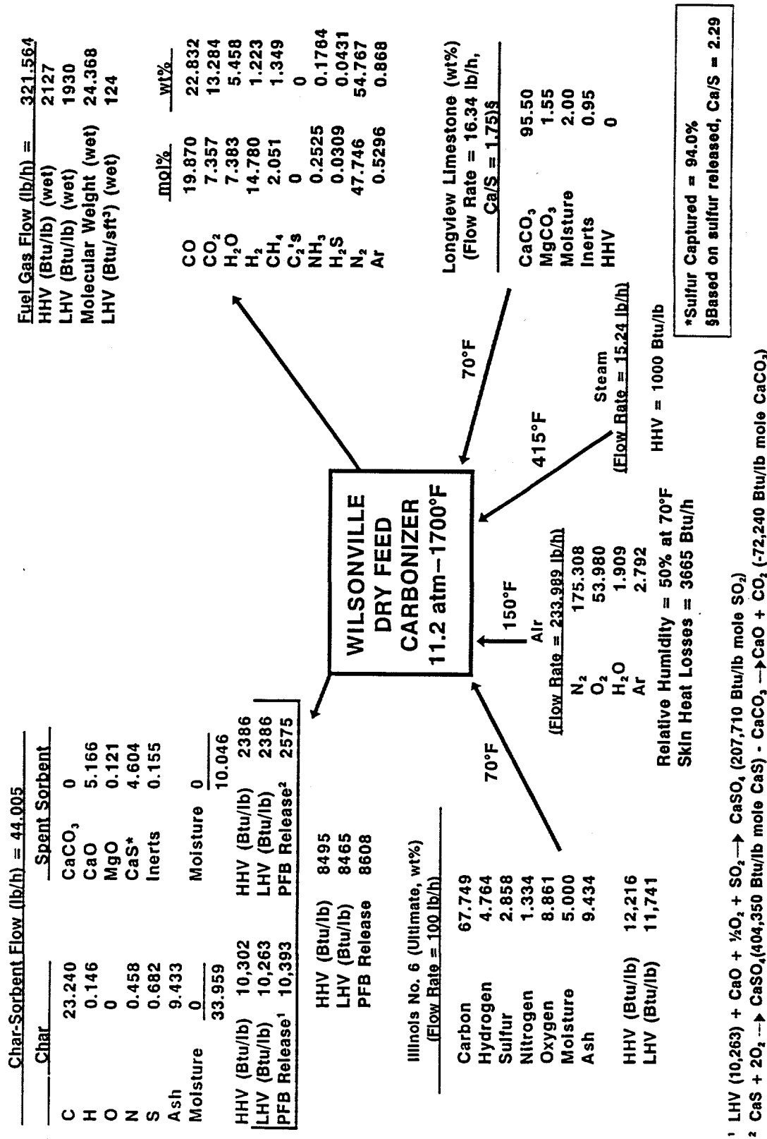
Figure 7. Wilsonville 1700°F Carbonizer Performance with Illinois No. 6 Coal
