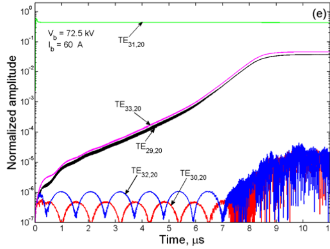
Fig. 1. Gyrotron operation in the TE_{31,20} -mode is accompanied by excitation of sidebands. The amplitude of distant sidebands (with radial indices 29 and 33) is much higher than the amplitudes of close sidebands with the radial indices 30 and 32.
