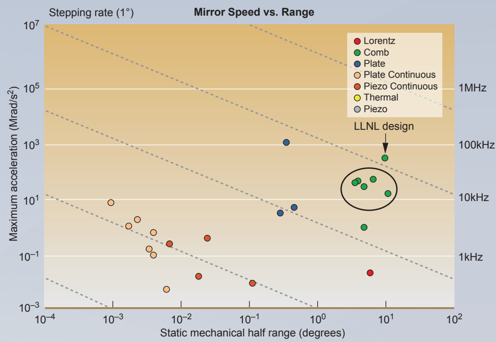
Figure 3: Existing mirrors that can be arrayed, possess at least tip and tilt degrees of freedom, and a fill-factor greater than 75%.
