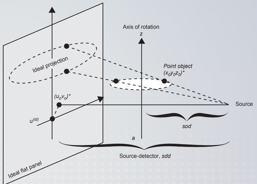
Figure 1. The experimental setup for the perfectly aligned x-ray computed tomography system assumed by CT reconstruction algorithms. The central ray extends from the source and intersects the rotation axis at right angles. If the panel is not perpendicular to the central ray, then the measured projection of a point will differ from the expected, which degrades the reconstruction resolution and contrast.
