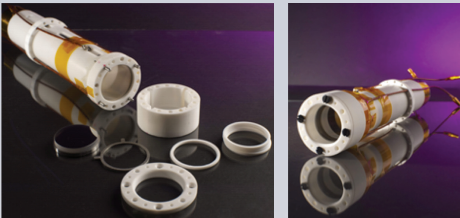
Figure 1. (left) Exploded view and (right) assembled laser photocathode and electron optics system.
