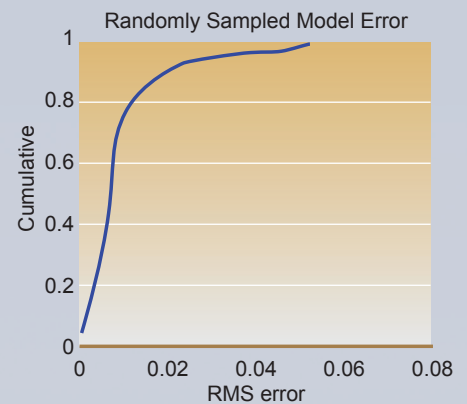
Figure 3. (top) The 3D parameter space has been partitioned into subregions. Each subregion has its own radial basis function expansion. (bottom) This figure shows the cumulative distribution error of the reduced-order model.
