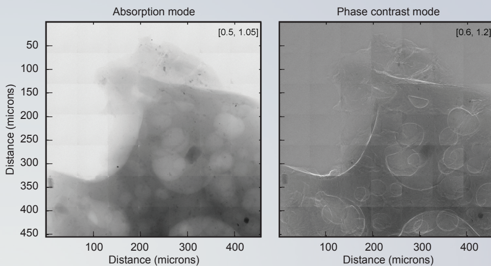
Figure 3. Digital radiographs of an extruded polymer foam containing bubbles of gas and/or air. The absorption-mode image on the left provides a relative measure of x-ray beam attenuation, thus indicating the amount of and/or density of material as a function of position, and the phase-contrast mode image on the right highlights changes in x-ray beam phase, thus enhancing the surfaces and edges in the foam.
