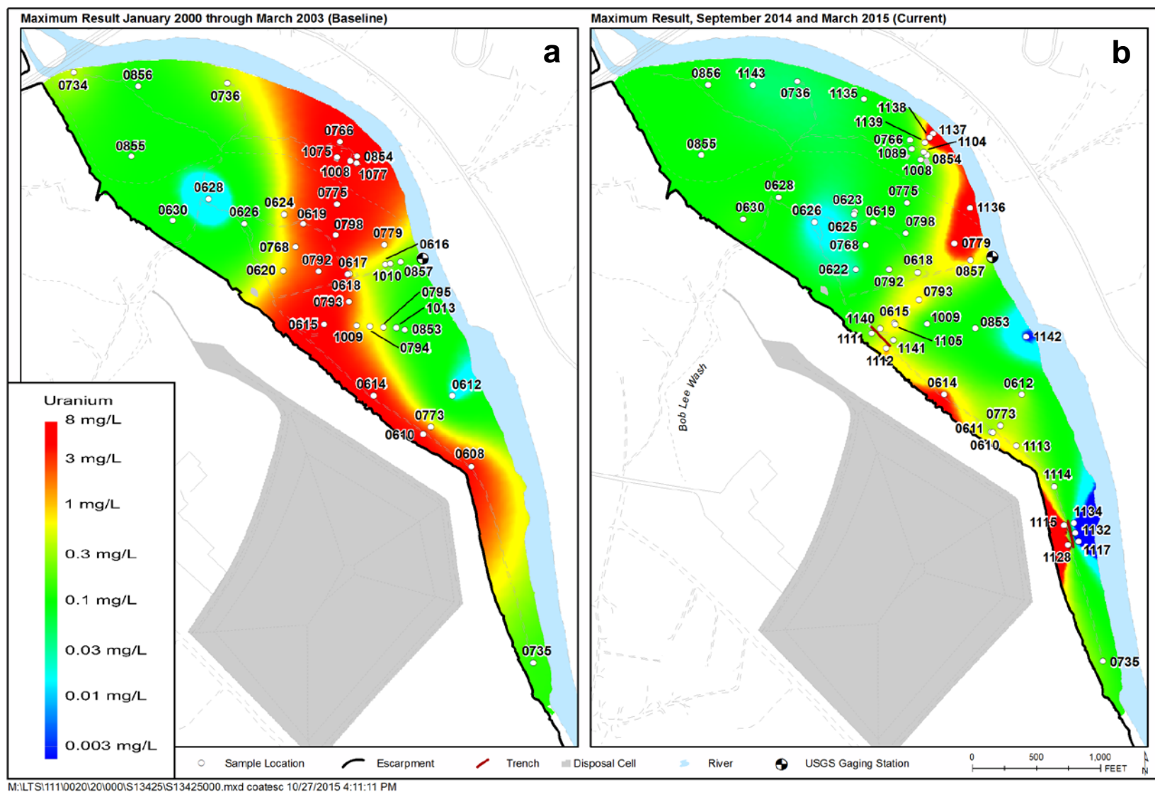
Fig. 3. Color Flood Plot of Maximum Uranium Concentrations in the Floodplain Aquifer in (a) Preremediation Years and (b) 2014–2015.
