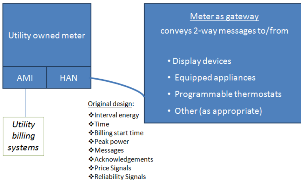
Figure 3. The Original HAN architecture with the Smart Meter as gateway
