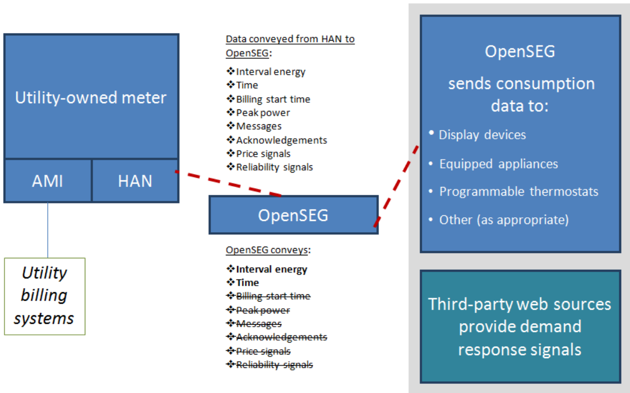
Figure 5. OpenSEG conveys electric consumption data
