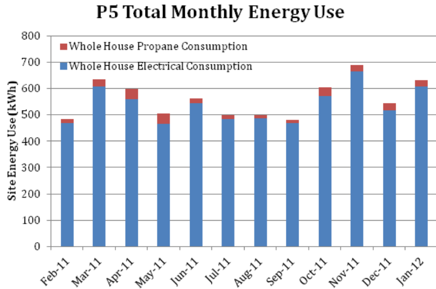
Figure 19 Summary of monthly post-retrofit energy use in P5 DER. Very little response to varying weather was observed in this super insulated, airtight retrofit.
