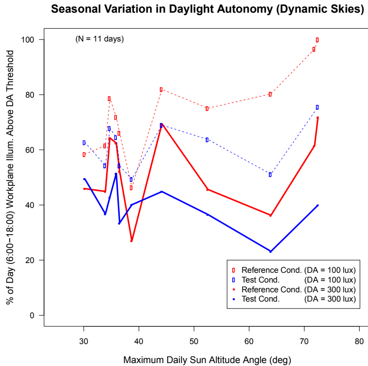
Fig. 8. Seasonal performance comparison based on daylight autonomy (DA) between the OLS (blue) and the reference Venetian blind (red) under dynamic sky conditions (6:00-18:00 ST).
