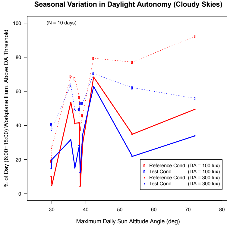
Fig. 7. Seasonal performance comparison based on daylight autonomy (DA) between the OLS (blue) and the reference Venetian blind (red) under cloudy conditions (6:00-18:00 ST).
