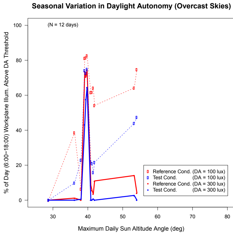
Fig. 9. Seasonal performance comparison based on daylight autonomy (DA) between the OLS (blue) and the reference Venetian blind (red) under overcast sky conditions (6:00-18:00 ST).
