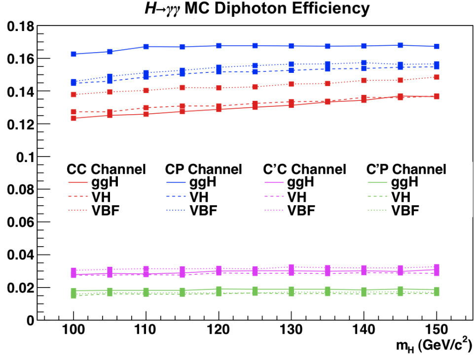
Figure 8.8: Diphoton efficiency for H \rightarrow \gamma\gamma MC signal events ( \epsilon_{\gamma\gamma}^{\text{MC}} ) as defined in the text, for each category and Higgs boson mass hypothesis. Values are calculated from the MC simulation for each production mechanism separately.
