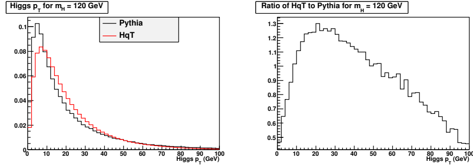
Figure C.1: Left: The Higgs boson p_T spectrum from HqT compared to that from PYTHIA, for a mass of 120 GeV/ c^2 . The integral of each histogram is normalized to 1.0. Right: The ratio of the two histograms on the left; the spectrum from HqT is divided by the spectrum from PYTHIA.
