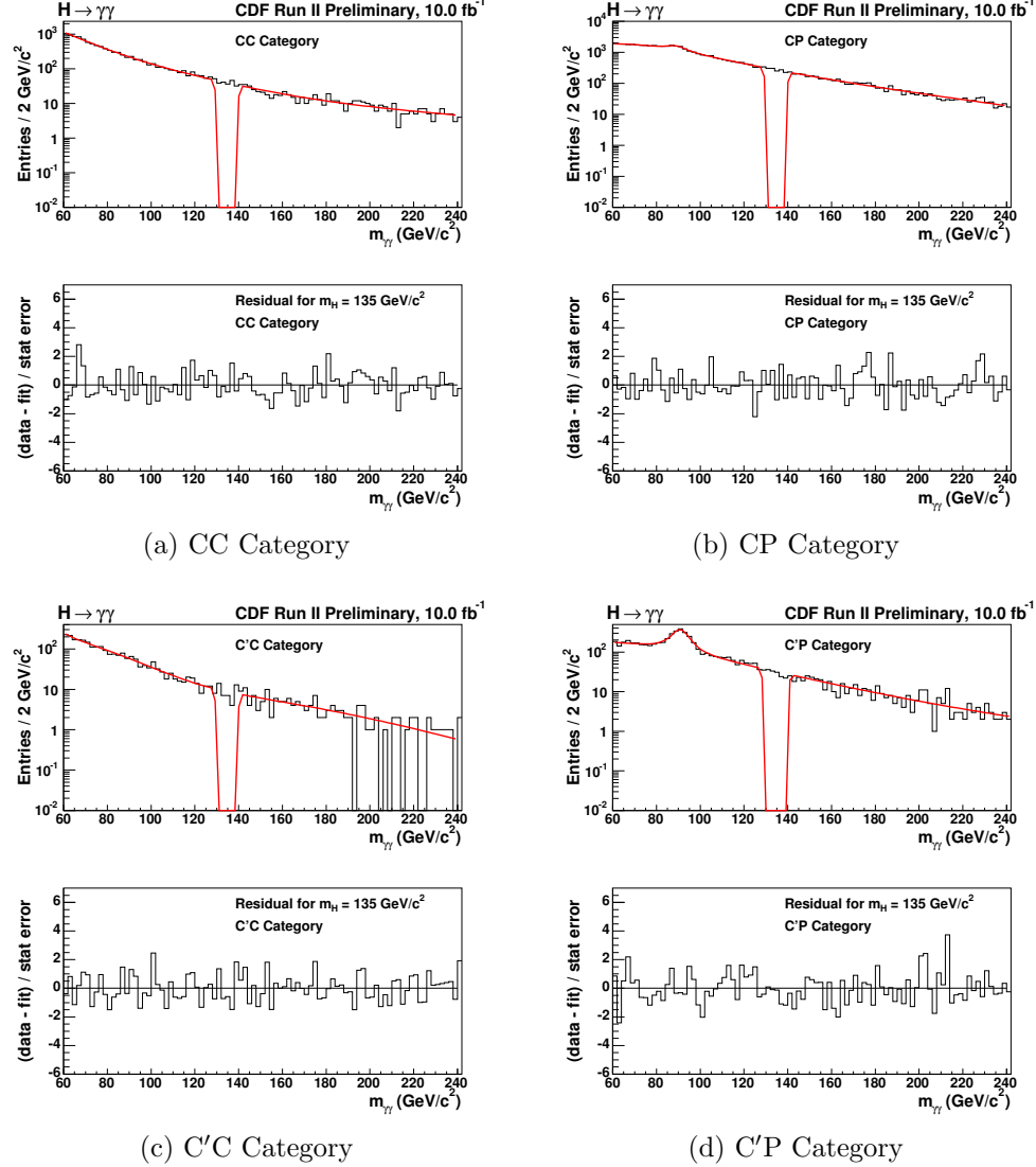
Figure D.8: Each subfigure shows a fit (red line) made to the sideband region of the data for each diphoton category using Equation (7.1) for the CC and C'C categories and the sum of Equations (7.1) and (7.2) for the CP and C'P categories. The two vertical red lines in each figure indicate the signal window excluded from the fit, here for a Higgs boson mass of 135 \text{ GeV}/c^2 . The bottom plot in each subfigure is obtained from first interpolating the fit into the signal region in order to obtain the background prediction in the signal region. The residual shown is then the resulting data yield minus the background yield, divided by the statistical error from the background yield.
