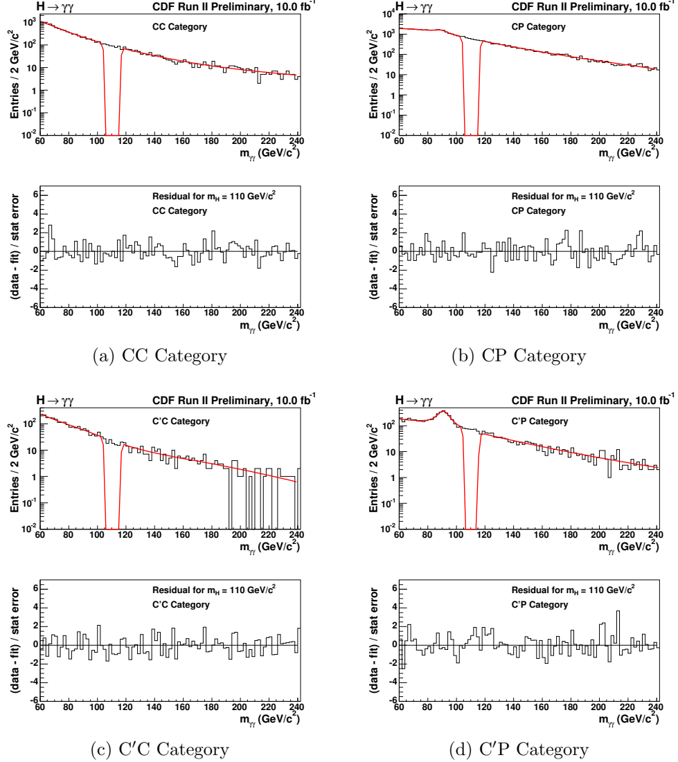
Figure D.3: Each subfigure shows a fit (red line) made to the sideband region of the data for each diphoton category using Equation (7.1) for the CC and C'C categories and the sum of Equations (7.1) and (7.2) for the CP and C'P categories. The two vertical red lines in each figure indicate the signal window excluded from the fit, here for a Higgs boson mass of 110 \text{ GeV}/c^2 . The bottom plot in each subfigure is obtained from first interpolating the fit into the signal region in order to obtain the background prediction in the signal region. The residual shown is then the resulting data yield minus the background yield, divided by the statistical error from the background yield.
