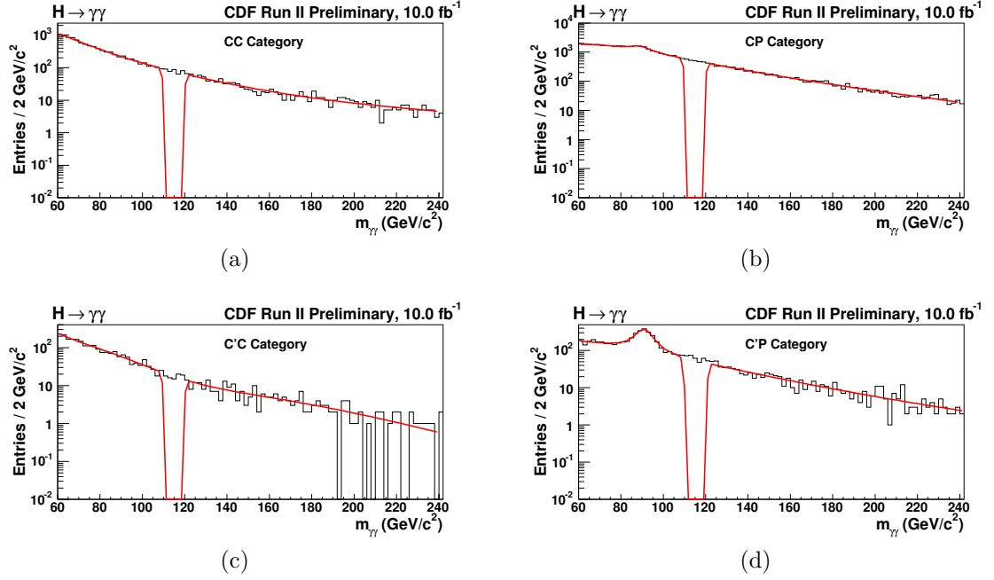
Figure 7.8: Each figure shows a fit (red line) made to the sideband region of the data for each diphoton category using f_s(m) for the CC and C'C categories and the sum of f_Z(m) and f_s(m) for the CP and C'P categories. The two vertical lines in each figure indicate the signal window excluded from the fit, here for a Higgs boson mass of 115 GeV/c 2 .
