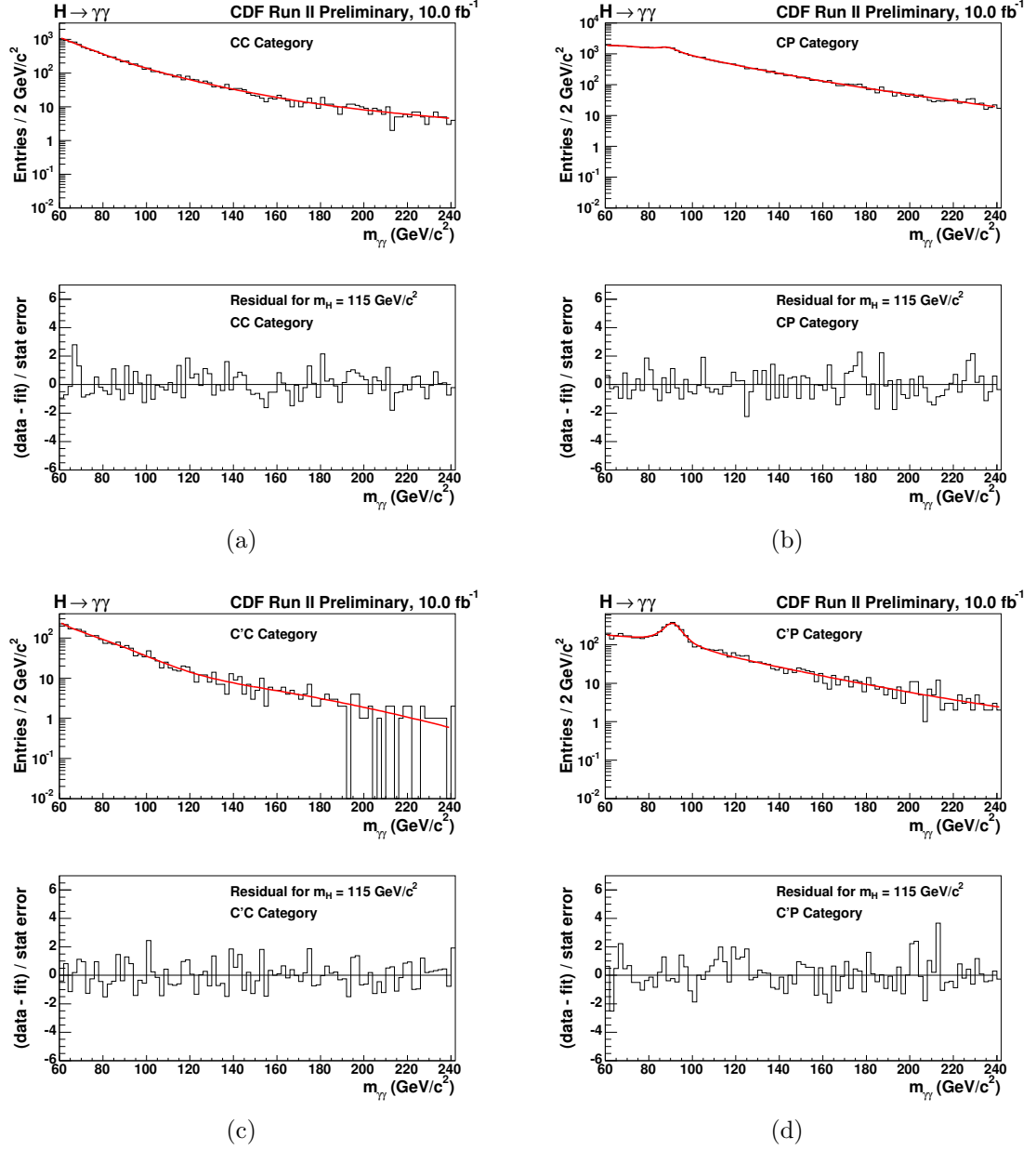
Figure 7.9: The upper plot in each subfigure shows the sideband fit from Figure 7.8 interpolated into the 115 GeV/c 2 signal region, for each diphoton category. The residual in the lower plot of each subfigure shows the data yield minus the background yield, divided by the statistical error from the background yield.
