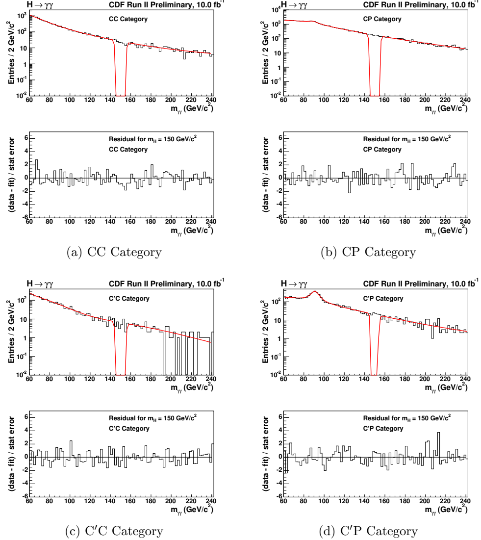
Figure D.11: Each subfigure shows a fit (red line) made to the sideband region of the data for each diphoton category using Equation (7.1) for the CC and C'C categories and the sum of Equations (7.1) and (7.2) for the CP and C'P categories. The two vertical red lines in each figure indicate the signal window excluded from the fit, here for a Higgs boson mass of 150 \text{ GeV}/c^2 . The bottom plot in each subfigure is obtained from first interpolating the fit into the signal region in order to obtain the background prediction in the signal region. The residual shown is then the resulting data yield minus the background yield, divided by the statistical error from the background yield.
