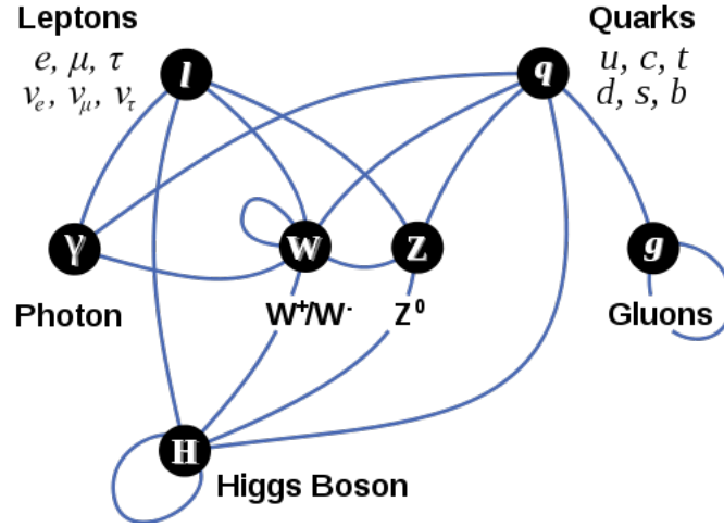
Figure 1.2: A diagram showing the ways in which the elementary particles interact with one another, including interactions with the Higgs field [5]. The Higgs boson is the only particle predicted by the SM that has not yet been observed in nature.
