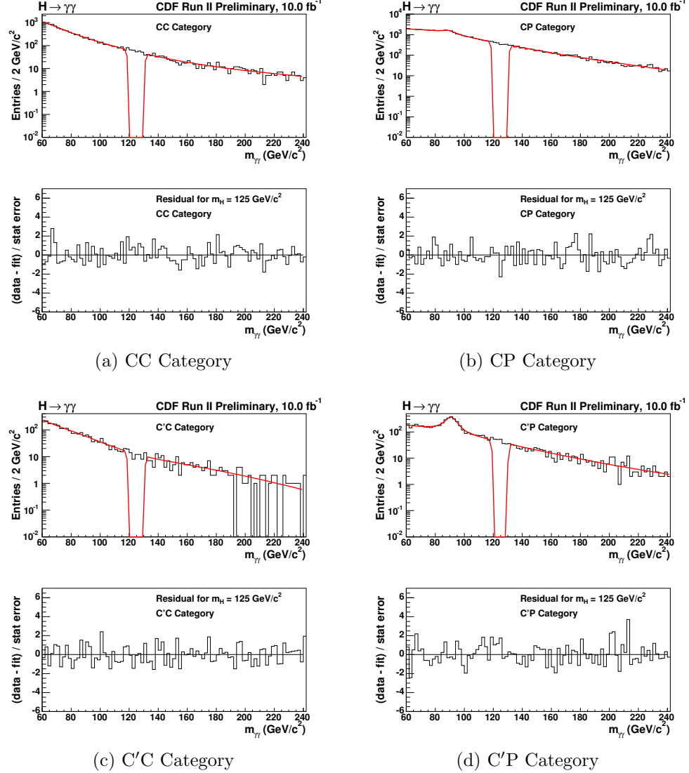
Figure D.6: Each subfigure shows a fit (red line) made to the sideband region of the data for each diphoton category using Equation (7.1) for the CC and C'C categories and the sum of Equations (7.1) and (7.2) for the CP and C'P categories. The two vertical red lines in each figure indicate the signal window excluded from the fit, here for a Higgs boson mass of 125 \text{ GeV}/c^2 . The bottom plot in each subfigure is obtained from first interpolating the fit into the signal region in order to obtain the background prediction in the signal region. The residual shown is then the resulting data yield minus the background yield, divided by the statistical error from the background yield.
