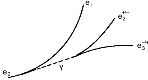
Figure 5.19: Illustration of a trident.
