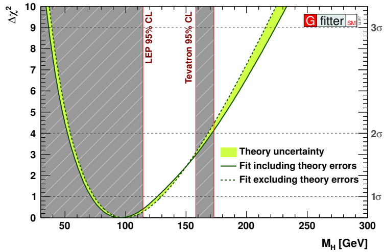
Figure 1.8: An indirect constraint on the Higgs boson mass is obtained from a global electroweak fit performed by the Gfitter collaboration. From July of 2011, the Gfitter collaboration uses a \Delta\chi^2 statistic to fit electroweak parameters of the SM theory to the corresponding measured values [29]. The preferred value of the Higgs boson mass from this indirect electroweak measurement is the mass for which the \Delta\chi^2 is minimized ( 96 \text{ GeV}/c^2 ). With 95% confidence level (see the 2\sigma horizontal line), this plot demonstrates that if the Higgs boson exists, the SM theory prefers its mass to be below about m_H < 169 \text{ GeV}/c^2 . See Reference [30] for a preliminary updated plot using results from more recent direct searches and electroweak measurements.
