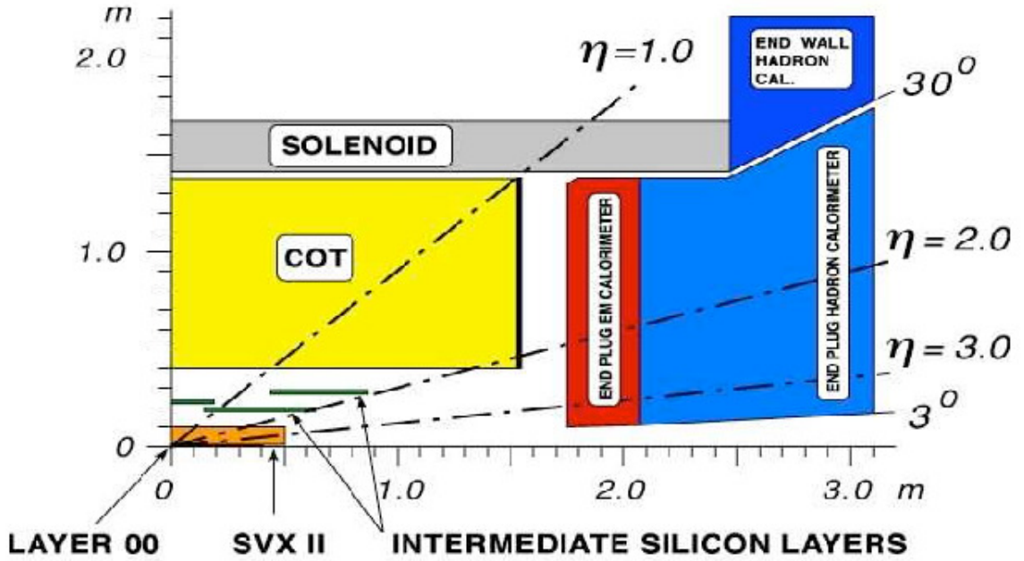
Figure 3.4: An r-z view of one quadrant of the detector showing the CDF tracking coverage [40]. The COT detector provides a coverage of |\eta| < 1.0 and the silicon detector provides a coverage of |\eta| < 2.0 .
