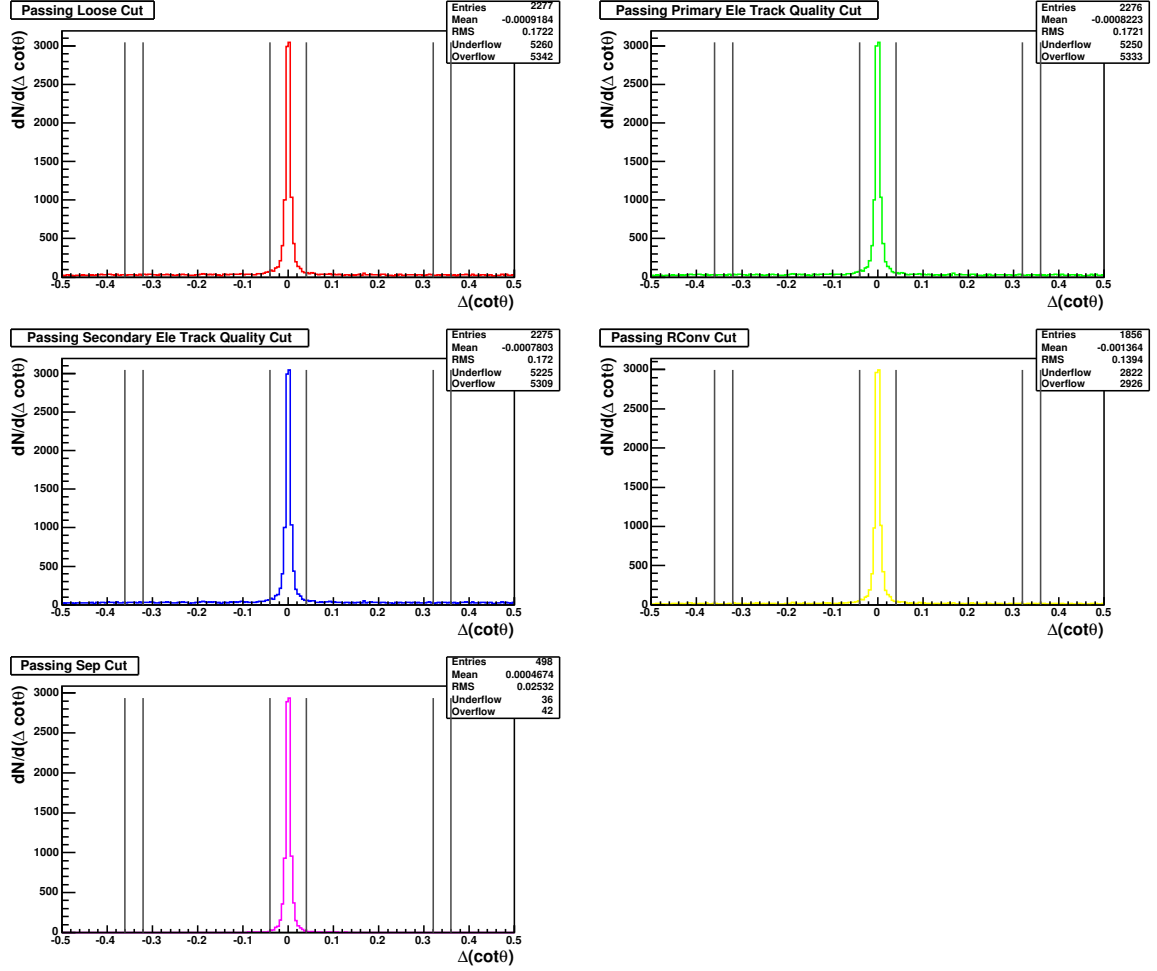
Figure 5.22: The \Delta \cot \theta distribution for conversions in the Z \rightarrow e + \text{trident} MC simulation for each cut tested in Method A (see Table 5.3). Grey vertical lines show where the central and sideband windows are located. The central window is -0.04 < \Delta \cot \theta < 0.04 ; the left and right sideband windows are -0.36 < \Delta \cot \theta < -0.32 and +0.32 < \Delta \cot \theta < +0.36 , respectively.
