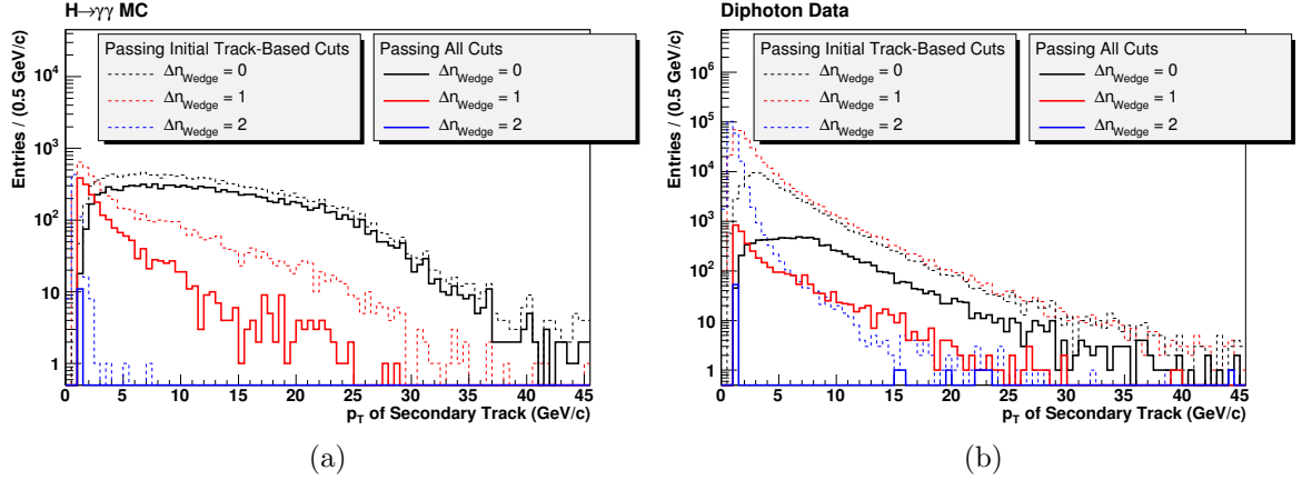
Figure 5.8: The p_T distribution of the second track of a conversion for different wedge separation numbers. This is shown for (a) H \rightarrow \gamma\gamma conversions and (b) conversions reconstructed in the data described in Chapter 6. Conversions from H \rightarrow \gamma\gamma events are of higher p_T than those from backgrounds in the data. The second track is, therefore, expected to have higher than average p_T than backgrounds in the data.
