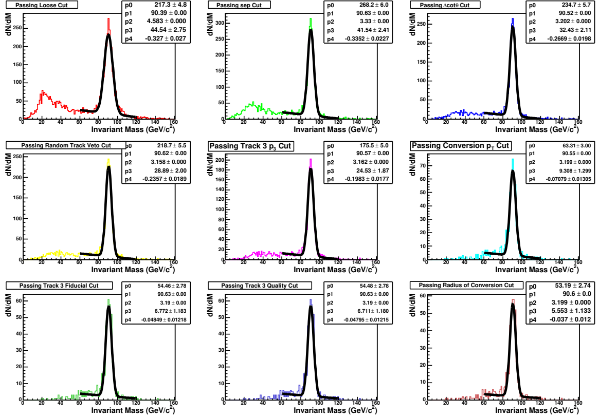
Figure 5.25: The invariant mass distribution of Z \rightarrow e + \text{trident} events in the MC simulation. The upper left distribution includes only the loose cuts of Table 5.6, which are cuts applied to the same-sign pair of the trident. For the remaining distributions, consecutively tighter cuts on the conversion have been applied. These are the cuts given in Table 5.7. Each histogram is fit to the sum of a Gaussian function and a polynomial function. The number of signal events is obtained from the integral in the range 83.0 < m_{ee} < 99.0 \text{ GeV}/c^2 , with the background subtracted from sideband regions 61.0 < m_{ee} < 69 \text{ GeV}/c^2 and 113.0 < m_{ee} < 121 \text{ GeV}/c^2 .
