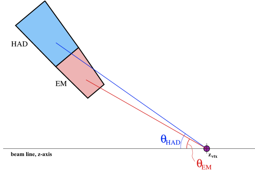
Figure 3.17: The E_T measurement for an EM cluster is calculated from E_T = E \sin \theta with the EM polar angle obtained relative to the primary vertex location [40]. For trigger towers, the primary vertex is assumed to have z_{\text{vtx}} = 0 . During offline EM calorimeter clustering, this also true, but once an EM cluster is obtained, its E_T is calculated using the reconstructed primary vertex.
