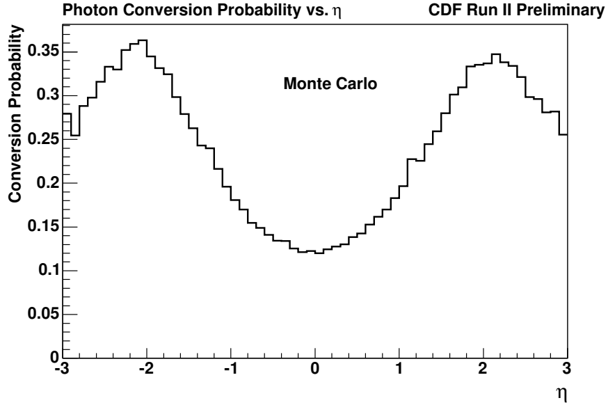
Figure 5.1: Photons from a H \rightarrow \gamma\gamma MC sample are used to study the conversion probability as a function of \eta . We use generator-level (“truth”) information from the simulated MC to select photons that convert. Using this truth information, the probability is obtained from the ratio of the \eta distribution for photons that convert to the \eta distribution for all generated photons.
