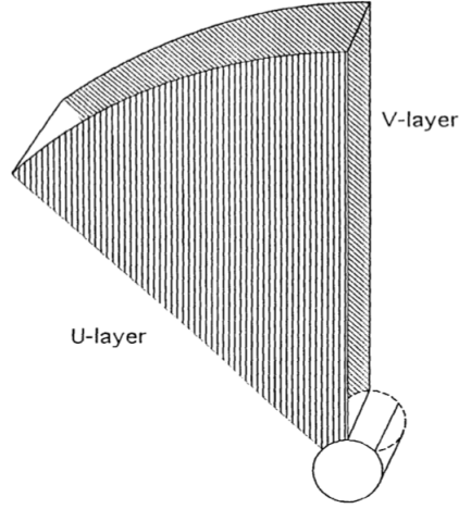
Figure 3.13: Diagram showing one 45^\circ sector of the PES detector, located 6 radiation lengths into the PEM [43]. The two scintillator layers are oriented 45^\circ to one another.
