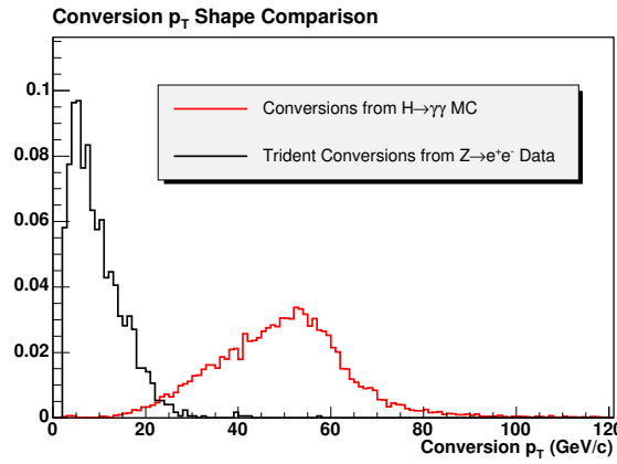
Figure 5.20: The conversion p_T distribution from H \rightarrow \gamma\gamma photons versus photons from tridents.
