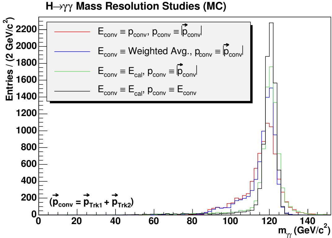
Figure 5.18: The Higgs boson mass for m_H = 120 \text{ GeV}/c^2 is shown, reconstructed from a central photon and a central conversion. Each histogram shows a different manner in which the conversion four-momentum was defined based on calorimeter and/or tracking measurements. The “Weighted Avg.” method refers to defining the conversion energy from an error-weighted average of the calorimeter energy and track momentum. The black histogram shows the method that provides the best resolution, which is discussed in the main text.
