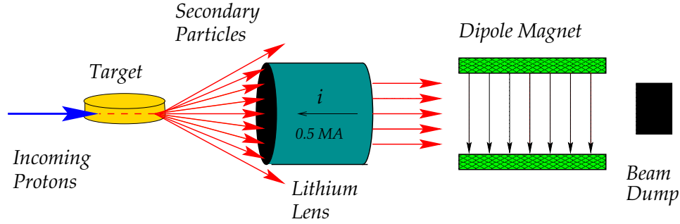
Figure 2.2: Mechanism for antiproton extraction [37]. Protons were sent to a fixed target, a lithium lens was used to reduce the spread of secondary particles, and a dipole magnet was used to separate antiprotons with 8 GeV of energy. These antiprotons were sent to the Debuncher (see text) and all other secondary particles were sent to an area for disposal (a beam dump).
