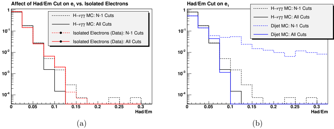
Figure 5.12: The dashed lines in both figures show the distribution after all other cuts have been applied except for the Had/Em cut ( N - 1 cuts). The solid lines show the distribution after this cut has been applied. For the H \rightarrow \gamma\gamma and dijet MC samples, the other cuts applied are those from this chapter. The isolated electrons come from Z \rightarrow e^+e^- decays and the other cuts applied are those described in Section 4.3.
