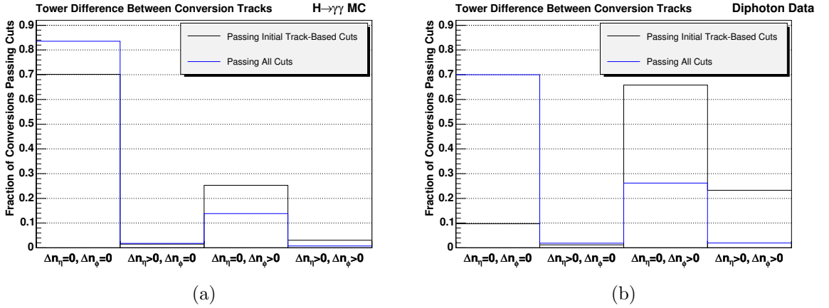
Figure 5.6: Different scenarios of \Delta n_\eta and \Delta n_\phi for (a) H \rightarrow \gamma\gamma conversions and (b) conversions reconstructed in the data described in Chapter 6. The \Delta n_\eta = 0 , \Delta n_\phi = 0 scenario are 1-tower conversions in which the two tracks point to the same tower. Essentially all conversions in the \Delta n_\eta > 0 , \Delta n_\phi = 0 scenario have \Delta n_\eta = 1 , which means that most of the shower energy from e_2 is generally included in the 1–3 tower EM cluster for the leading electron. These are considered 1-tower conversions. The \Delta n_\eta = 0 , \Delta n_\phi > 0 scenario are 2-tower conversions where the two tracks point to the same \eta tower, but different \phi wedges. The last scenario shows another type of 2-tower conversion. The fraction of conversions with tracks in different \phi towers reduces after the initial track-based selection due to additional cuts such as requiring a minimum p_T for the second track.
