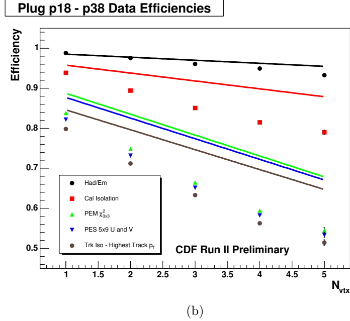
Figure 4.8: As a function of the number of vertices reconstructed in the event, cumulative plug photon ID efficiencies are plotted for each cut made in the order they are shown. Efficiencies from the data are represented by markers (solid shapes) and efficiencies from the MC prediction are represented by lines. The same set of MC efficiency lines are drawn for both data periods. See the text for details on the upper and lower plots.
