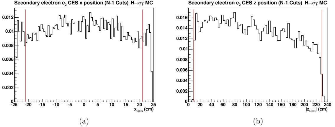
Figure 5.10: The local x and z position in the CES that the second track of a H \rightarrow \gamma\gamma conversion points to. All cuts made in the conversion selection have been applied, except for the cut on the variable shown ( N - 1 cuts). Red lines show where cuts are made.
