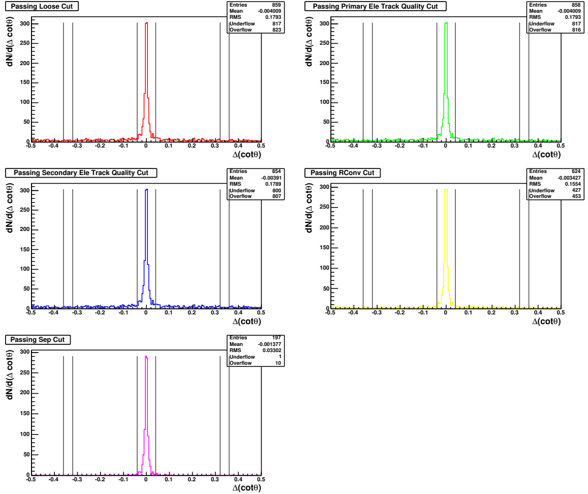
Figure 5.21: The \Delta \cot \theta distribution for conversions in the Z \rightarrow e + \text{trident} data for each cut tested in Method A (see Table 5.3). Grey vertical lines show where the central and sideband windows are located. The central window is -0.04 < \Delta \cot \theta < 0.04 ; the left and right sideband windows are -0.36 < \Delta \cot \theta < -0.32 and +0.32 < \Delta \cot \theta < +0.36 , respectively.
