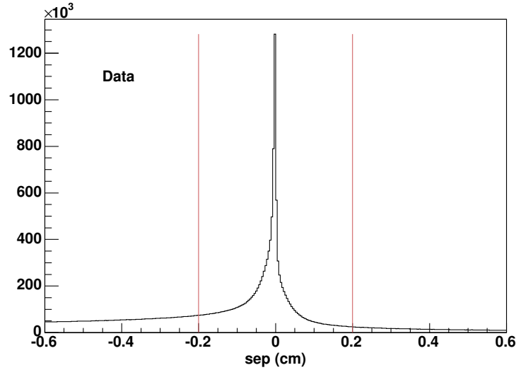
Figure 5.4: The sep distribution for electron candidate ( e_1 ) tracks and any other track in the event. True conversions populate the sep = 0 cm region. Red lines show where cuts are made. (The data sample is described in Chapter 6.)
