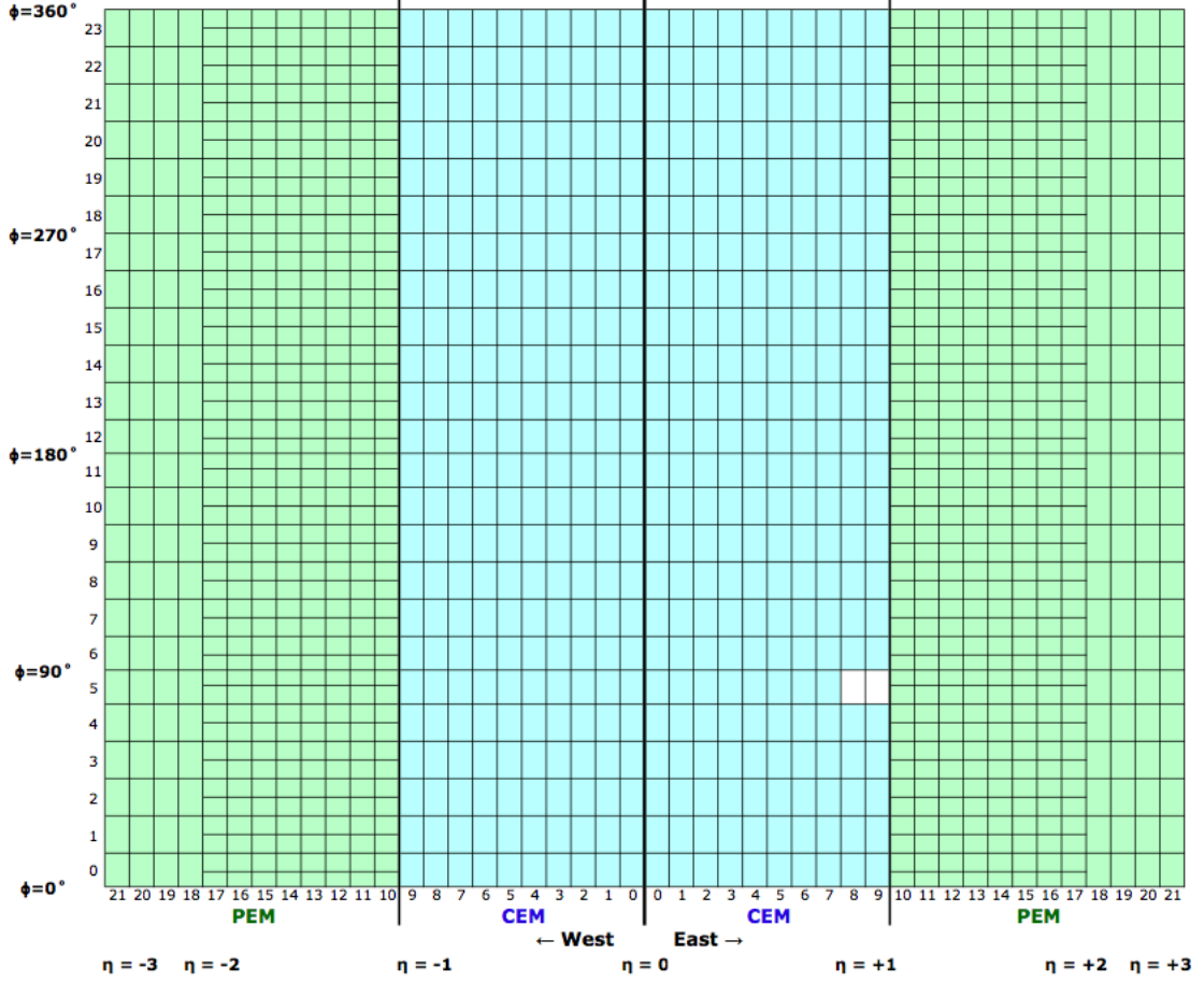
Figure 3.19: Calorimeter segmentation in \eta - \phi space for the central (blue) and plug (green) electromagnetic calorimeters, CEM and PEM, respectively. Calorimeter wedge numbers (0–23) are shown on the left vertical axis labels, each covering 15^\circ in \phi . For a portion of the plug region, each wedge contains two towers such that the tower \phi segmentation is 7.5^\circ . The x axis shows the west (left) and east (right) \eta tower numbers, from 0–21 as shown in Figure 3.8, with a coverage of 0 < |\eta| < 3.6 . The white box, called the chimney, is a region excluded from use in particle identification. It is a gap in the detector used for cables and cryogenic utilities needed for the solenoid.
