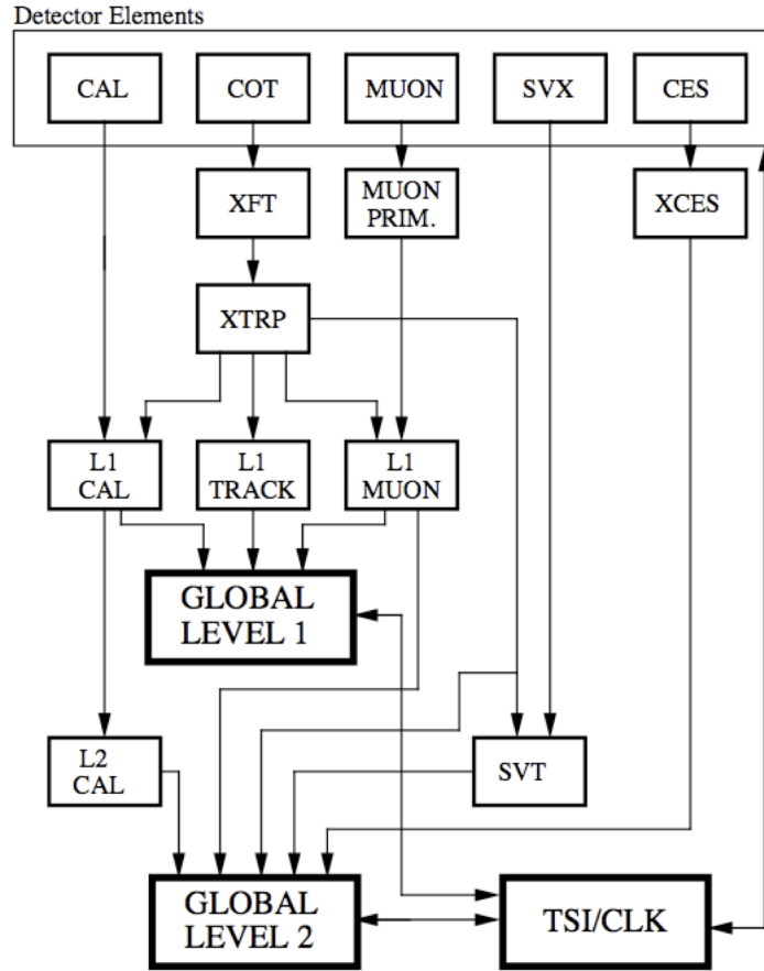
Figure 3.14: A block diagram showing detector inputs for the first two levels of the trigger system [43]. The third level of the trigger system uses all detector components.
