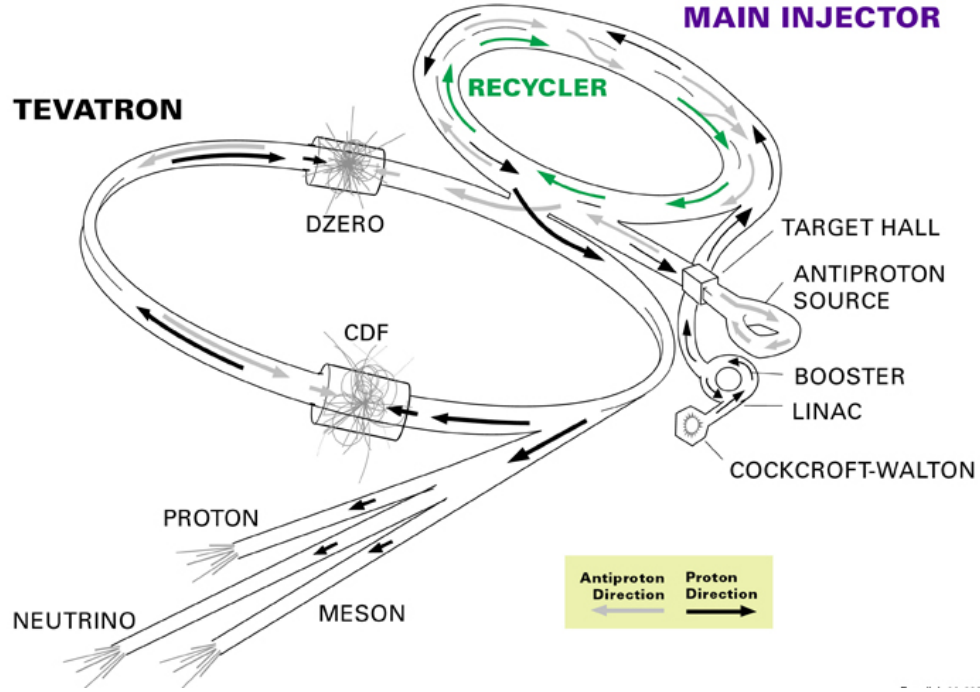
Figure 2.1: Fermilab's p\bar{p} accelerator chain [2, 37]. See the text for more detail.
