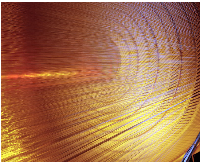
Figure 3.6: A picture of CDF's Run I Central Tracking Chamber (CTC), which sits in the museum area of the main CDF building (B0) [40]. The Run II COT design is very similar, but with a larger number of cells and a larger number of wires for stereo layers, allowing for a smaller maximum drift distance [42].
