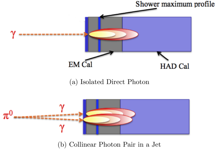
Figure 4.2: Illustration of the shower profile in the shower maximum detector for (a) a direct (prompt) photon and (b) collinear pairs of photons from the decay of a neutral meson [40].
