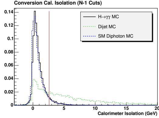
Figure 5.15: The calorimeter isolation distribution for conversions reconstructed in H \rightarrow \gamma\gamma , dijet, and QCD diphoton MC samples. The red line shows where a cut is made on this variable.
