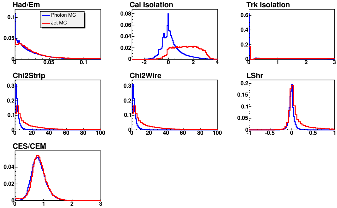
Figure 4.3: Distributions of variables used as inputs to the NN, shown for photon and jet MC samples. Each distribution is normalized to unit area.
