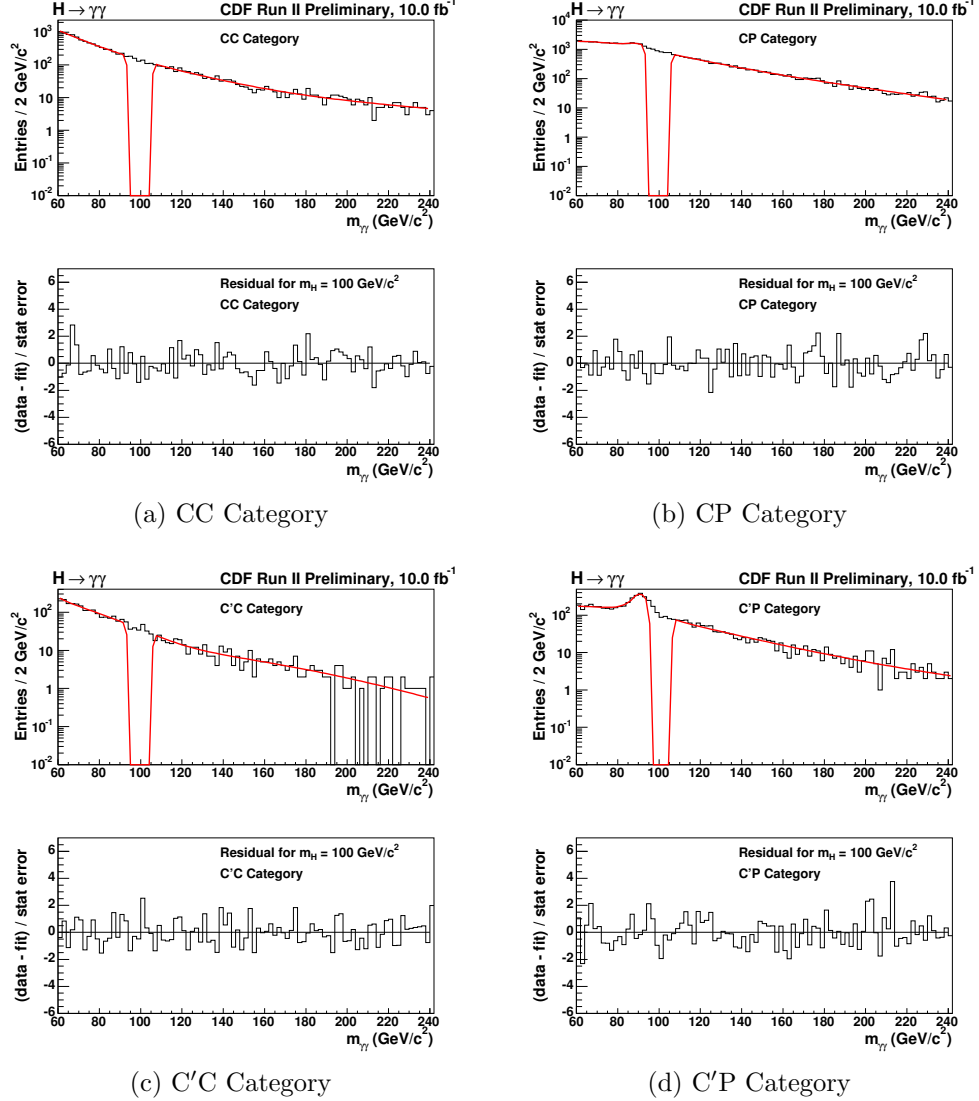
Figure D.1: Each subfigure shows a fit (red line) made to the sideband region of the data for each diphoton category using Equation (7.1) for the CC and C'C categories and the sum of Equations (7.1) and (7.2) for the CP and C'P categories. The two vertical red lines in each figure indicate the signal window excluded from the fit, here for a Higgs boson mass of 100 \text{ GeV}/c^2 . The bottom plot in each subfigure is obtained from first interpolating the fit into the signal region in order to obtain the background prediction in the signal region. The residual shown is then the resulting data yield minus the background yield, divided by the statistical error from the background yield.
