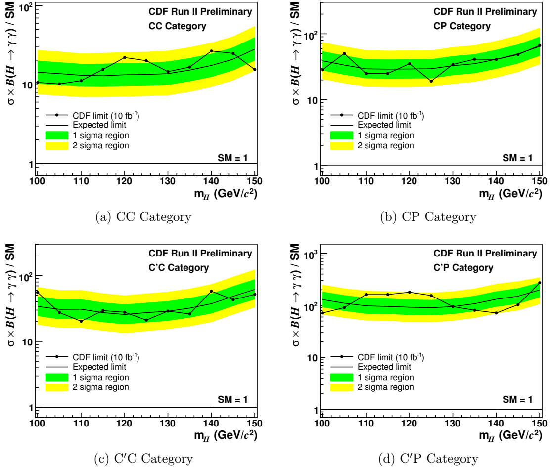
Figure 11.3: 95% C.L. upper limits on the production cross section multiplied by the H \rightarrow \gamma\gamma branching ratio, relative to the SM prediction, calculated for each diphoton category alone.
