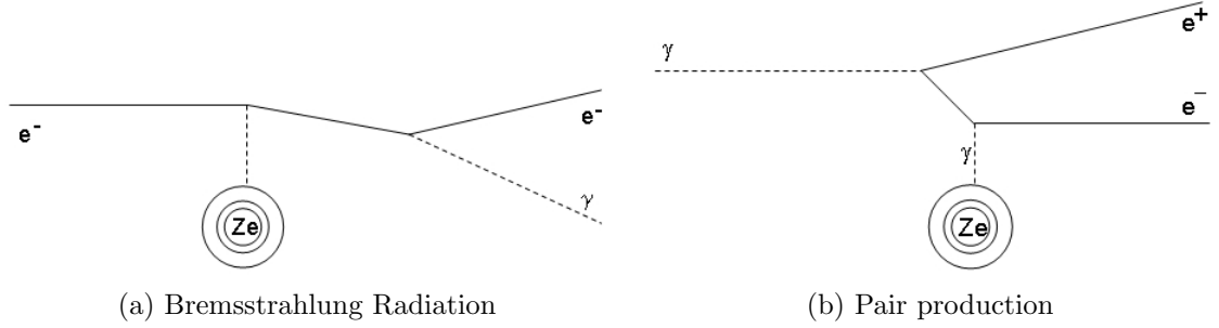
Figure 3.11: (a) The interaction process for an electron in the presence of absorber material. (b) An example interaction process for a photon in the presence of absorber material.
