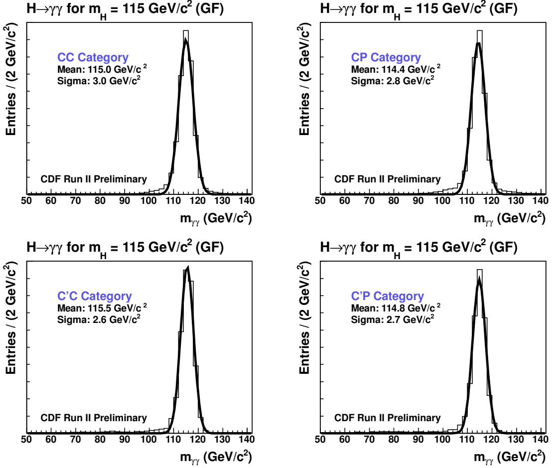
Figure 8.5: The m_{\gamma\gamma} distributions for GF events in each diphoton category along with Gaussian fits made to these distributions. The shapes are obtained from the PYTHIA MC prediction and reweighted to the N_{\text{vtx}} distribution of the data.
