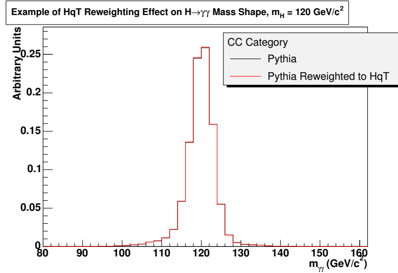
Figure C.2: Effect of HqT reweighting on the m_{\gamma\gamma} shape (GF signal events). An example is shown for a mass of 120 GeV/ c^2 in the CC category.
