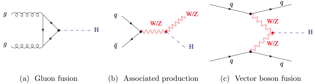
Figure 1.4: The dominant production mechanisms at the Tevatron for the SM Higgs boson [3, 23, 24]. We search for a Higgs boson originating from any of these three processes.
