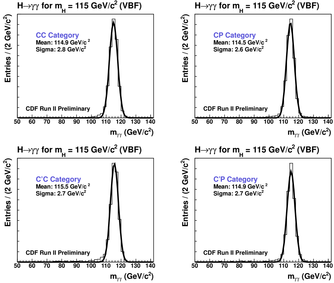
Figure 8.7: The m_{\gamma\gamma} distributions for VBF events in each diphoton category along with Gaussian fits made to these distributions. The shapes are obtained from the PYTHIA MC prediction and reweighted to the N_{\text{vtx}} distribution of the data.
