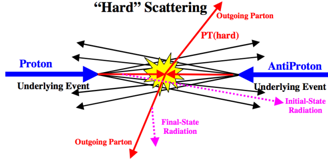
Figure 8.1: A schematic [76] of a hard scattering interaction between a pair of partons from the proton and antiproton, indicated by the red lines pointing towards one another; the resulting high p_T (hard) particles produced by the collision have red lines pointing outward away from the collision vertex. As an example, ISR is shown coming from the parton in the proton and FSR is shown coming from one of the outgoing particles. All other objects shown are the soft p\bar{p} (beam) remnants, which are considered the underlying event.
