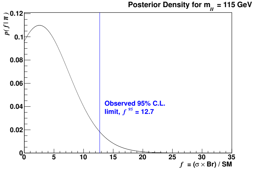
Figure 11.1: The posterior density for f = \sigma \times B(H \rightarrow \gamma\gamma)/\text{SM} shows the observed limit set by the data of 12.7 times the SM prediction for a Higgs mass hypothesis of 115 GeV/c 2 . This limit is indicated by the blue line, where 95% of the density is below this limit. This posterior density was obtained using all four diphoton categories.
