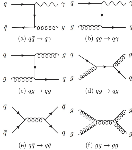
Figure 7.3: The main diagrams for \gamma +jet production (first row) and dijet production (second and third rows) at the Tevatron, which can be misreconstructed as diphoton events in the data [28].
