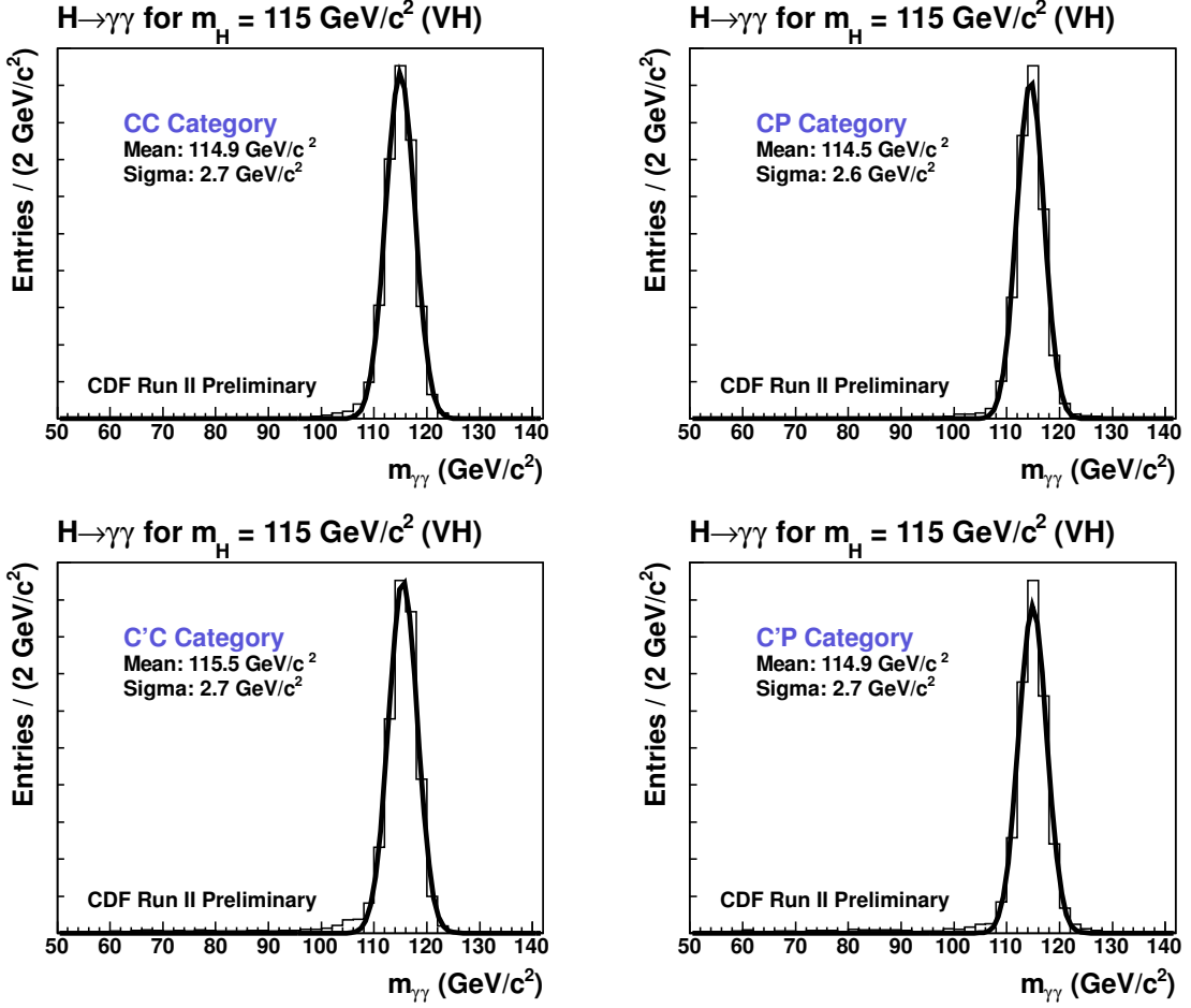
Figure 8.6: The m_{\gamma\gamma} distributions for VH events in each diphoton category along with Gaussian fits made to these distributions. The shapes are obtained from the PYTHIA MC prediction and reweighted to the N_{\text{vtx}} distribution of the data.
