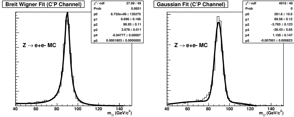
Figure 7.7: MC simulation of Z \rightarrow e^+e^- events that pass the diphoton selection for the C'P category. The left and right plots show the m_{\gamma\gamma} distribution fit to a Breit-Wigner and Gaussian function, respectively. The former better describes the shape and is used when fitting to the Z contribution in the data. In the left plot, the parameters p_0 – p_2 correspond to those described in Equation (7.2).
