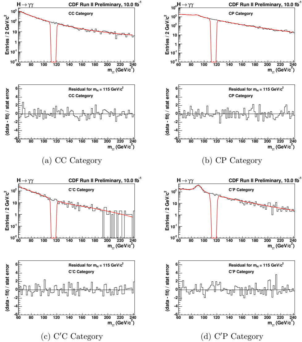
Figure D.4: Each subfigure shows a fit (red line) made to the sideband region of the data for each diphoton category using Equation (7.1) for the CC and C'C categories and the sum of Equations (7.1) and (7.2) for the CP and C'P categories. The two vertical red lines in each figure indicate the signal window excluded from the fit, here for a Higgs boson mass of 115 \text{ GeV}/c^2 . The bottom plot in each subfigure is obtained from first interpolating the fit into the signal region in order to obtain the background prediction in the signal region. The residual shown is then the resulting data yield minus the background yield, divided by the statistical error from the background yield.
