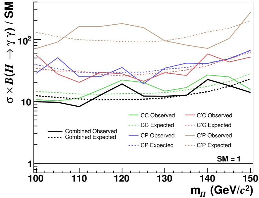
Figure 11.5: 95% C.L. upper limits on the production cross section multiplied by the H \rightarrow \gamma\gamma branching ratio, relative to the SM prediction. Observed and expected limits are shown for each category calculated alone and for the combined limit using all four categories.
