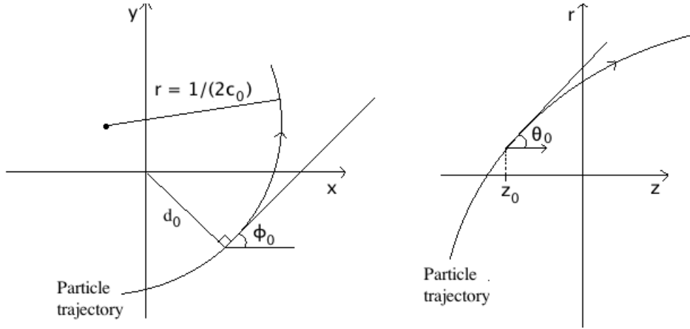
Figure 3.15: Diagram showing r - \phi (left) and r - z (right) track parameters.
