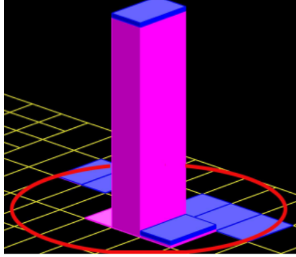
Figure 3.18: “Lego” plot of an EM shower in the calorimeter. The yellow grid shows the \eta - \phi segmentation, so each rectangular region represents a calorimeter tower [40]. Pink represents the amount of EM E_T and blue represents the amount of HAD E_T . The tower blocks provide an example of an EM shower in the central calorimeters. The energy of an EM shower is generally contained within a few towers. Only a small amount of this energy leaks into the hadron towers. The red circle indicates a region in \eta - \phi space defined by \Delta R = \sqrt{\Delta\phi^2 + \Delta\eta^2} .
