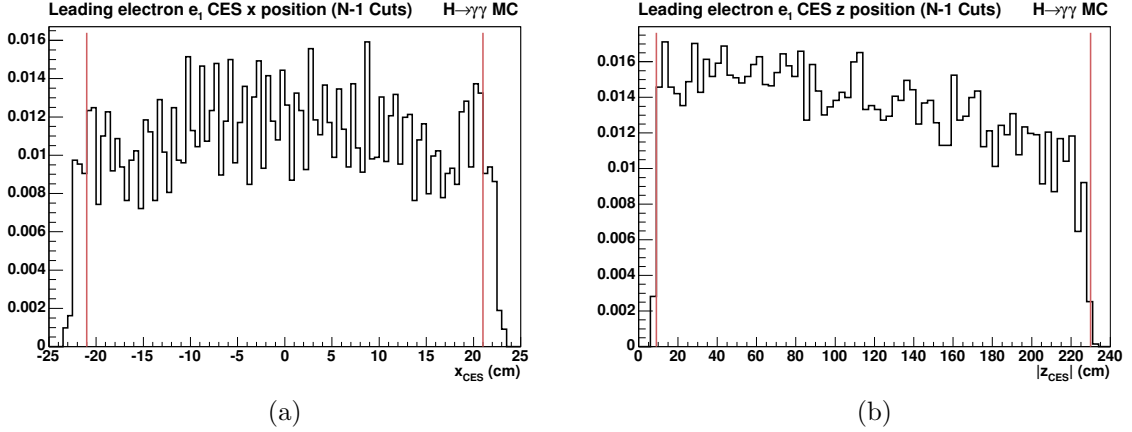
Figure 5.9: The local x and z position of the electron candidate’s EM cluster in the CES for conversions from a H \rightarrow \gamma\gamma MC simulation. All cuts made in the conversion selection have been applied, except for the cut on the variable shown (“ N - 1 cuts”). Red lines show where cuts are made.
