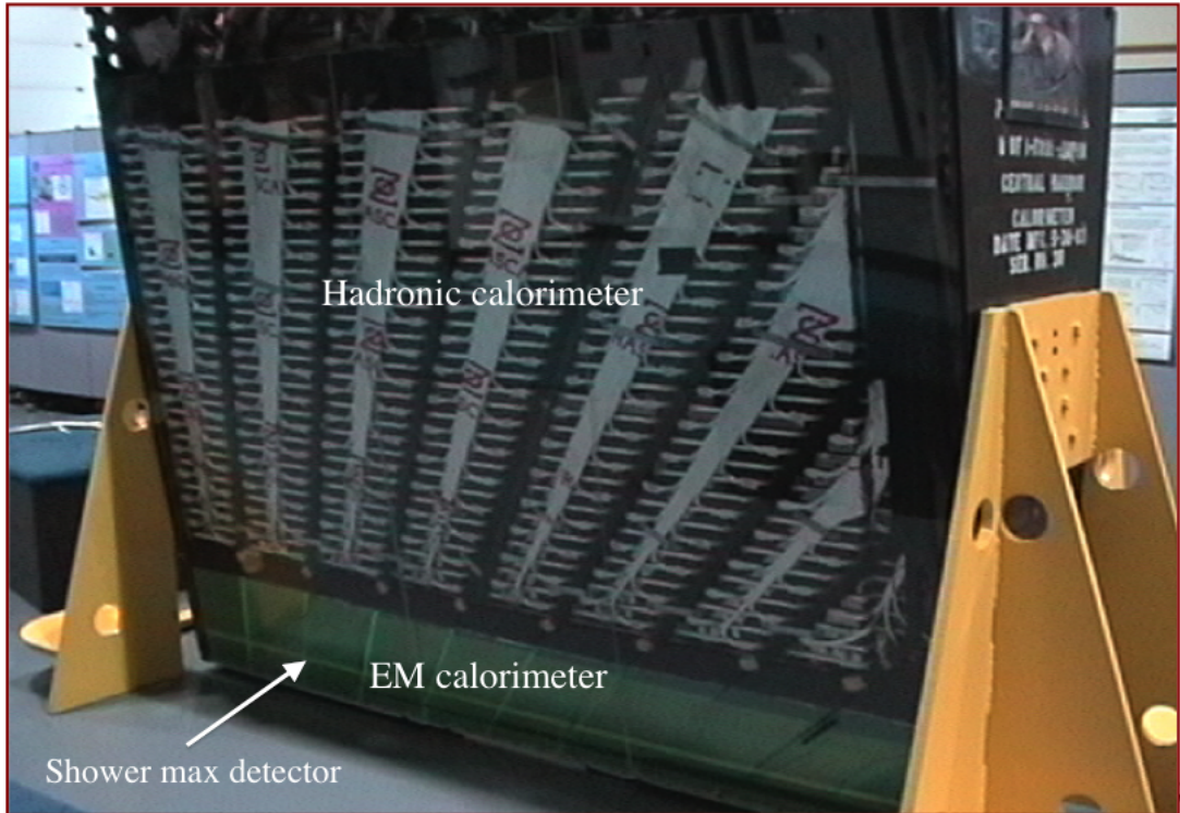
Figure 3.9: An example of a central calorimeter wedge [40]. The lower (upper) region is a portion of the EM (HAD) calorimeter. The shower maximum detector is located six radiation lengths into the EM calorimeter.
