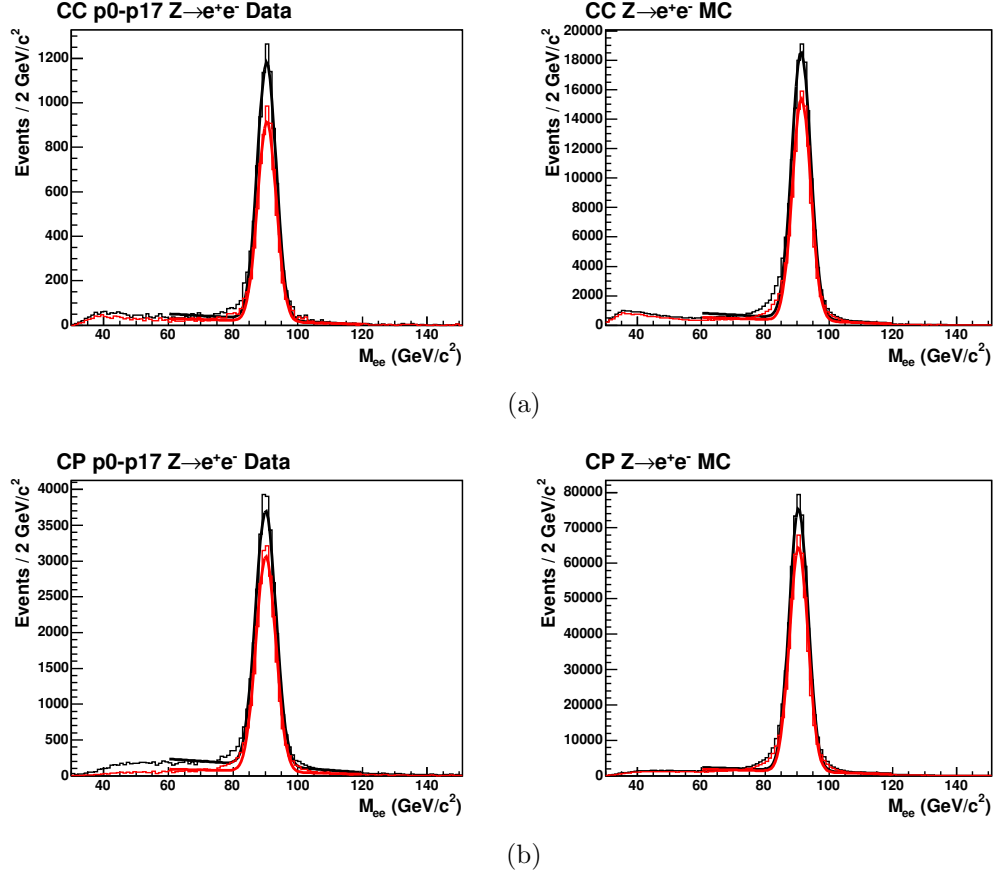
Figure 4.6: Example Z \rightarrow e^+e^- invariant mass ( M_{ee} ) plots are shown for the (a) central and (b) plug photon ID efficiency study. The black (red) histograms of each plot are from cases in which the probe electron leg passes loose (tight) cuts. The fit discussed in the text is also shown for each histogram. Plots obtained from the data (MC simulation) are shown on the left (right).
