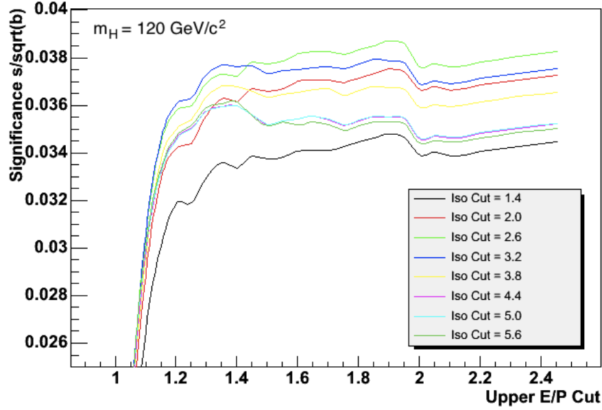
Figure 5.14: Optimization study on cuts applied to the conversion E/p and calorimeter isolation. For each trial, a symmetric cut is applied to the E/p shape, so that a cut of 1.9 on the x axis represents selecting conversions with 0.1 < E/p < 1.9 . The different colors represent different isolation cuts, such as requiring calorimeter isolation to be less than 2.6 GeV.
