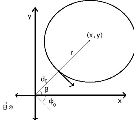
Figure B.1: The helical track for a positively-charged particle in the r-\phi plane. The CDF magnetic field points along the negative z axis. For q > 0 , the angle \beta = \phi_0 + \frac{\pi}{2} with 0 < \phi_0 < 2\pi . The figure is not drawn to scale relative to the detector geometry, but rather demonstrates the calculations performed based on track parameters.
