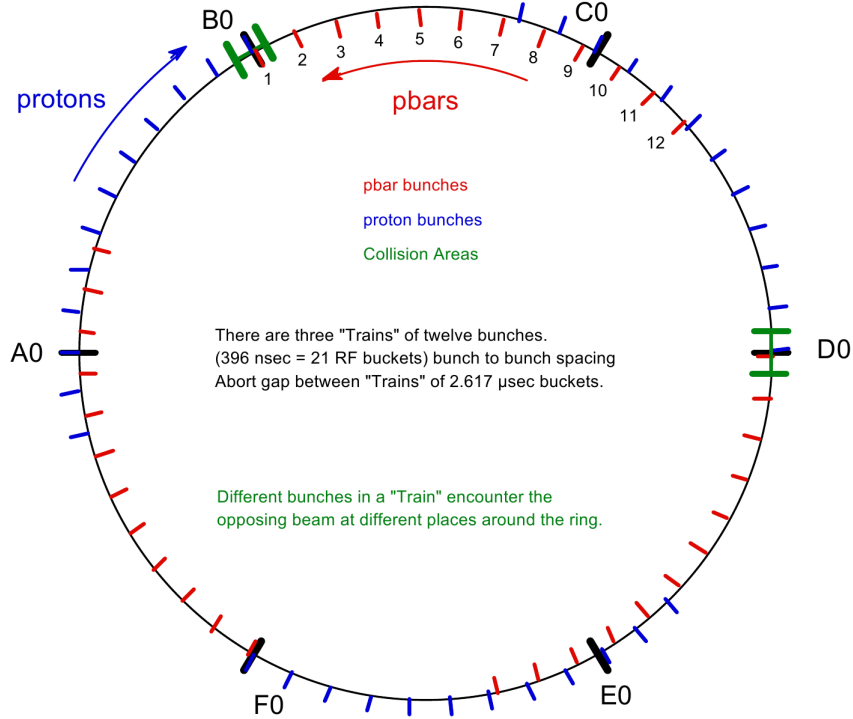
Figure 2.3: Proton and antiproton beams are shown [37] divided into three trains of 12 bunches each. This gave 36 proton bunches and 36 antiproton bunches. A gap between trains allowed for beams to be cleanly dumped (aborted).
