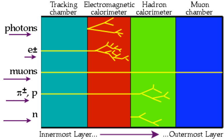
Figure 3.2: Diagram [40] showing which detector regions are sensitive to different types of particles. The left side of the figure corresponds to the innermost cylindrical layer of the detector, near the beam line, and the right side of the figure corresponds to the outermost layer of the detector.
