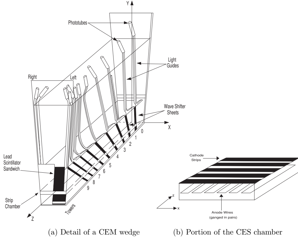
Figure 3.12: Diagrams showing the orientation of the cathode strips and anode wires of the CES detector, also indicating the local CES x and z axes [40]. The CES detector is located 6 radiation lengths into the CEM.
