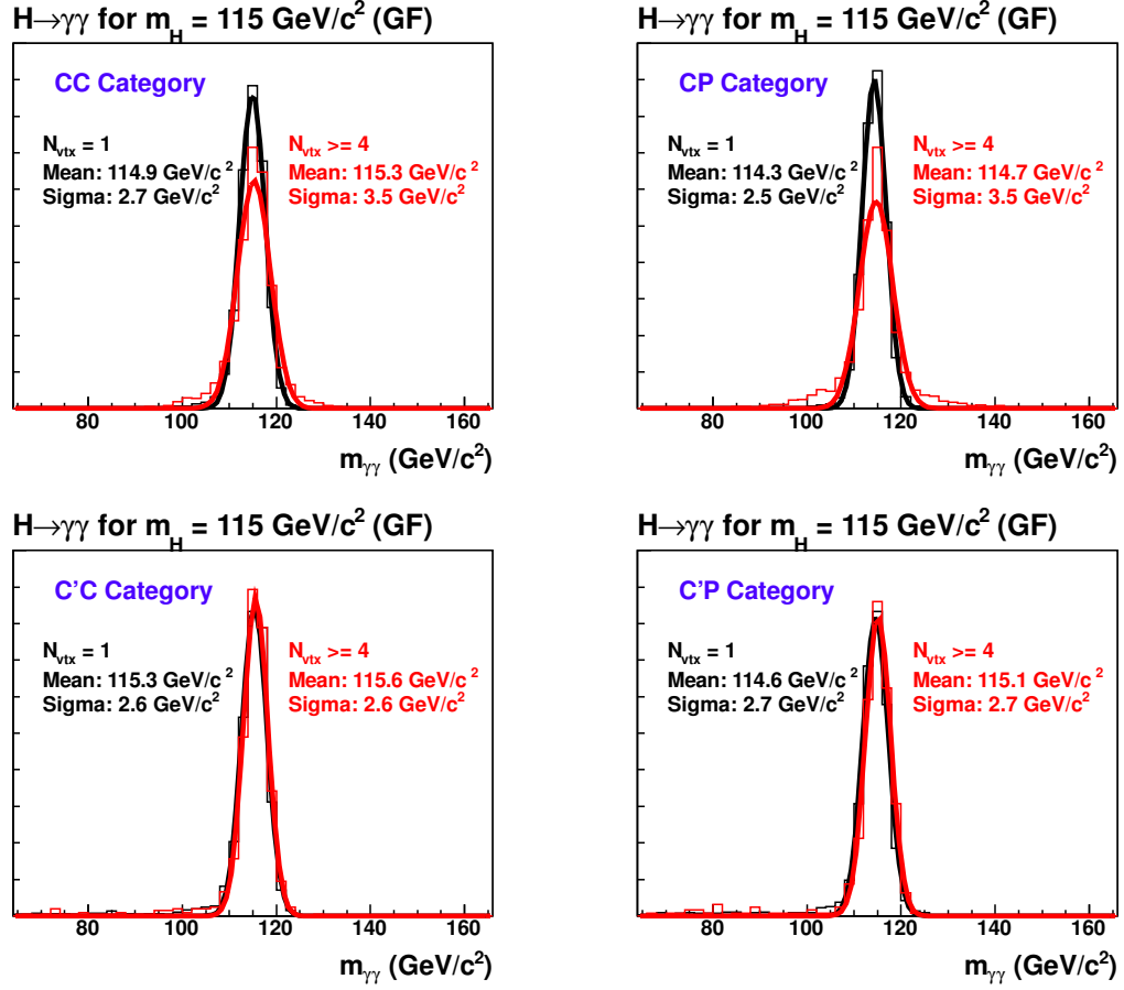
Figure 8.3: For m_H = 115 \text{ GeV}/c^2 , the signal resolution (in \text{GeV}/c^2 ) for GF production is shown, determined from a Gaussian fit made to the m_{\gamma\gamma} distribution.
