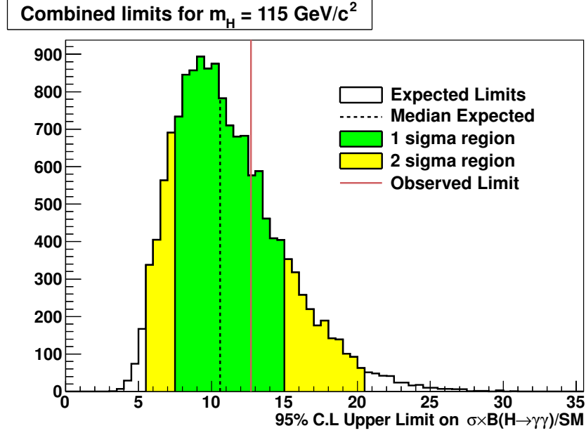
Figure 11.2: For m_H = 115 \text{ GeV}/c^2 and using all four categories, a distribution of 95% upper credibility level limits on the production cross section multiplied by the H \rightarrow \gamma\gamma branching ratio relative to the SM prediction. The expected limit distribution is shown with the median, \pm 1\sigma , and \pm 2\sigma regions. The observed limit is also shown as the vertical line (from Figure 11.1).
