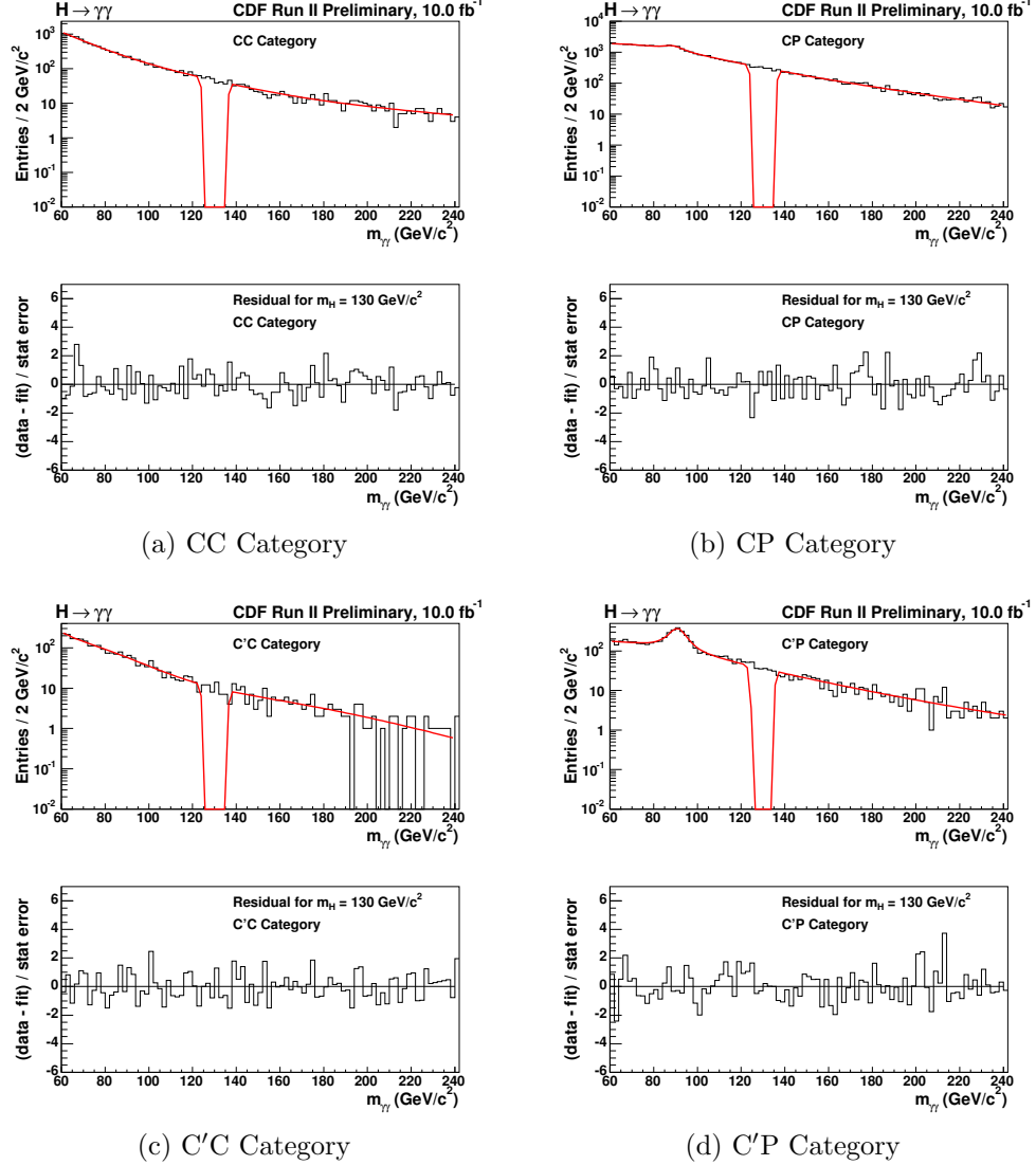
Figure D.7: Each subfigure shows a fit (red line) made to the sideband region of the data for each diphoton category using Equation (7.1) for the CC and C'C categories and the sum of Equations (7.1) and (7.2) for the CP and C'P categories. The two vertical red lines in each figure indicate the signal window excluded from the fit, here for a Higgs boson mass of 130 \text{ GeV}/c^2 . The bottom plot in each subfigure is obtained from first interpolating the fit into the signal region in order to obtain the background prediction in the signal region. The residual shown is then the resulting data yield minus the background yield, divided by the statistical error from the background yield.
