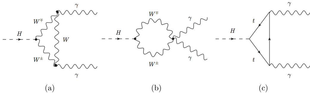
Figure 1.7: Diagrams of the Higgs boson decay to a pair of photons, obtained most often through a W or top loop [28].
