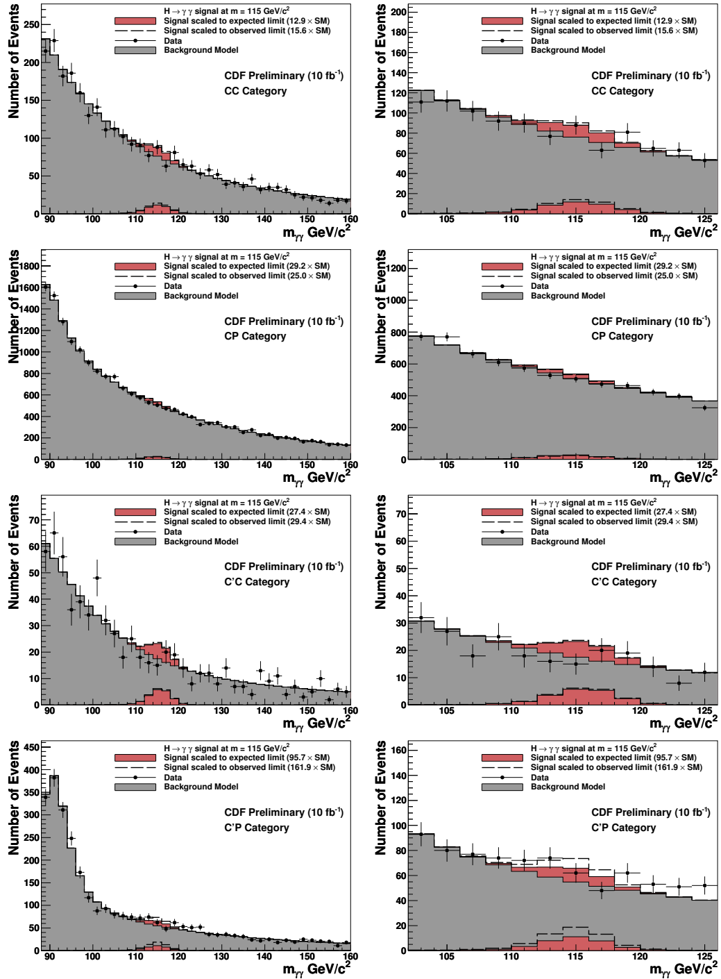
Figure 11.4: Invariant mass distribution over (left) the whole mass range and (right) zoomed in, for an example theoretical SM Higgs mass at 115 \text{ GeV}/c^2 . The signal is shown scaled to the expected and observed limits obtained from the respective category alone.
