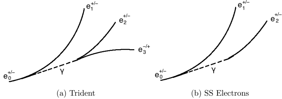
Figure 5.23: (a) Illustration of a trident, which has two electron tracks of the same sign and a third track with opposite sign. (b) An illustration of the same-sign (SS) electron tracks that we reconstruct for Method B.
