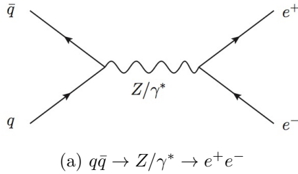
Figure 7.5: Diagram of the Drell-Yan process.
