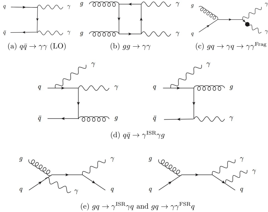
Figure 7.1: Diagrams [28, 66] of prompt diphoton production at hadron colliders. The LO process at the Tevatron is quark-antiquark annihilation in (a). The black circle shown in (c) represents a fragmentation process of a final-state quark radiating a photon, which takes most of its energy and which radiates at very small angle. The diagrams for (c) and (e) are time-like processes, however there are also the equivalent space-like processes.
