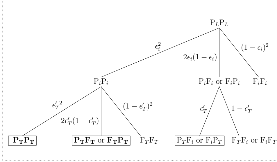
Figure A.1: The categorization of events based on \epsilon_i and \epsilon_T , relative to events that contain two loose central electrons.
