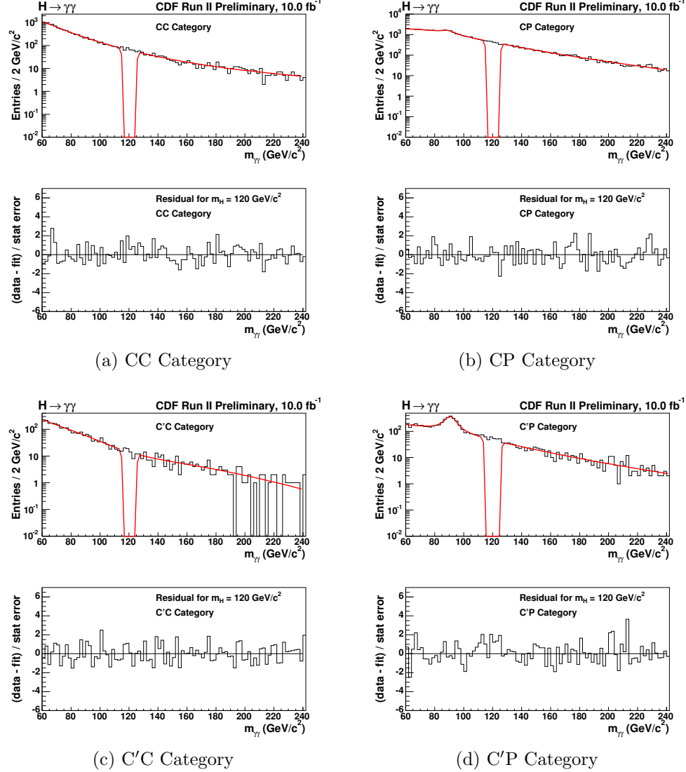
Figure D.5: Each subfigure shows a fit (red line) made to the sideband region of the data for each diphoton category using Equation (7.1) for the CC and C'C categories and the sum of Equations (7.1) and (7.2) for the CP and C'P categories. The two vertical red lines in each figure indicate the signal window excluded from the fit, here for a Higgs boson mass of 120 \text{ GeV}/c^2 . The bottom plot in each subfigure is obtained from first interpolating the fit into the signal region in order to obtain the background prediction in the signal region. The residual shown is then the resulting data yield minus the background yield, divided by the statistical error from the background yield.
