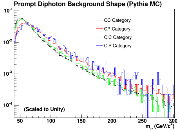
Figure 7.2: The prompt diphoton background shape for each diphoton category is shown, obtained from a \gamma\gamma PYTHIA sample including the LO diagrams (a) and (b) of Figure 7.1, but also modified to include diagrams (d) and (e) [66]. Each shape is normalized to unit area.
