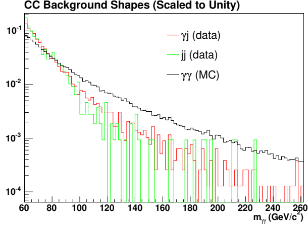
Figure 7.4: As an example, the shape of the \gamma + jet and dijet backgrounds in the CC data are shown, normalized to unit area. The enriched fake data samples are obtained by selecting diphoton events in the same way as that for the CC diphoton data, except one or both photons have a NN value < 0.3 rather than both passing the standard > 0.74 requirement. The prompt CC diphoton background shape from Figure 7.2 is also shown for comparison.
