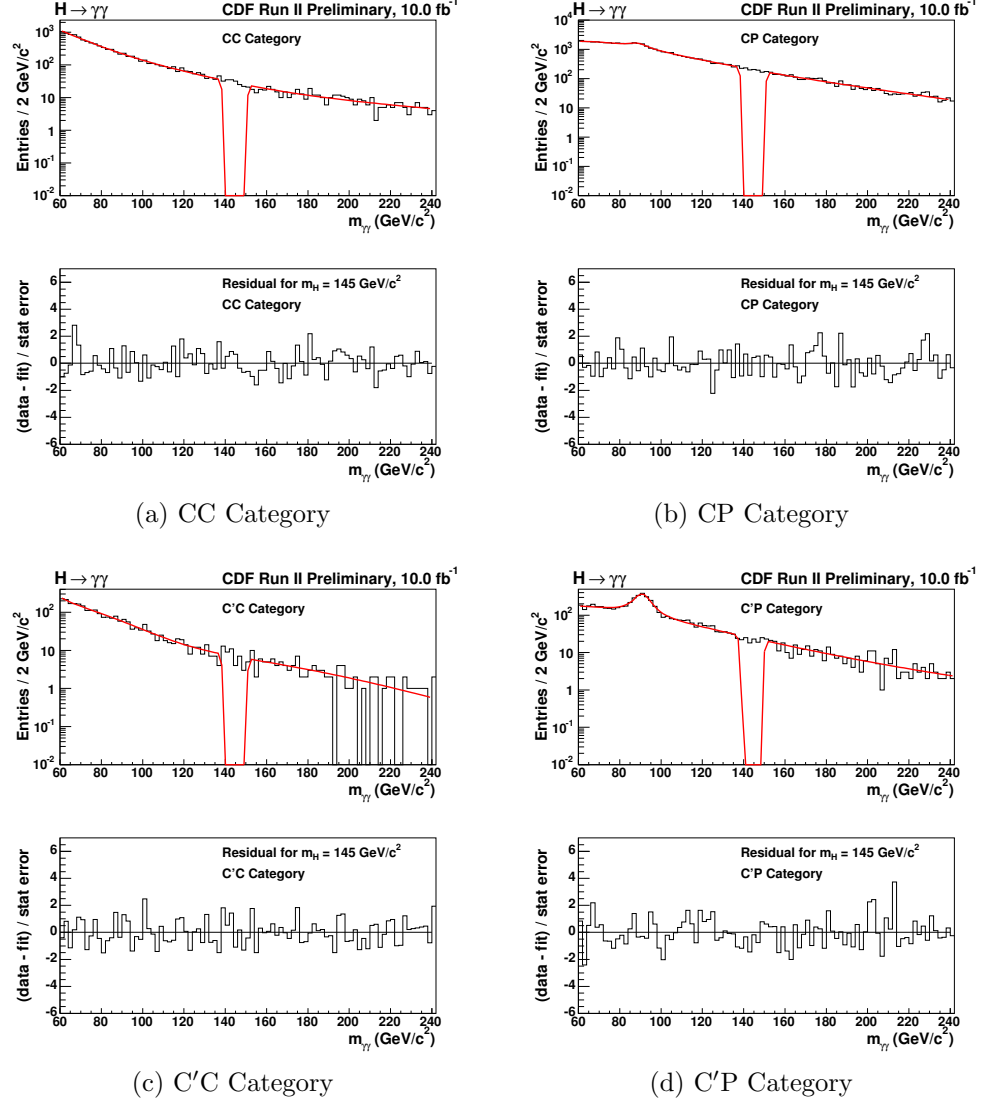
Figure D.10: Each subfigure shows a fit (red line) made to the sideband region of the data for each diphoton category using Equation (7.1) for the CC and C'C categories and the sum of Equations (7.1) and (7.2) for the CP and C'P categories. The two vertical red lines in each figure indicate the signal window excluded from the fit, here for a Higgs boson mass of 145 \text{ GeV}/c^2 . The bottom plot in each subfigure is obtained from first interpolating the fit into the signal region in order to obtain the background prediction in the signal region. The residual shown is then the resulting data yield minus the background yield, divided by the statistical error from the background yield.
