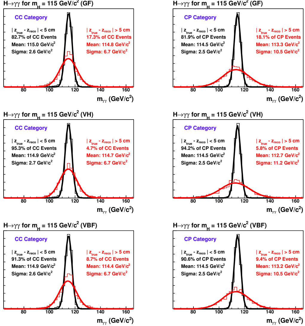
Figure 8.4: For an example Higgs boson mass of m_H = 115 \text{ GeV}/c^2 , the GF, VH, and VBF H \rightarrow \gamma\gamma diphoton mass shapes are shown for events where a correct and incorrect vertex are reconstructed. These are provided for CC and CP categories only since the effect is negligible for C'C and C'P events.
