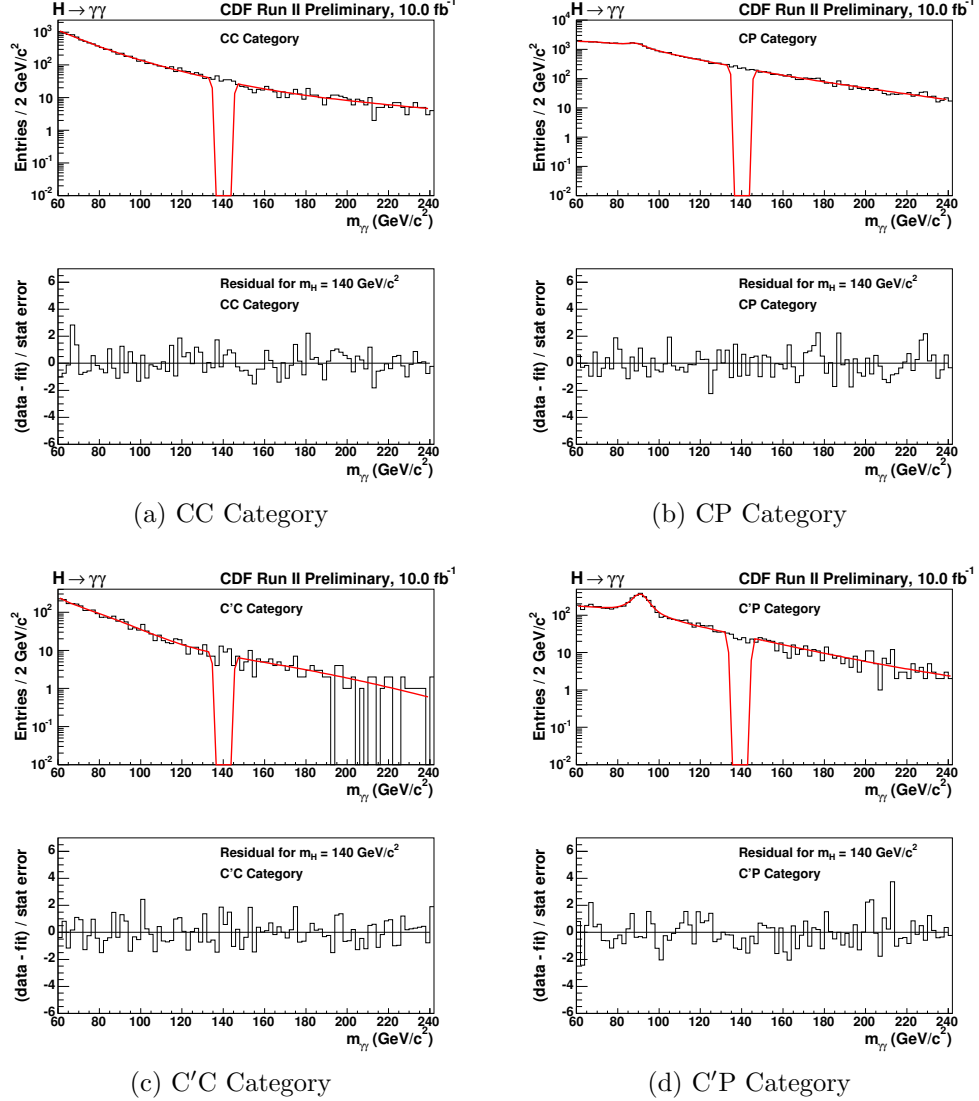
Figure D.9: Each subfigure shows a fit (red line) made to the sideband region of the data for each diphoton category using Equation (7.1) for the CC and C'C categories and the sum of Equations (7.1) and (7.2) for the CP and C'P categories. The two vertical red lines in each figure indicate the signal window excluded from the fit, here for a Higgs boson mass of 140 \text{ GeV}/c^2 . The bottom plot in each subfigure is obtained from first interpolating the fit into the signal region in order to obtain the background prediction in the signal region. The residual shown is then the resulting data yield minus the background yield, divided by the statistical error from the background yield.
