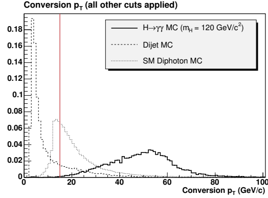
Figure 5.11: The p_T distribution for conversions reconstructed in H \rightarrow \gamma\gamma , dijet, and QCD diphoton MC samples; each histogram is scaled to unity. Conversion photons from Higgs boson decays have a higher than average p_T value compared to the backgrounds. Conversions from jets are from \pi^0/\eta \rightarrow \gamma\gamma decays and populate the lower p_T region; much of these are removed with a cut on this variable. All cuts made in the conversion selection have been applied, except for the cut on the variable shown ( N - 1 cuts).
