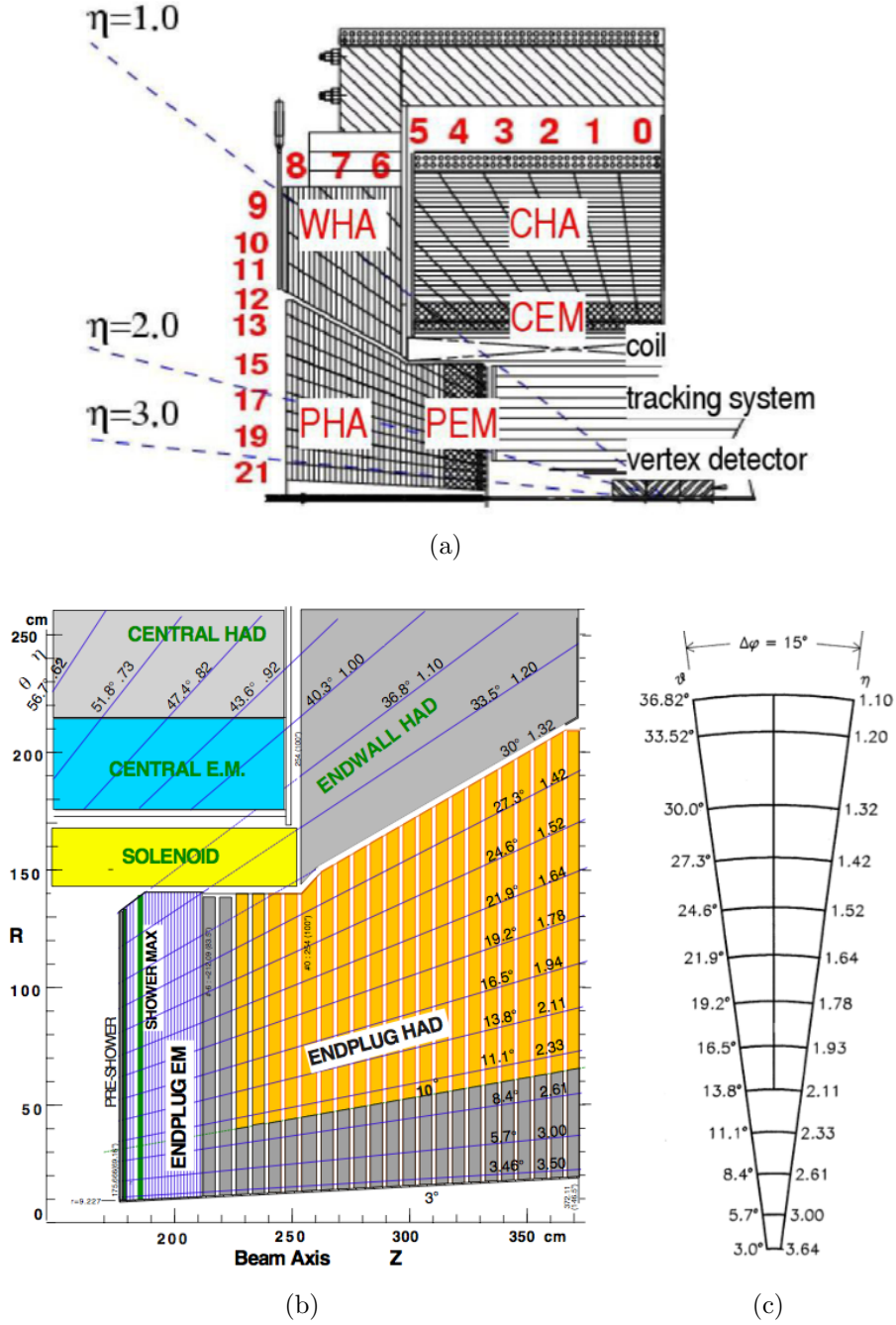
Figure 3.8: (a) One quadrant of the CDF detector showing the different calorimeter subdetectors. (b) Similar to (a), but more detail is shown for the plug calorimeters [40]. (c) The plug calorimeter segmentation for a single \phi wedge, also showing \theta and \eta boundaries for each tower in the wedge [43].
