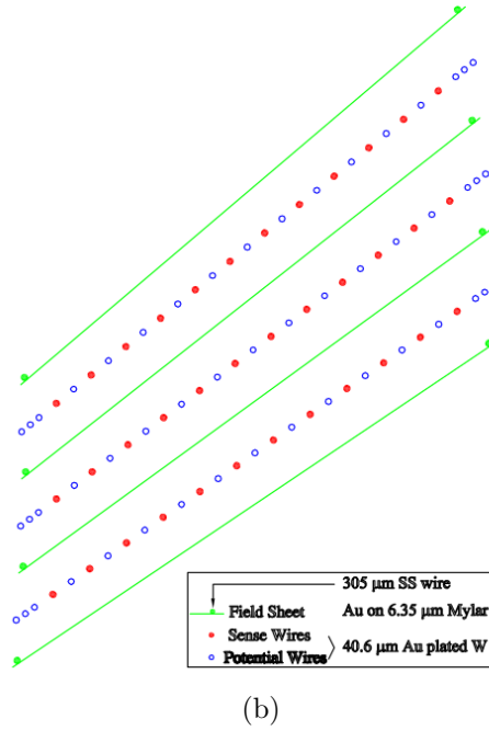
Figure 3.7: (a) The upper figure shows the a portion of the COT in the r - \phi plane. The number of cells per superlayer is given, along with whether the superlayer has axial or stereo wires. The radius of each layer relative to the beam line is also shown (in cm). The blow-up subfigure shows the geometry of the sense and field planes. (b) The lower figure provides a diagram demonstrating more detail of the field/sense planes, where three cells are shown. Each figure shown here is from Reference [42].
