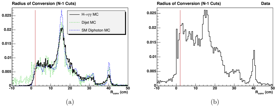
Figure 5.16: (a) The radius of conversion distribution for conversions reconstructed in H \rightarrow \gamma\gamma , dijet, and QCD diphoton MC samples. (b) The radius of conversion distribution for conversions reconstructed in the data described in Chapter 6. The red line shows where a cut is made on this variable.
