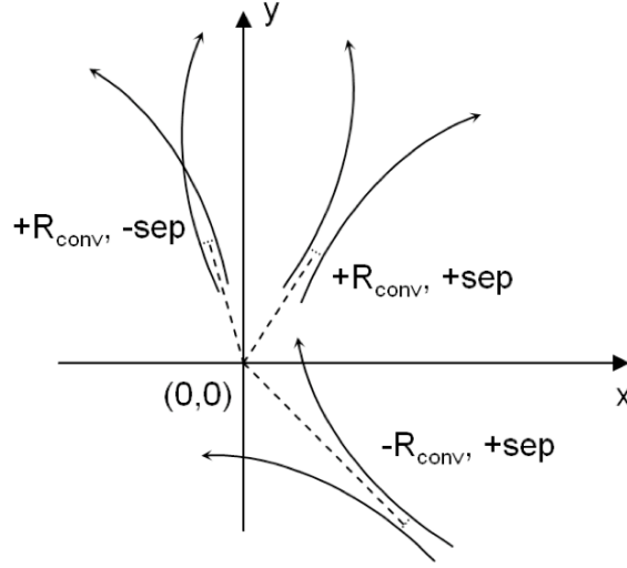
Figure 5.3: The radius of conversion, R_{conv} , is the radial distance from the center of the detector to the location where the two tracks are parallel. Sep is the spatial separation between the tracks in the r - \phi plane at this location. Three different conversion examples are shown [63] illustrating the R_{conv} variable as a dashed line and the sep variable as a dotted line. The R_{conv} is positive (negative) if the conversion points away from (towards) the origin and sep is positive (negative) if the electron-positron tracks do not (do) cross one another.
