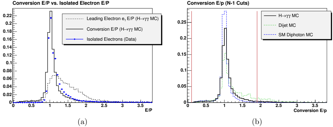
Figure 5.13: (a) The conversion E/p shape is compared to the leading electron's E/p shape and isolated electrons in the data. (b) The E/p shape for conversions reconstructed in H \rightarrow \gamma\gamma , dijet, and QCD diphoton MC samples. The red lines show where cuts are made on this variable.
