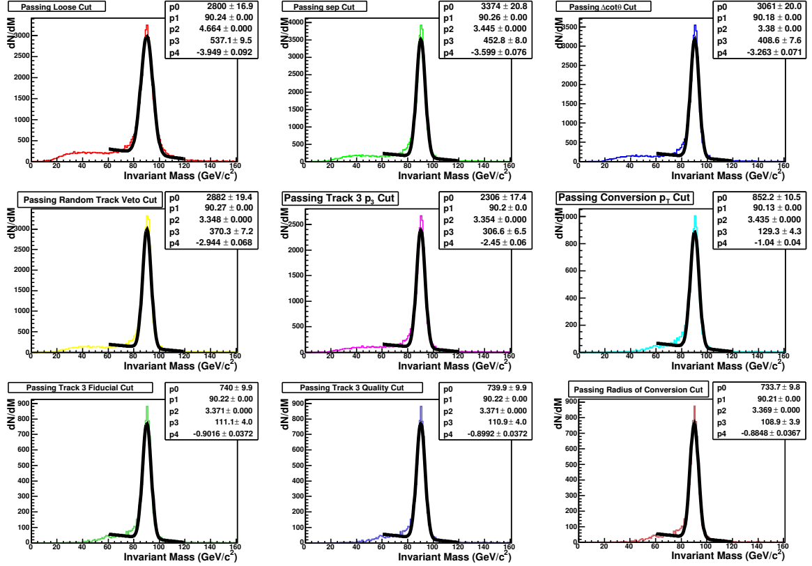
Figure 5.24: The invariant mass distribution of Z \rightarrow e + \text{trident} events in the data. The upper left distribution includes only the loose cuts of Table 5.6, which are cuts applied to the same-sign pair of the trident. For the remaining distributions, consecutively tighter cuts on the conversion have been applied. These are the cuts given in Table 5.7. Each histogram is fit to the sum of a Gaussian function and a polynomial function. The number of signal events is obtained from the integral in the range 83.0 < m_{ee} < 99.0 \text{ GeV}/c^2 , with the background subtracted from sideband regions 61.0 < m_{ee} < 69 \text{ GeV}/c^2 and 113.0 < m_{ee} < 121 \text{ GeV}/c^2 .
