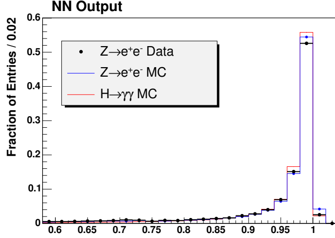
Figure 4.5: After all other cuts have been applied, the NN output for central electrons from Z decays in data and MC simulation is shown, demonstrating the similarity of the MC prediction to the data. The NN output for central photons from a H \rightarrow \gamma\gamma MC sample is also shown to demonstrate the similarity of the electron and photon response to the central ID selection. All histograms are normalized to unit area.
