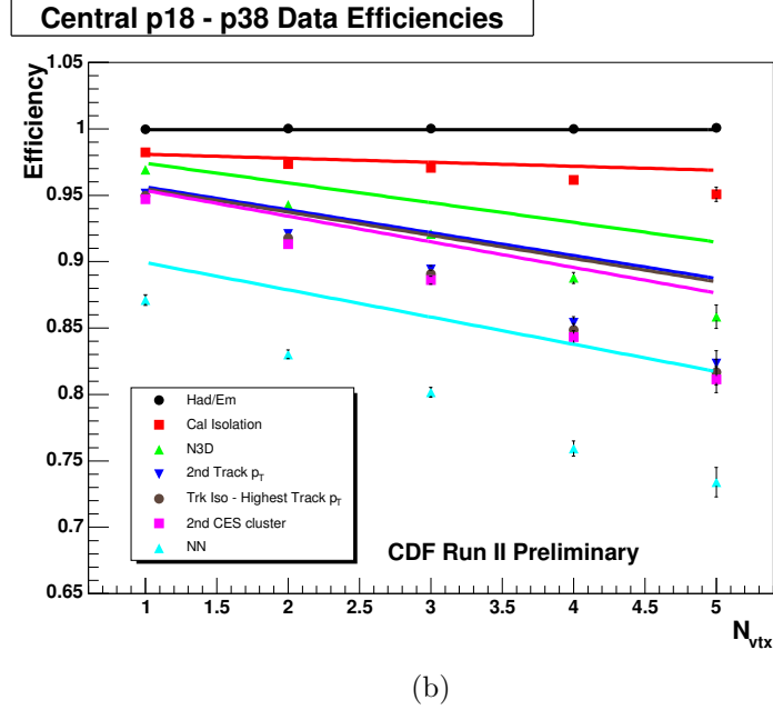
Figure 4.7: As a function of the number of vertices reconstructed in the event, cumulative central photon ID efficiencies are plotted for each cut made in the order they are shown. Efficiencies from the data are represented by markers (solid shapes) and efficiencies from the MC prediction are represented by lines. The same set of MC efficiency lines are drawn for both data periods. See the text for details on the upper and lower plots.
