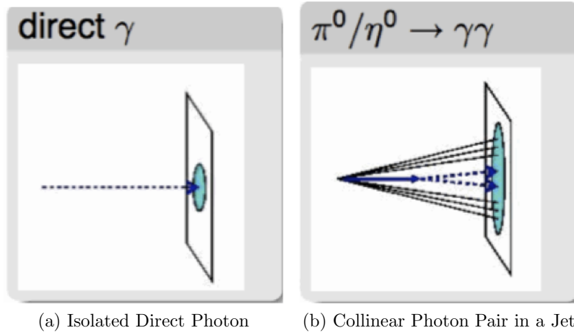
Figure 4.1: (a) Illustration of an isolated energy deposition from a direct (prompt) photon from the primary collision. (b) Illustration of an energy deposition from a collinear pair of photons from the decay of a neutral meson in the core of a jet [40]
