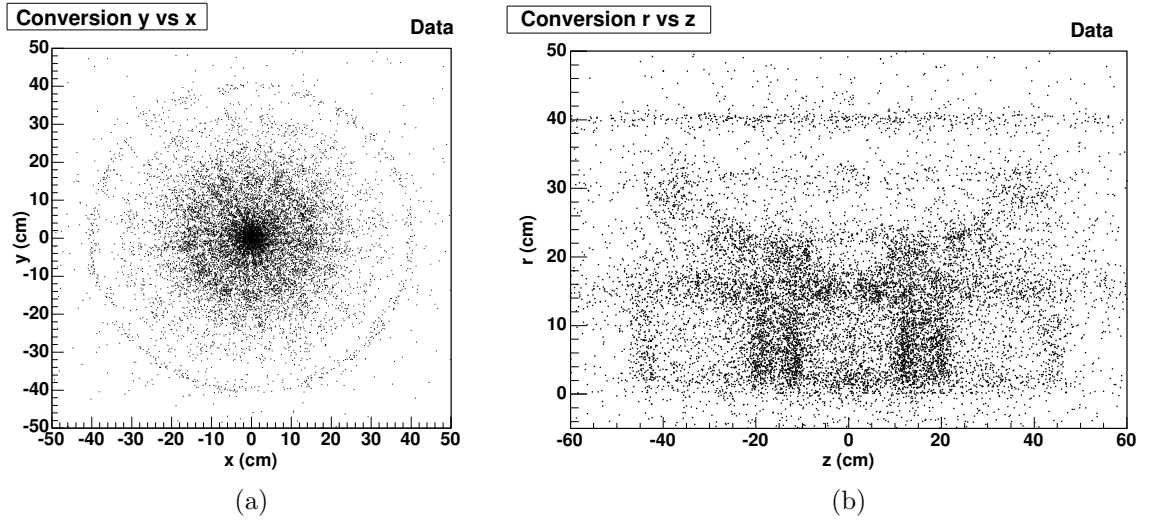
Figure 5.17: The reconstructed point of conversion in the (a) x - y view and (b) the r - z view for conversions reconstructed in data described in Chapter 6. All cuts described in this chapter have been applied except for the cut on R_{\text{conv}} .
