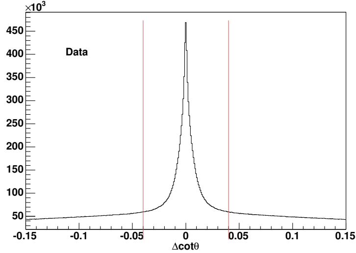
Figure 5.5: The \Delta \cot \theta distribution for electron candidate ( e_1 ) tracks and any other track in the event. True conversions populate the \Delta \cot \theta = 0 region. Red lines show where cuts are made. (The data sample is described in Chapter 6.)
