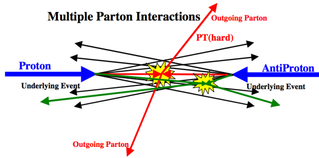
Figure 8.2: The same schematic and description as Figure 8.1 [76], except now a second pair of partons are shown having interacted, indicated by the green arrows moving away from the second vertex. Both beam remnants and multiple parton interactions contribute to the underlying event of the hard scattering process.
