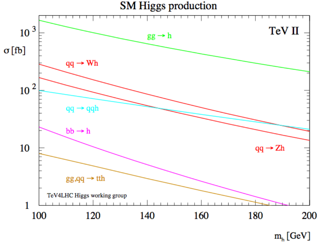
Figure 1.5: The dominant production mechanisms at the Tevatron for the SM Higgs boson [3, 25].
