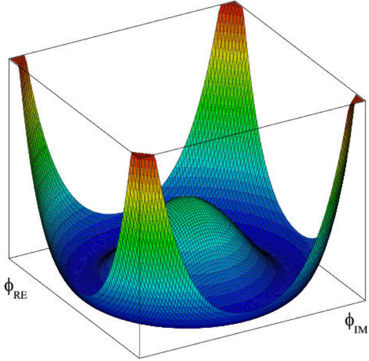
Figure 1.3: The shape of the Higgs potential when one field in Equation (1.6) is set to zero and the value of \lambda in Equation (1.8) is fixed. The figure [22] then shows the potential as a function of different values of the real and imaginary parts of the remaining scalar field.
