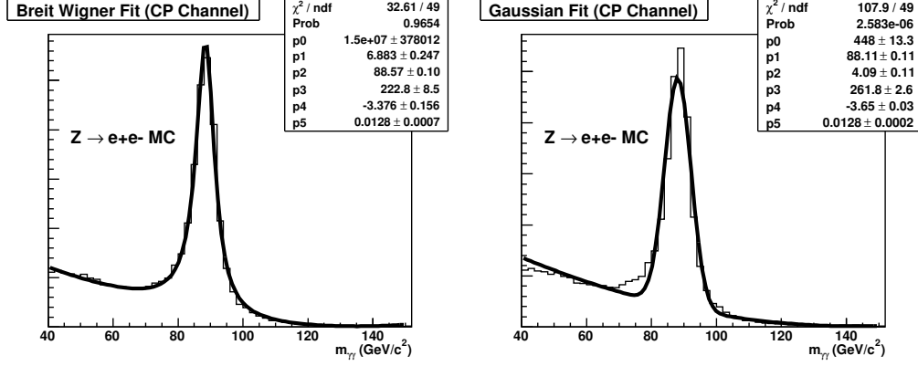
Figure 7.6: MC simulation of Z \rightarrow e^+e^- events that pass the diphoton selection for the CP category. The left and right plots show the m_{\gamma\gamma} distribution fit to a Breit-Wigner and Gaussian function, respectively. The former better describes the shape and is used when fitting to the Z contribution in the data. In the left plot, the parameters p_0 – p_2 correspond to those described in Equation (7.2).
