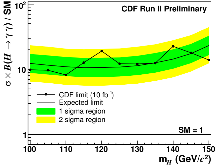
Figure 11.6: 95% C.L. upper limits on the production cross section multiplied by the H \rightarrow \gamma\gamma branching ratio, relative to the SM prediction, for categories combined.
