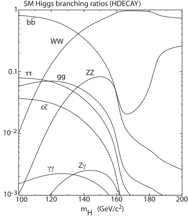
Figure 1.6: Possible decay modes for the SM Higgs boson for masses between 100 and 200 \text{GeV}/c^2 [27].
