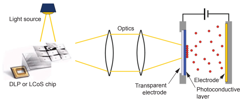
Figure 2. Process schematic of EPD. Electric fields are used to deposit charged nanoparticles from a solution onto a substrate. Once the particles are deposited, the green body can be post-processed to produce the final part.
