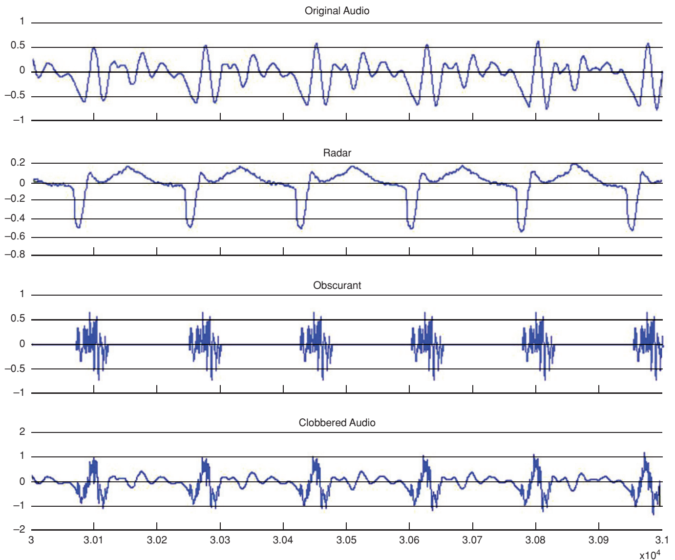
Figure 2. Illustration of the effect of introducing correlated additive white Gaussian noise onto the radar-triggered voiced portion of the acoustic signal.
