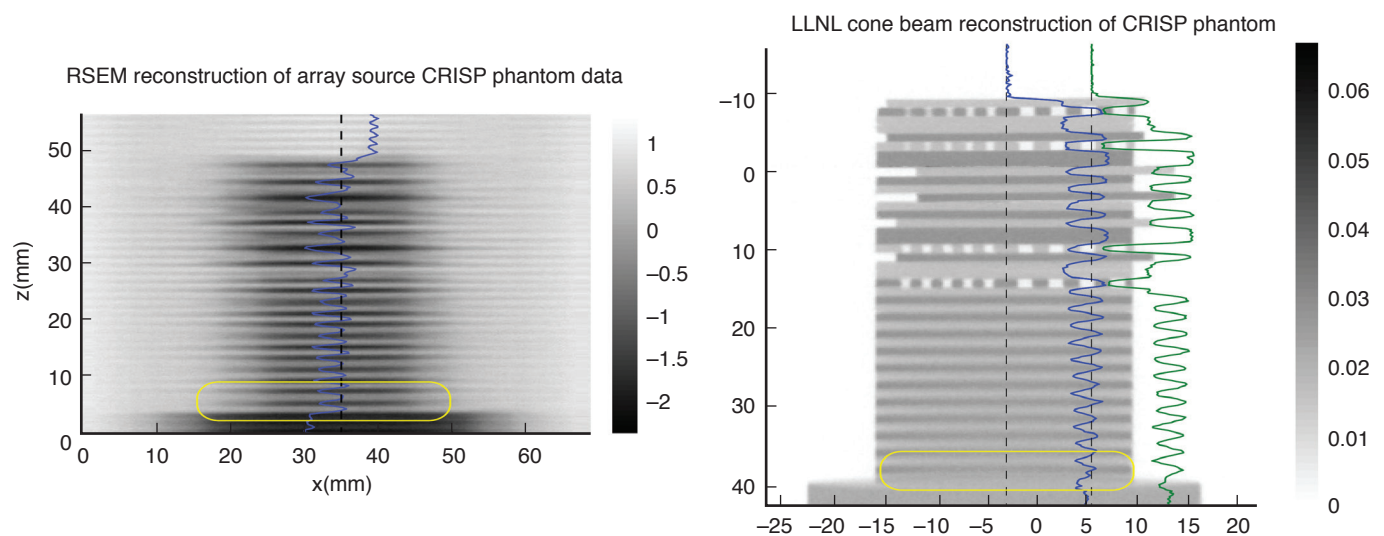
Figure 3. Reconstruction comparison of vertical slices through the cone-beam array-source data (left) and a single-source cone-beam data (right). Superimposed on the images are line profiles through the data. Cone-beam artifacts are reduced in the array-source data, as indicated by the yellow boxes.
