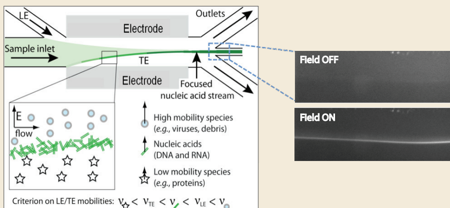
Figure 7. A sketch of the physical mechanism that enables DNA focusing by transverse free-flow ITP. Migrating ions line up in order of their mobilities under the transversely-applied electric field, with nucleic acids focusing into a tight band. The images at right show focusing of fluorescently-stained DNA.
