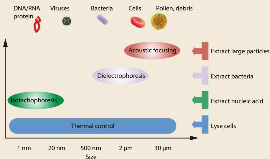
Figure 3. Size is one of the key physical properties by which LLNL's devices separate samples. This figure shows typical particles that can be manipulated by each of LLNL's four modules.
