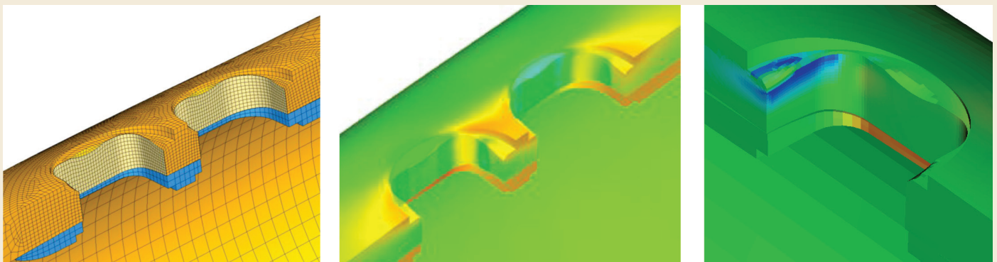
Figure 3. Samples of the modeling simulation and results of the composite case features.
