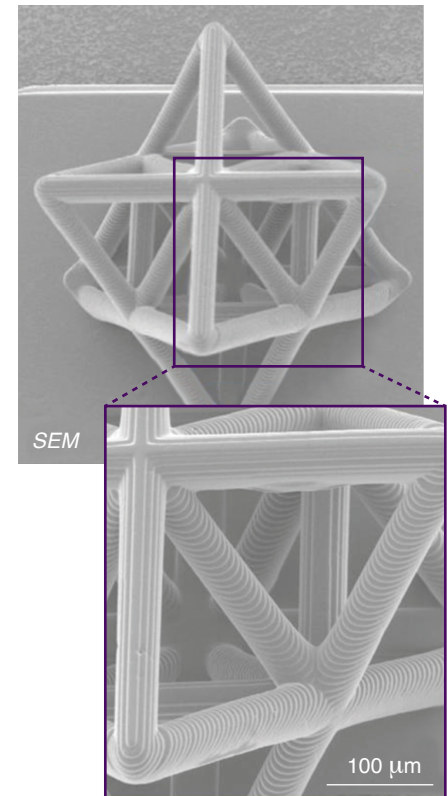
Figure 4. The smallest known embodiment of the octet truss, fabricated with PμSL.
