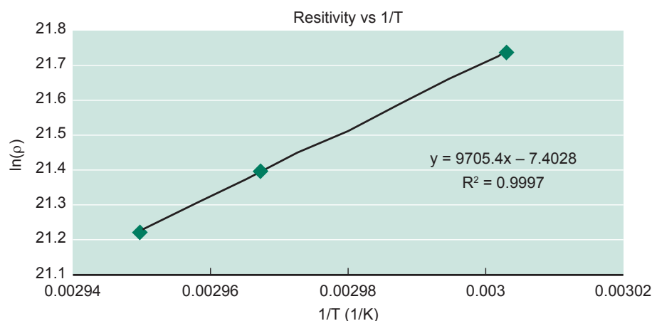
Figure 4. Arrhenius plot of the resistivity for deposited a-Se films.
