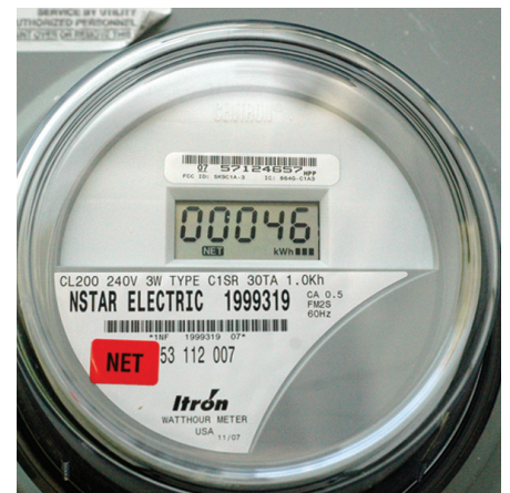
Figure 4. Smart meter.
