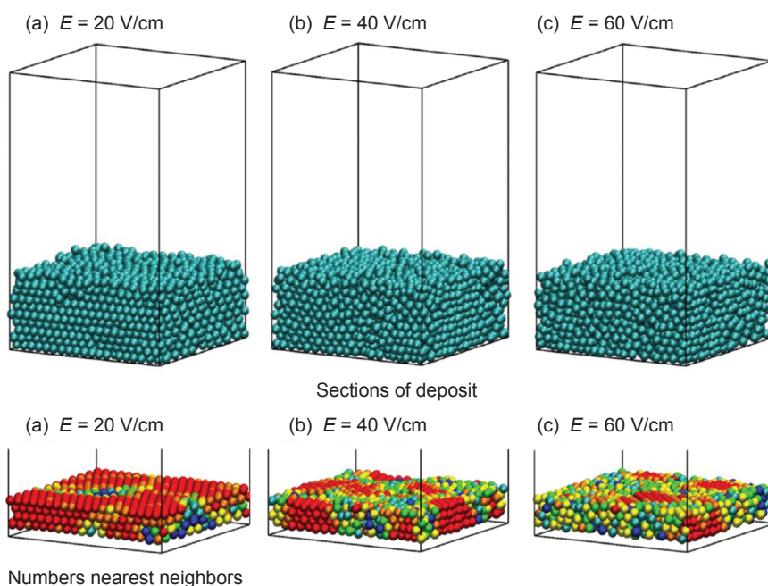
Figure 2. Demonstration of ordered-to-disordered transition for both experiments and modeled depositions. Higher electric field strength results in disordered deposits.
