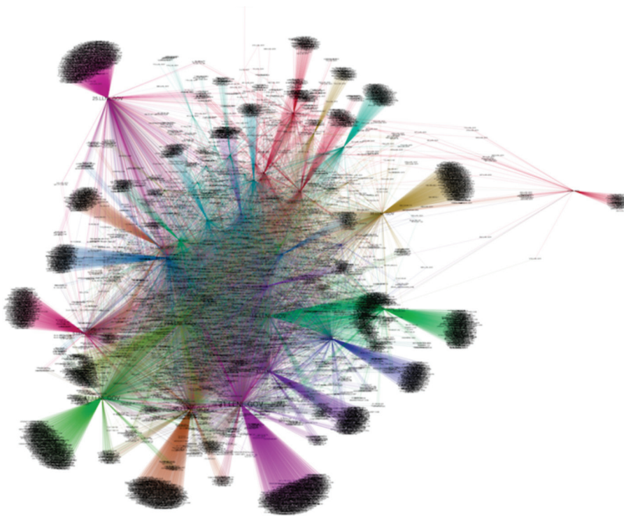
Figure 1. Visualization of LLNL-based network connections collected by the Foraker distributed sensor network over a period of one month. Nodes represent unique IP addresses; edges are colored to highlight community structures within the graph.
