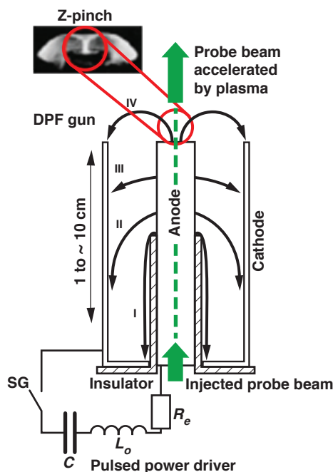
Figure 1. DPF and the proposed probe beam injection experiment. The Z-pinch plasma is formed at the end of a coaxial gun through multiple stages. The plasma sheath starts from flashover of the insulator (I), accelerates down the electrode along the coaxial gun (II, III), and collapses radially (IV) to form a dense, fast Z-pinch (inset).
