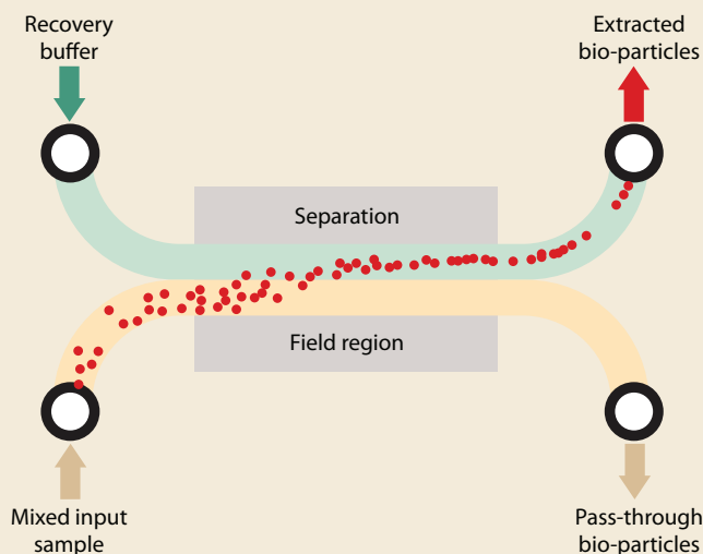
Figure 1. A summary of the common features of LLNL's microfluidic separation devices. A mixed input sample is introduced and flows side-by-side with a clean buffer (the streams do not mix), into which a set of particles is shifted by an applied field. The rest of the sample passes through. Channel dimensions are 10s to 100s of micrometers in width and depth and a few centimeters in length.
