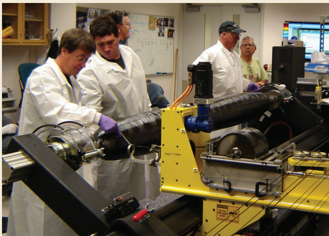
Figure 5. Case winds were carefully monitored and measured to provide consistency.
