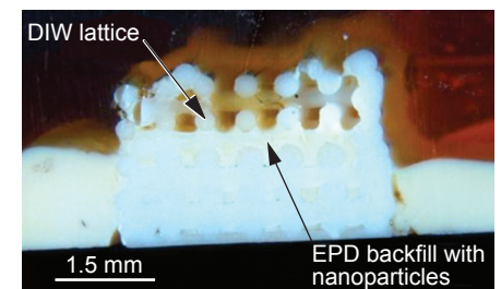
Figure 5. EPD combined with DIW to backfill a lattice with nanoparticles to obtain unique combinations of materials in a single structure.
