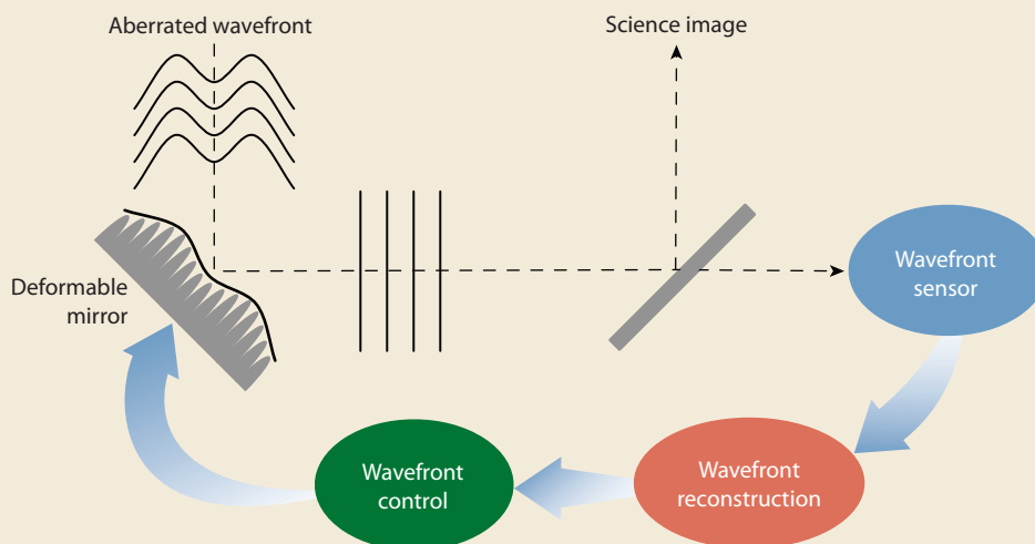
Figure 1. Adaptive Optics improves image quality by correcting the aberrated incoming wavefront. Correction is performed by phase conjugation with the adjustable surface of a deformable mirror. GPI's advanced wavefront sensing, reconstruction, and control methods enable high-contrast direct imaging.
