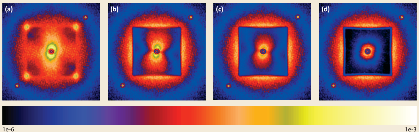
Figure 2. Simulated GPI AO coronagraphic images demonstrating the performance improvement with new advanced algorithms. Log-scale scattered light levels are from 10^6 to 10^3 less than the planet's brightness. (a) FTR enables a system with thousands of actuators. The resulting image is nearly diffraction-limited but has low contrast due to a structured halo of scattered light. (b) The spatially filtered wavefront sensor prevents aliasing and creates a "dark hole" of improved contrast. The remaining scattered light in this simulation is from residual atmospheric and noise errors. (c) OFC determines the optimal controller gain for each Fourier mode during closed-loop operation, resulting in improved performance throughout the dark hole. The hourglass shape of scattered light is due to frozen-flow atmospheric turbulence. (d) PFC detects multiple layers and uses a Kalman filter to predict the turbulence and to further improve contrast.
