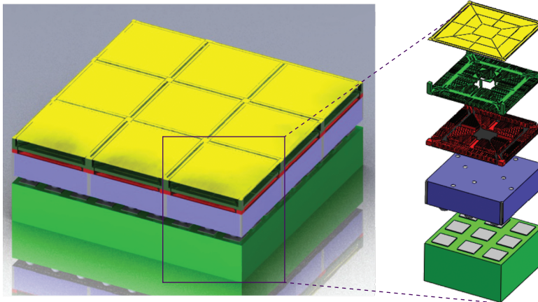
Figure 1. Micro-mirror array configuration.
