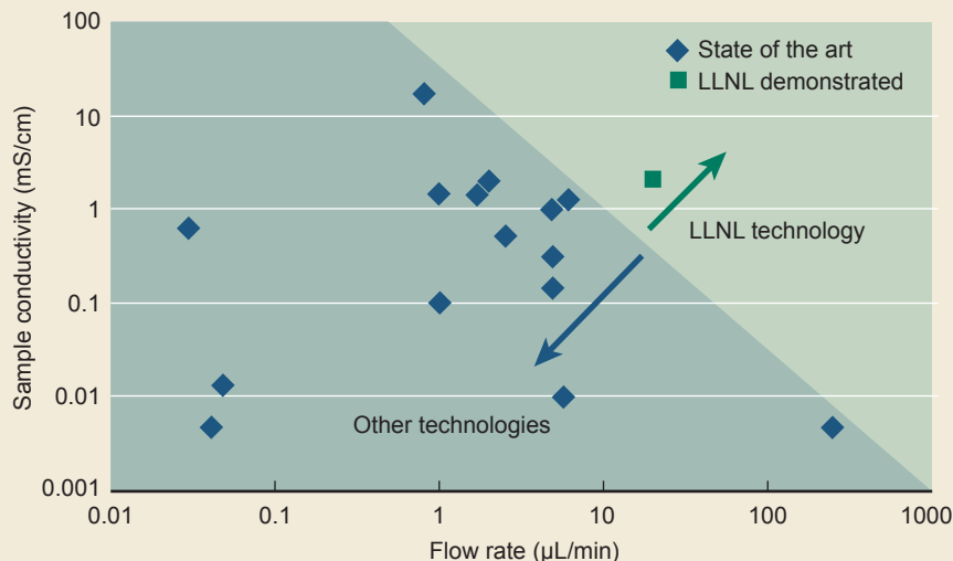
Figure 5. This plot highlights the advantage of LLNL's DEP device over alternative technologies.
