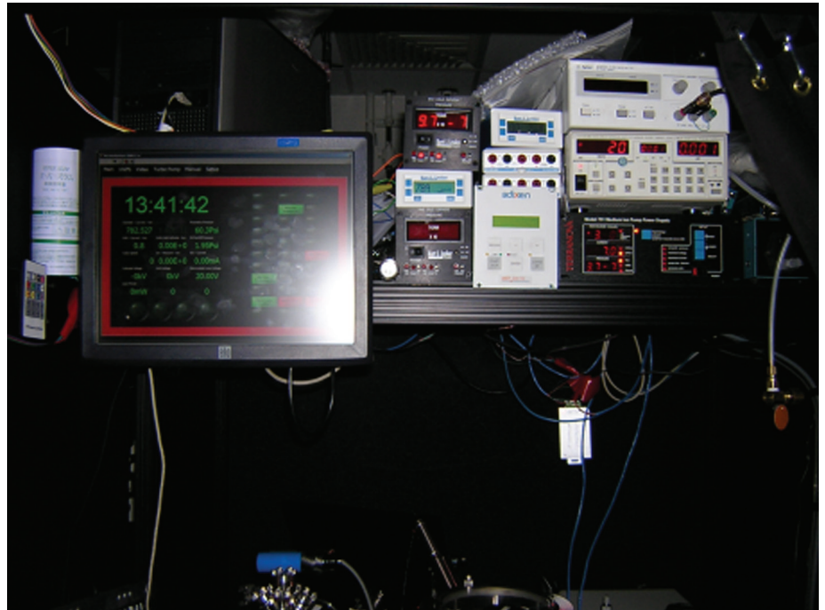
Figure 2. Testbed for experimental control systems.
