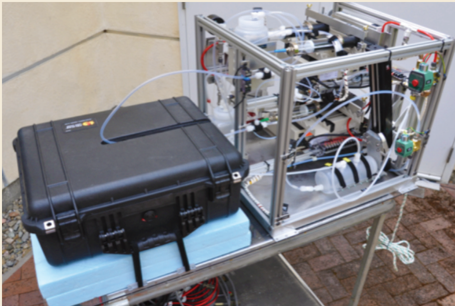
Figure 2. (top) Remote handling system used for the production of sensitive liquid explosives and Pelican case that holds the specimen that is scanned in the CT system. (right) The open Pelican case shows the specimen bottle inside that is filled with the sensitive liquid explosive prior to a CT scan.
