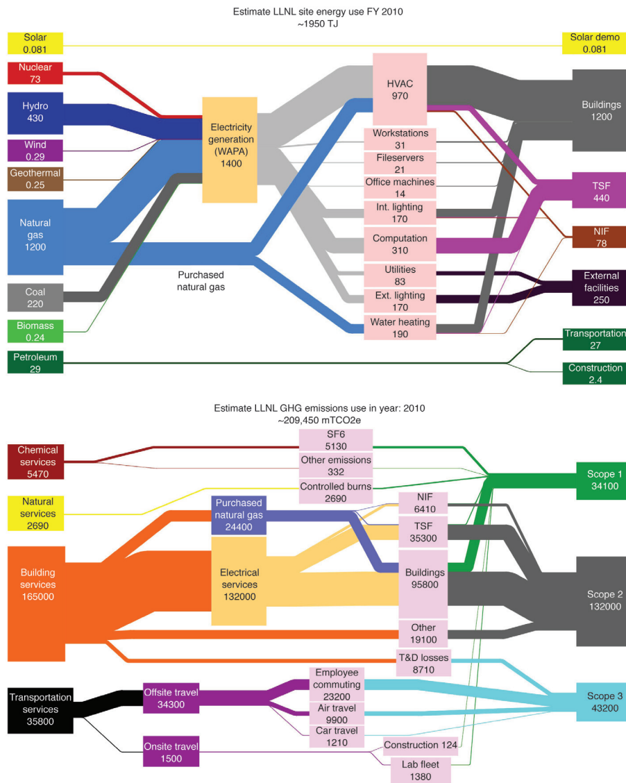
Figure 2. Visualization of the LLNL site energy use, showing which locations and services demand electricity and natural gas, as well as the energy sources for LLNL.
