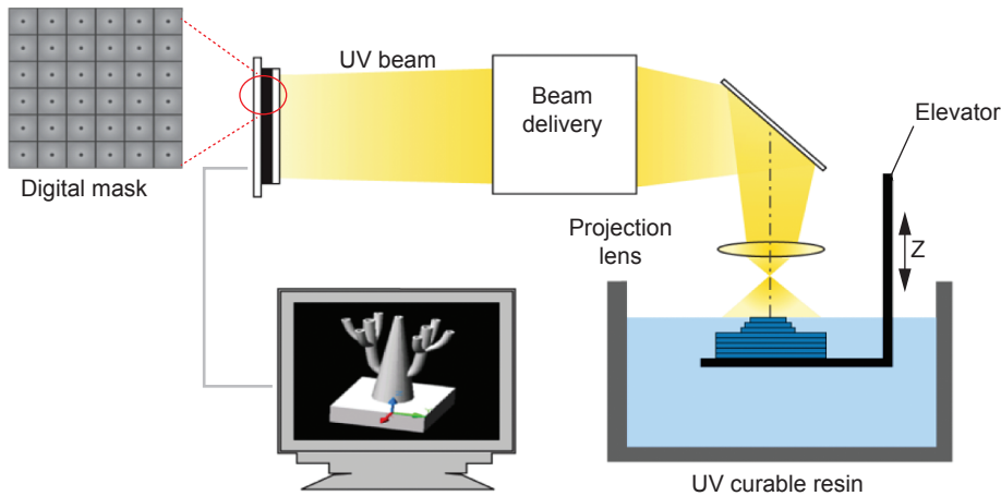
Figure 1. Process schematic of PμSL. A CAD model is sliced into a series of closely spaced horizontal planes. The slices are digitized as an image and transmitted to a spatial light modulator that projects the image through a reduction lens into a bath of photosensitive resin. The exposed material cures and the substrate on which it rests is lowered to repeat the process with the next image slice.
