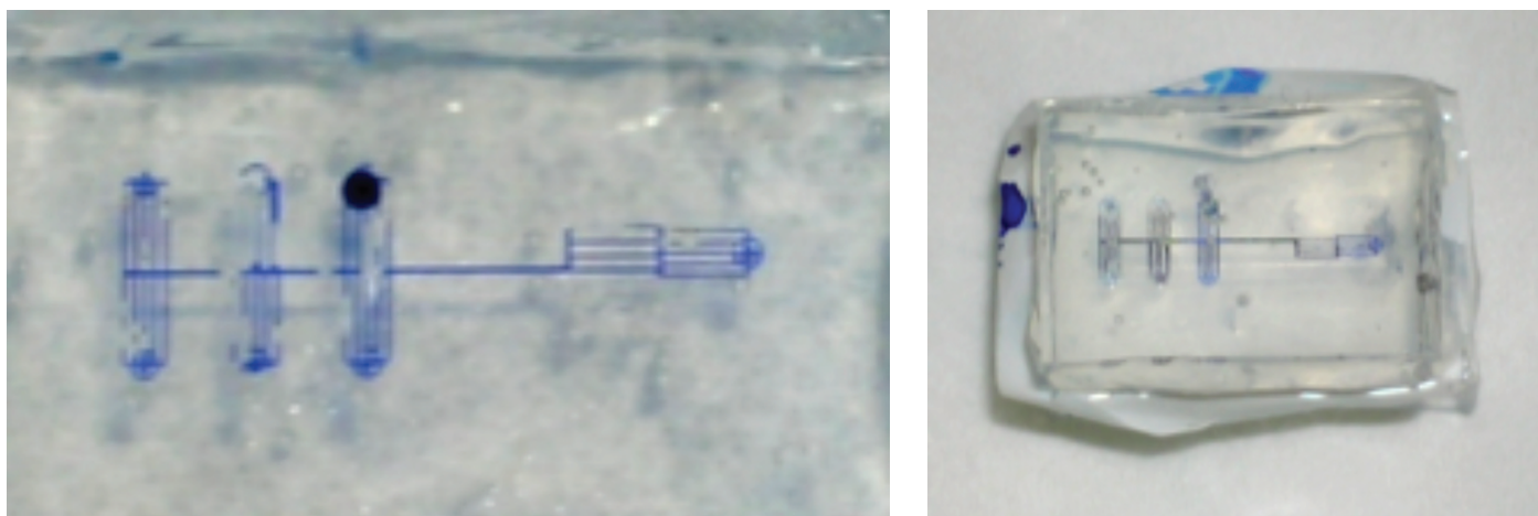
Figure 2. Two views of the dye-solution-filled microchannels, with no visible leaks at 15 psi. The sample is leak-free during the test at 7 psi for four days. All channels on both PDMS devices were filled with liquid.
