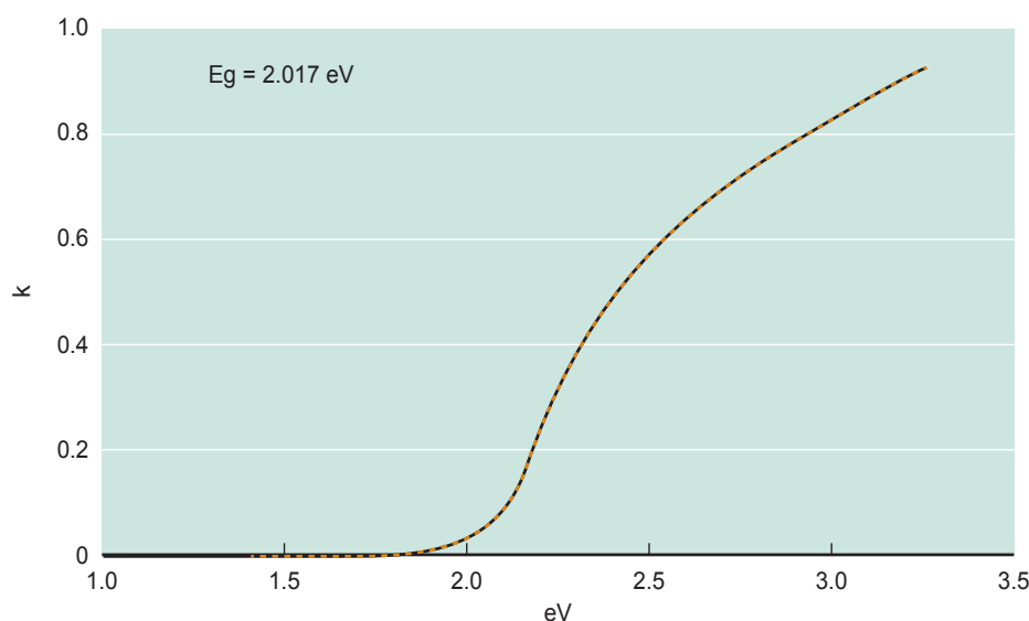
Figure 3. Modeled ellipsometric value for the extinction coefficient and band gap using a Cody-Lorentz oscillator.
