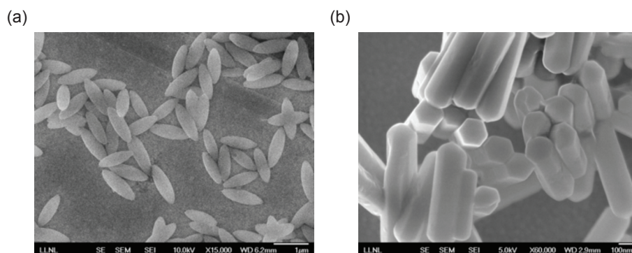
Figure 3. Representative fluorapatite nanorods with morphology managed through control of the degree of supersaturation during synthesis and growth.
