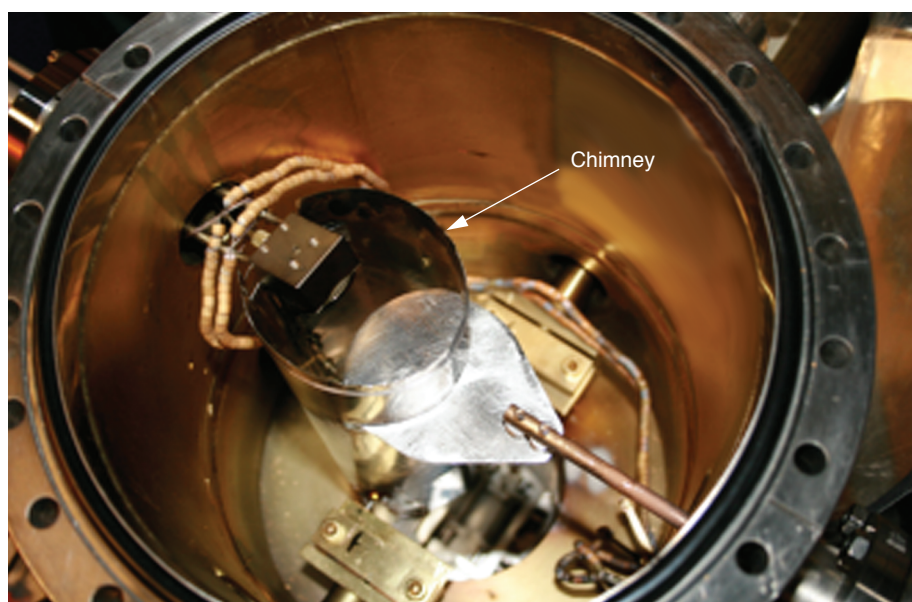
Figure 1. Safety features of a-Se thermal evaporation system.
