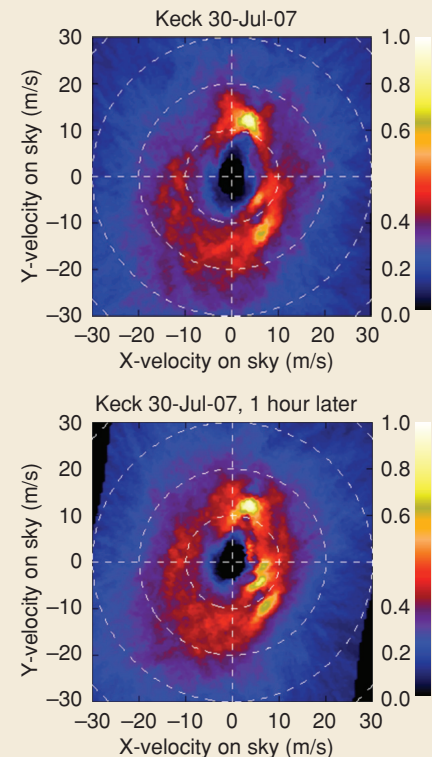
Figure 4. “Windmaps” showing the likelihood of a layer of frozen flow at a given velocity vector, based on analysis of Keck AO system telemetry during regular closed-loop observations. (top) First observation on July 30, 2007. Four layers are easily identifiable. (bottom) One hour later the wind velocities are very similar, and three layers are evident.
