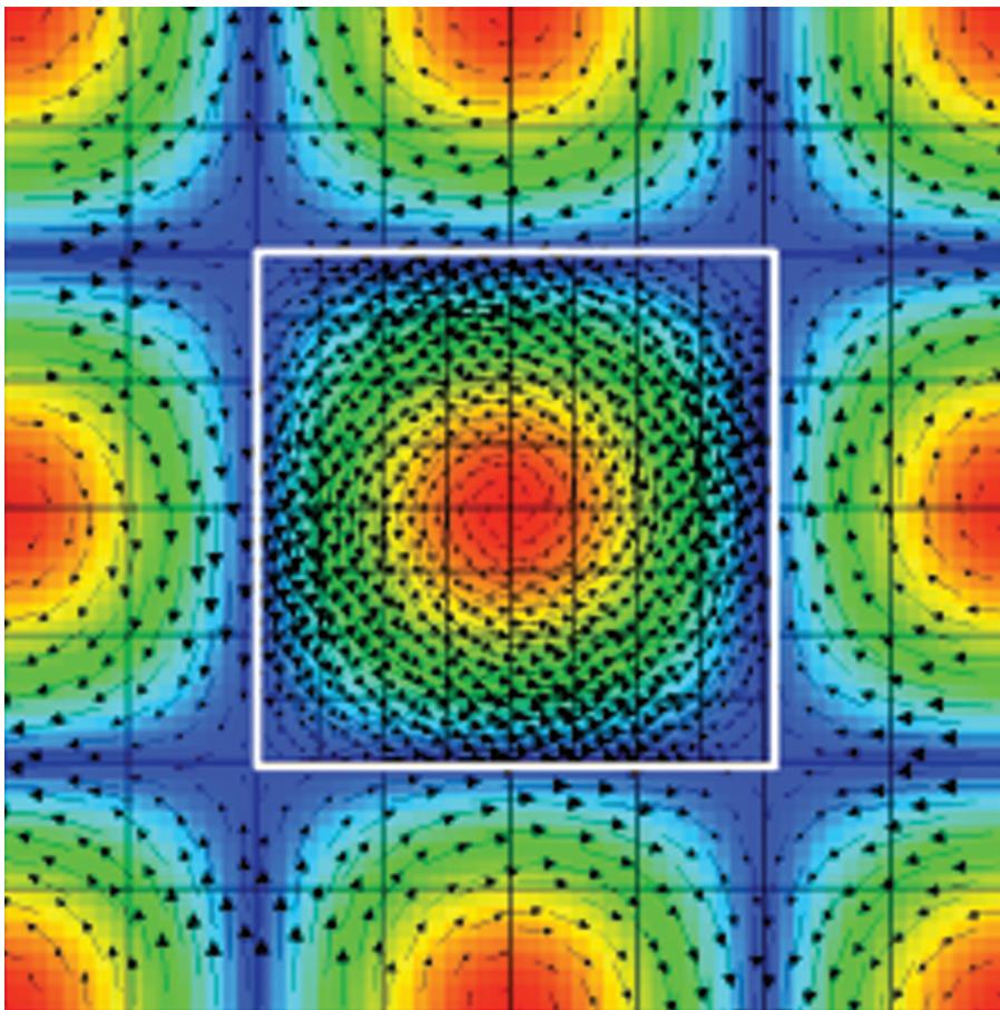
Figure 1. Taylor-Green array of 2-D counter-rotating vortices. The colors denote vorticity magnitude; the arrows depict the flow field. A finer mesh covers the central vortex within the white box.
