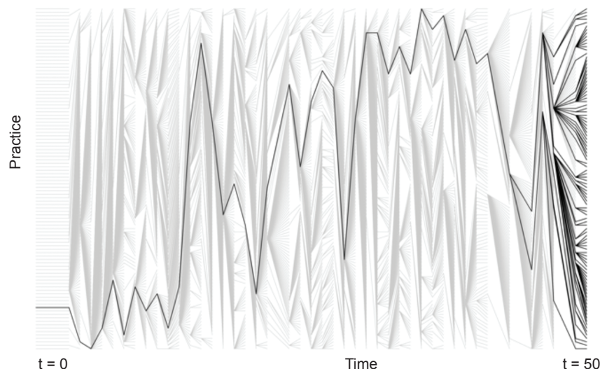
Figure 4. Genealogy of a PL. Dark lines trace the ancestry of each extant particle at time t = 50 back to a single master particle at time t = 0 .
