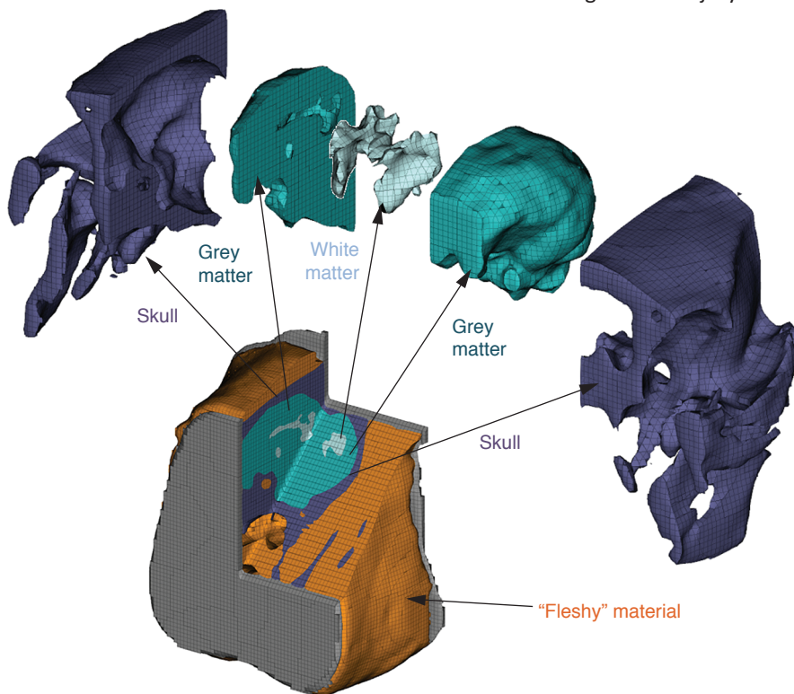
Figure 1. Regions of one pig head model, showing a moderately high fidelity brain and skull.
