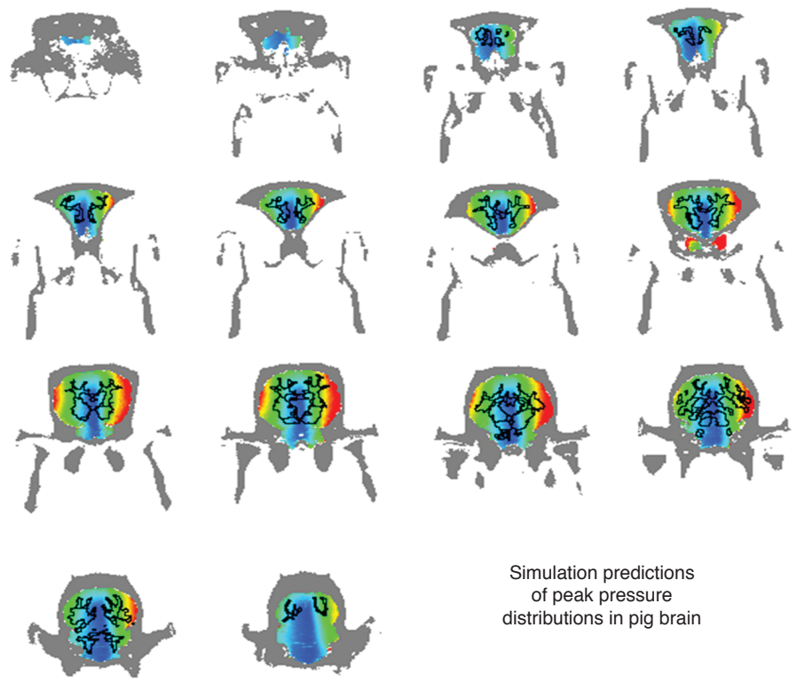
Figure 3. Typical peak pressure contours on vertical cross sections through the animal brain occurring at any time over the load history. Grey regions represent the skull. Black outlines show white matter—grey matter interface.
