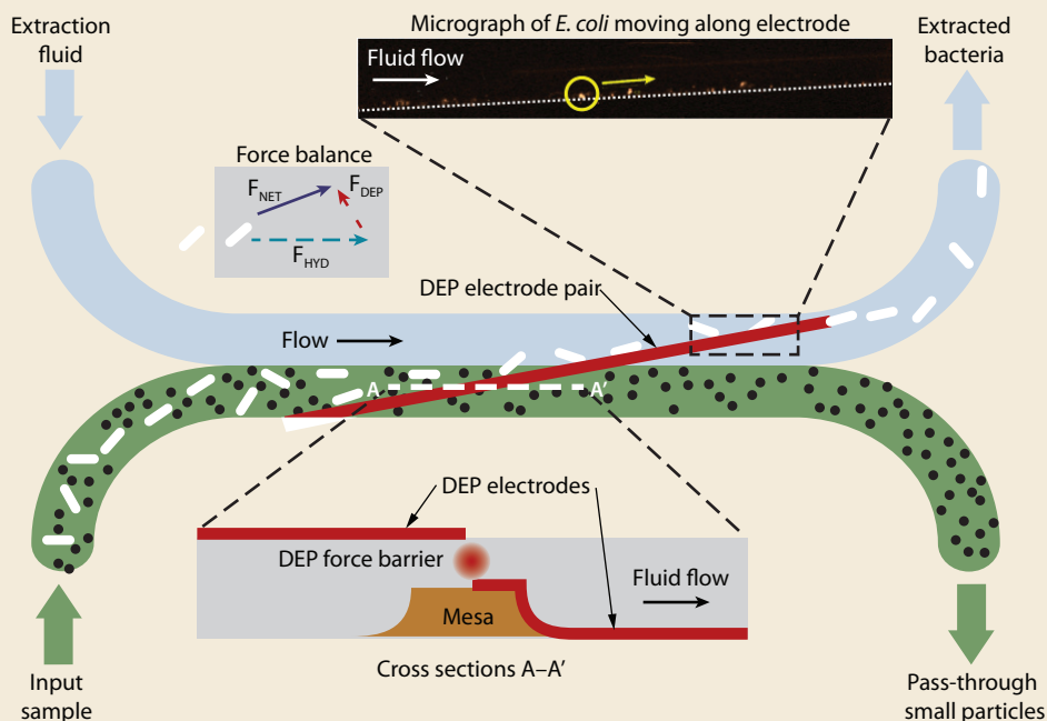
Figure 6. A schematic of LLNL's DEP device shows the angled placement and geometry of the constriction (mesa) in the fluid channel. This enables the critical balance between DEP and hydrodynamic forces that allows bacteria-size particles to be filtered out at high flow rates.
