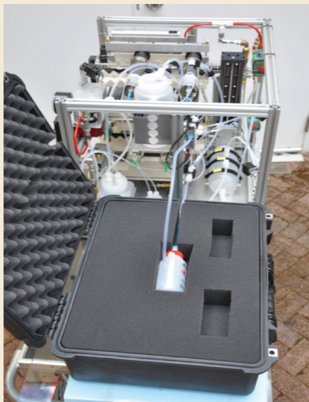
Figure 2. (top) Remote handling system used for the production of sensitive liquid explosives and Pelican case that holds the specimen that is scanned in the CT system. (right) The open Pelican case shows the specimen bottle inside that is filled with the sensitive liquid explosive prior to a CT scan.
