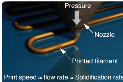
Figure 3. Process schematic of DIW, a layer-by-layer printing approach in which concentrated inks are deposited in planar and 3-D layouts with lateral dimensions (minimum ~200 nm). Paramount to this approach is the creation of concentrated inks that can be extruded through a fine nozzle as filament that then undergoes rapid solidification to maintain its shape.
