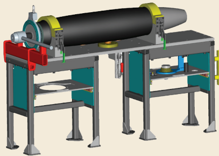
Figure 4. Manufacturing of custom assembly tooling was vital to meet warhead delivery schedule.
