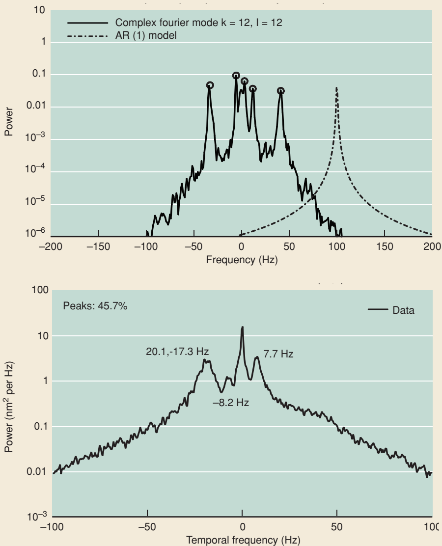
Figure 3. Each layer of frozen flow produces a distinctive peak in the temporal PSD of a Fourier mode as seen by the AO system. (top) A GPI simulation with a pure flow model of five layers. (bottom) Actual observation from the Altair AO system.
