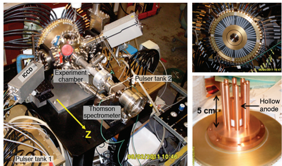
Figure 2: Photographs of 4-kJ DPF device: (left) overall experiment, including pulsed power tanks that drive the coaxial gun load at bottom right; and (top right) low-inductance cable feed system that transmits the power from the pulsers to the gun load.
