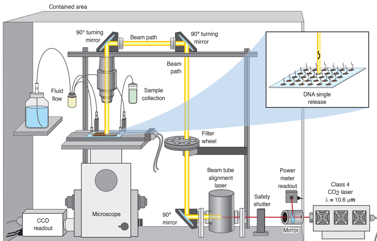
Figure 1. Schematic of laser induced DNA desorption system.
