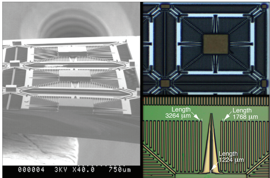
Figure 3. Rotary comb shuttles.
