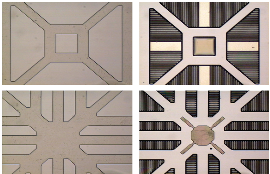
Figure 4. Back plate comb pads.
