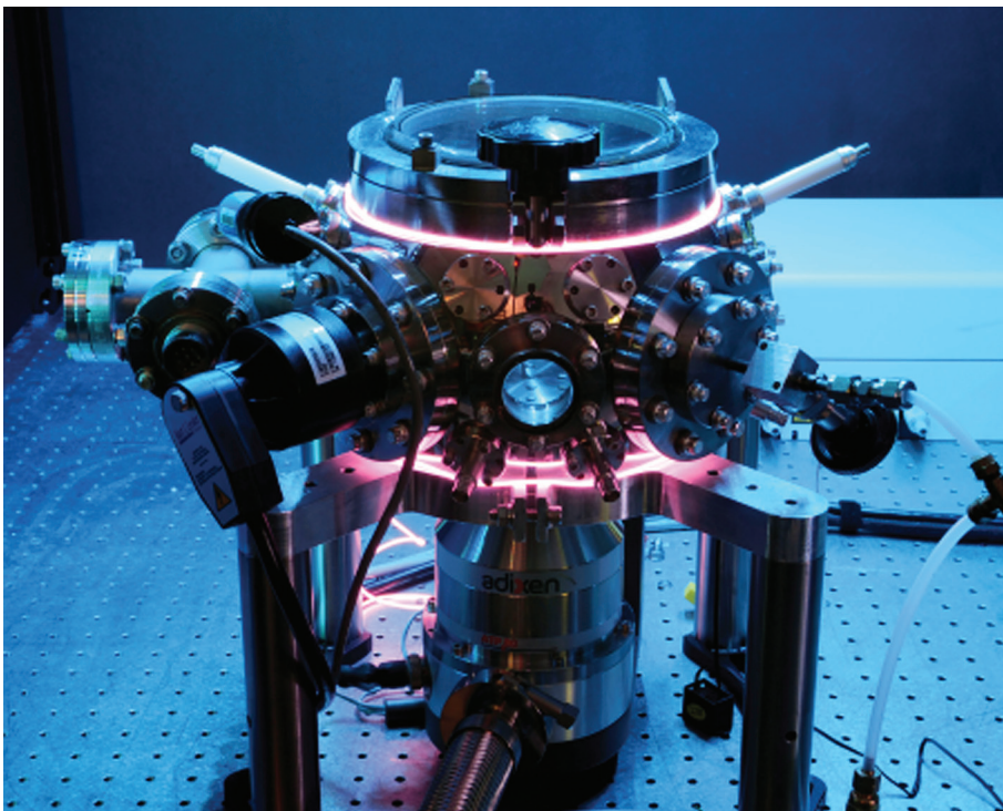
Figure 1. UHV electron optics testbed.
