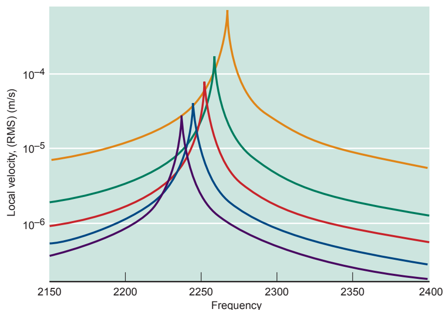
Figure 1. Comparison of output velocities (measurement signal) of tubes of different diameters.
