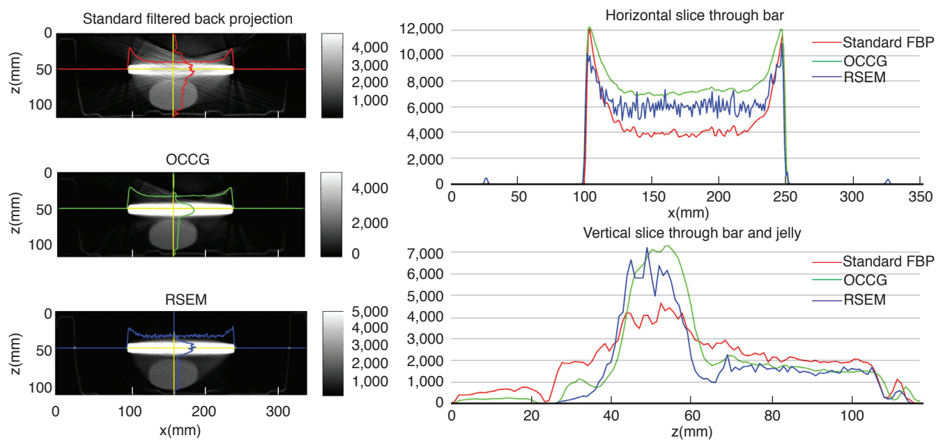
Figure 2. Reconstruction comparisons of a data set consisting of a steel bar (white object) and a container of jelly (gray ellipsoid). Profiles through the reconstructions are shown for a standard CT algorithm, an OCCG algorithm, and the RSEM.
