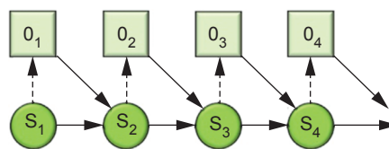
Figure 3. Graphical representation of a PDFA. PDFAs are characterized by an unknown hidden state sequence ( S_1, S_2, \dots ) that evolves not according to a Markov chain like an HMM, but deterministically conditional on the previous state and the previous observable.
