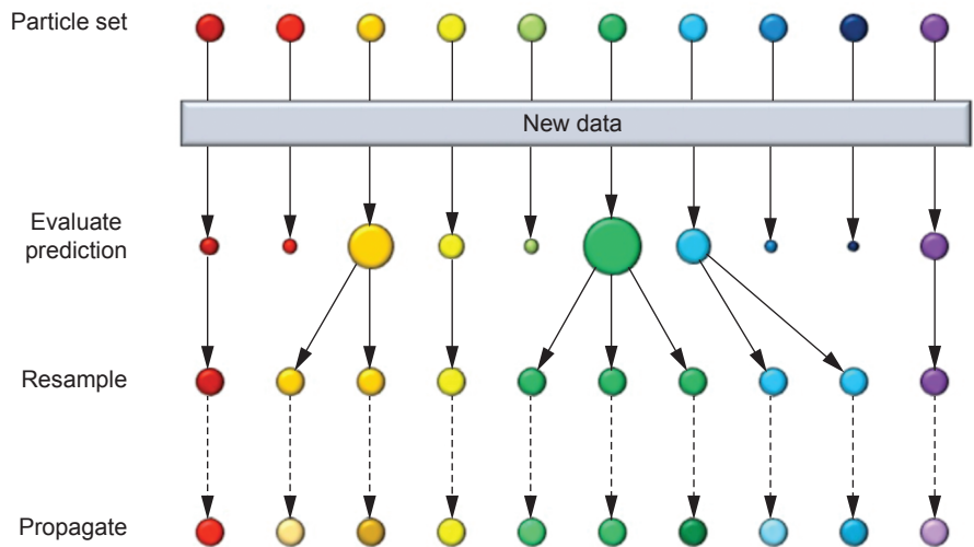
Figure 2. Schematic of the PL. PL provides full quantification of parameter uncertainty via a collection of particles that are dynamically propagated through time as data continues to arrive.
