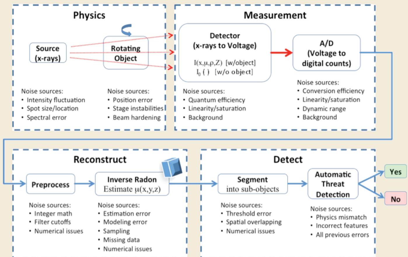
Figure 1. CT method. Images obtained from current CT-based explosives detection systems provide estimates of the linear attenuation coefficients and other features of the items inside luggage. These attenuation coefficients depend strongly on a material's density and elemental composition and on the x-ray source and detector used to measure them.
