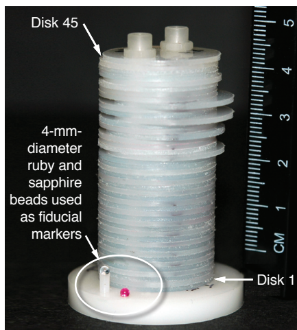
Figure 1. Contrast and Resolution Interleaved Stacked Plate (CRISP) phantom.
