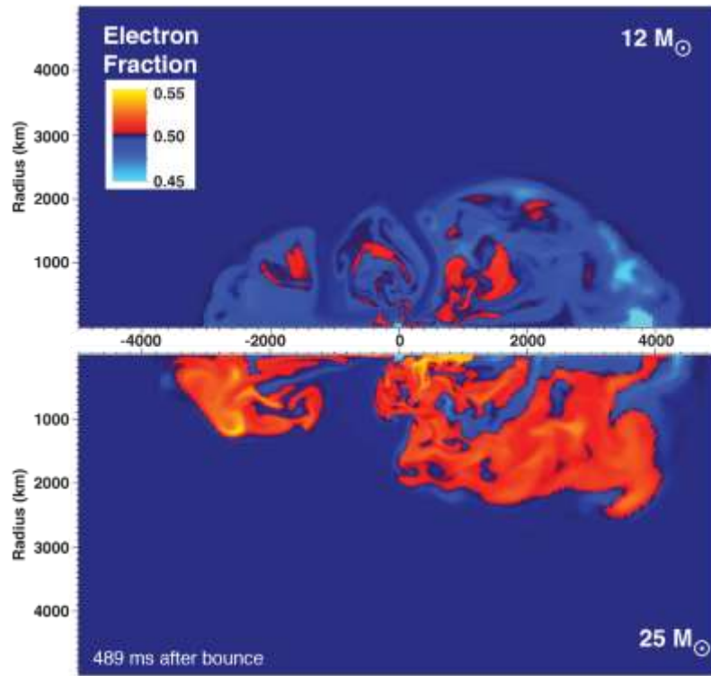
Figure 9: Neutron richness (Electron Fraction Y_e ) of the material near the center of a core collapse supernovae explosion for the explosion of a 12 (upper panel) and 25 (lower panel) solar mass star. Neutron richness is a critical parameter that determines the elements that are synthesized. The distribution is clearly not spherically symmetric and indicates that multi-dimensional models are needed to reliably determine the production of elements in supernovae. (Figure from Raph Hix)
