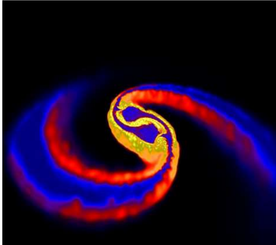
Figure 11: Multi-dimensional simulation of the merging of two colliding neutron stars into a black hole. Some material is ejected and provides a possible site of the r-process. (Daniel Price (U/Exeter) and Stephan Rosswog (Int. U/Bremen))
