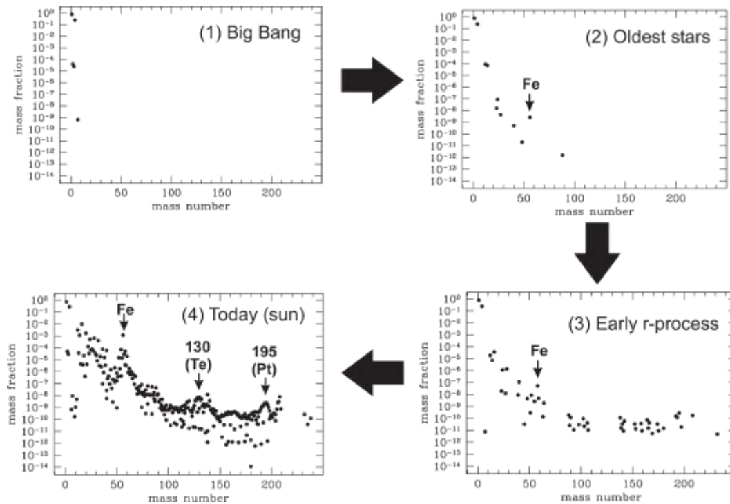
Figure 1: How did nature create the elements found today in the solar system (panel 4) from the few elements present at the time of the Big Bang (panel 1)? This is one of the key open questions nuclear astrophysics seeks to answer. Observations that for example show an emerging abundance pattern in old stars (panel 2) or r-process contributions from early explosive nucleosynthesis (panel 3) are now filling in the gaps and reveal a step by step history of the evolution of the elements. The future goal of nuclear astrophysics is to identify and understand the underlying nuclear processes and their corresponding astrophysical environments.
