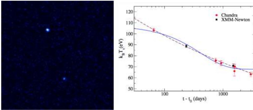
Figure 15: Transient KSI731-260, an accreting neutron star for which accretion turned off in early 2001. The faint X-ray afterglow (left) is believed to be from the heated neutron star crust, and its decrease in temperature over many months has been observed (see graph on the right). Such observations can reveal the inner structure of the neutron star crust, once the nuclear processes that heat and cool the crust are understood. This is a major goal of the field. (Image credit left: NASA/Chandra/Wijnands et al., Figure right from A. Turlione et al. arXiv:1309.3909 )
