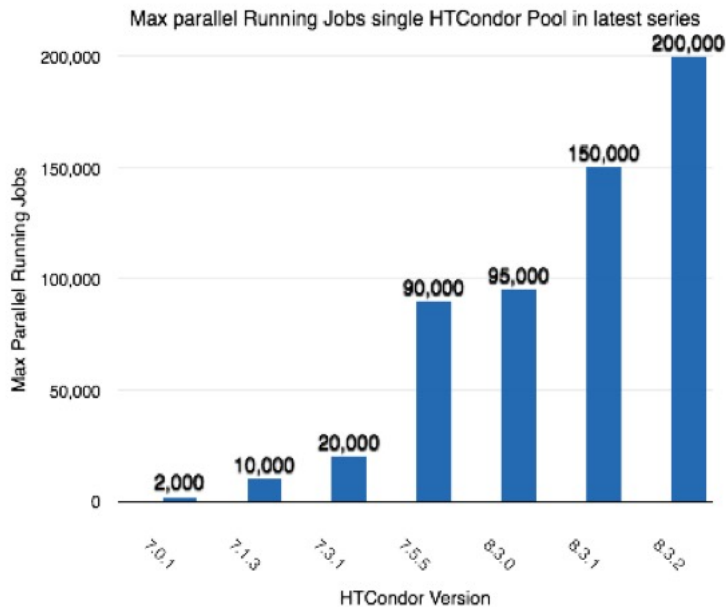
Figure 7. The maximum running parallel jobs for some HTCondor versions. This is a combination of results from [13], [8] and Figure 3. Bear in mind this tests were performed by different people with different hardware and are presented here as a vision of the expanded capabilities of the software.
