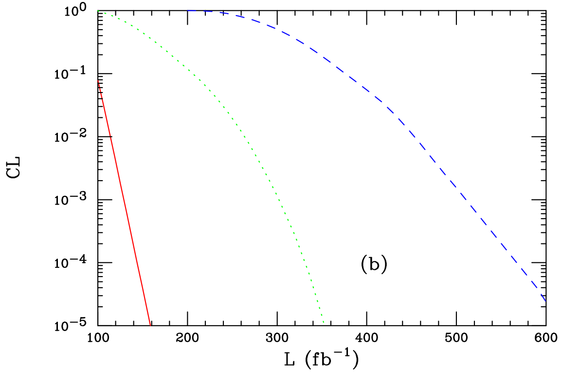
Figure 5: CL as a function of the integrated luminosity resulting from the coupling fits following from the analysis discussed in the text for both (a) a 500 GeV or a (b) 1 TeV e^+e^- collider. In (a) the solid(dash-dotted,dotted) curve corresponds to a first KK excitation mass of 4(5,6) TeV. In (b) the solid(dotted,dashed) curve corresponds to a first KK mass of 5(6,7) TeV.
