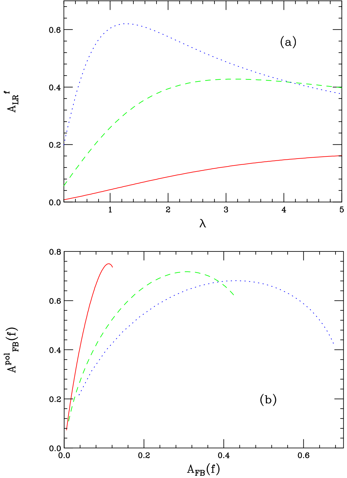
Figure 6: (a) A_{LR}^f as a function of the parameter \lambda for f = \ell (solid), f = c (dashed) and f = b (dots). (b) Correlations between on-peak observables for the same three cases as shown in (a). \lambda varies from 0.2 to 5 along each curve.
