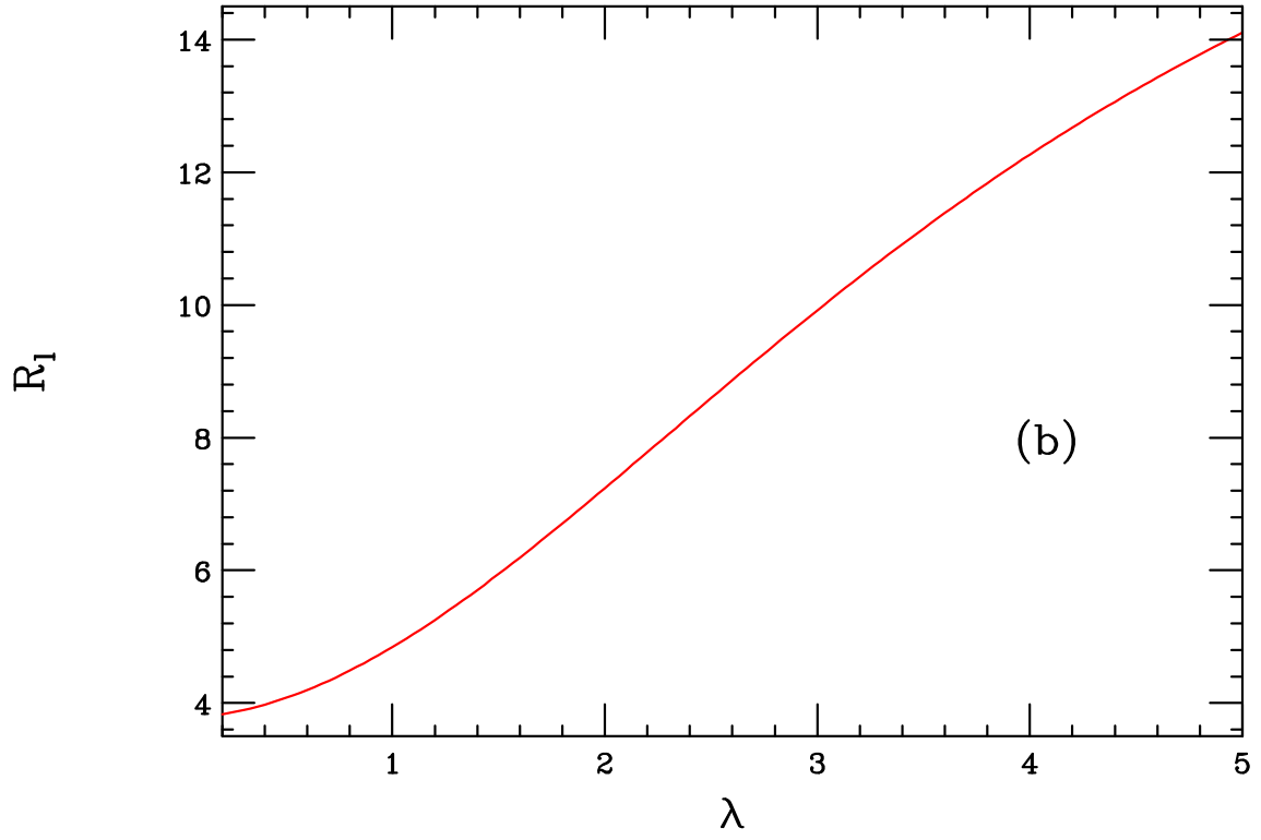
Figure 8: (a) The ratios of the \bar{b}b (dots) and \bar{c}c cross sections to that for all hadrons on top of the 4 TeV KK excitation. (b) The ratio of the hadron cross section to that for leptons on the peak of the KK excitation.
