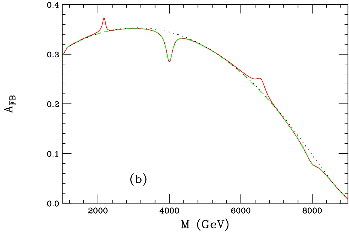
Figure 2: Same as the previous plot for the case of 1/R = 4 TeV (solid) but now also showing both the SM result for comparison (dots) as well as the alternative excitation curve for the case where the naive couplings are altered as in the scenario of Arkani-Hamed and Schmaltz (dashed) [7].
