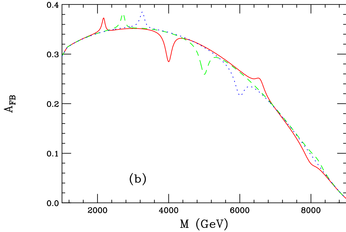
Figure 1: (a) Cross section and (b) Forward-Backward asymmetry for Drell-Yan production of the degenerate neutral KK excitations Z^{(n)} and \gamma^{(n)} as a function of the dilepton invariant mass at the LHC assuming one extra dimension and naive coupling values with 1/R=4(5, 6) TeV corresponding to the solid(dashed, dotted) curve. The second excitation is only shown for the case of 1/R = 4 TeV.
