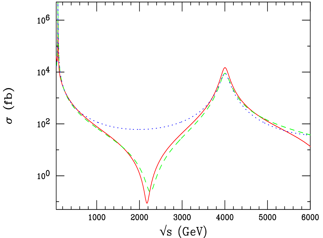
Figure 9: Cross sections for e^+e^- \rightarrow \mu^+\mu^- (solid) and b\bar{b} at high energy lepton colliders. The solid curve applies in both the ‘conventional’ scenario and that of Arkani-Hamed and Schmaltz[7]. The dashed curve correspond to the case of ‘conventional’ couplings for the b ’s while the dotted curve is for the case of the Arkani-Hamed and Schmaltz scenario.
