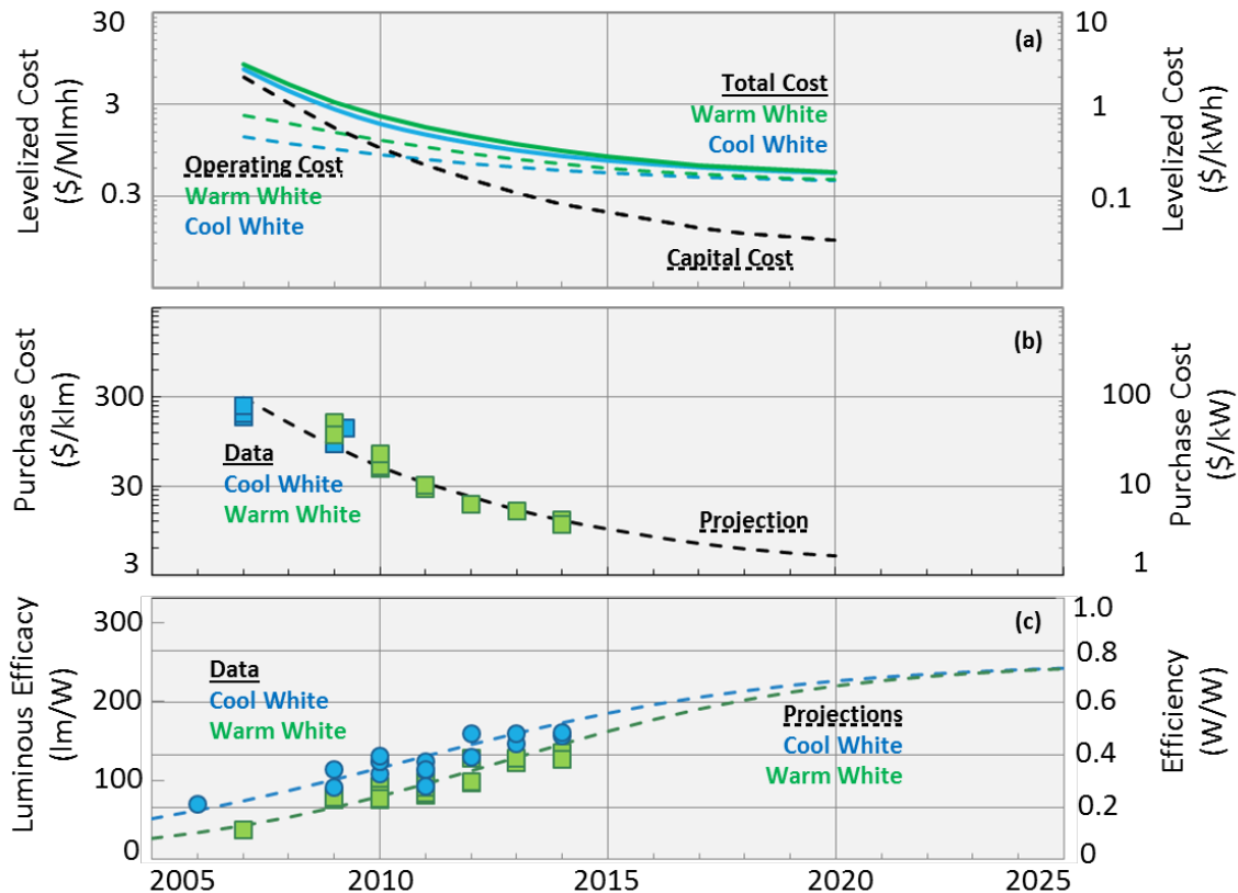
Figure 2. History and projections of SSL for humans: (a) levelized costs (total, capital and operating), (b) lamp cost, and (c) efficiency. Data and projections taken from the U.S. Department of Energy Solid-State Lighting Research and Development Plan (2015). Levelized costs were calculated from capital (purchase) and operating costs using a 50,000 hour lifetime. Left and right axes units were scaled using a 2015 state-of-the-art luminous efficacy of radiation of 331 \text{lm}/\text{W} . Similar projections can be anticipated for horticultural lighting (SSL for plants).
