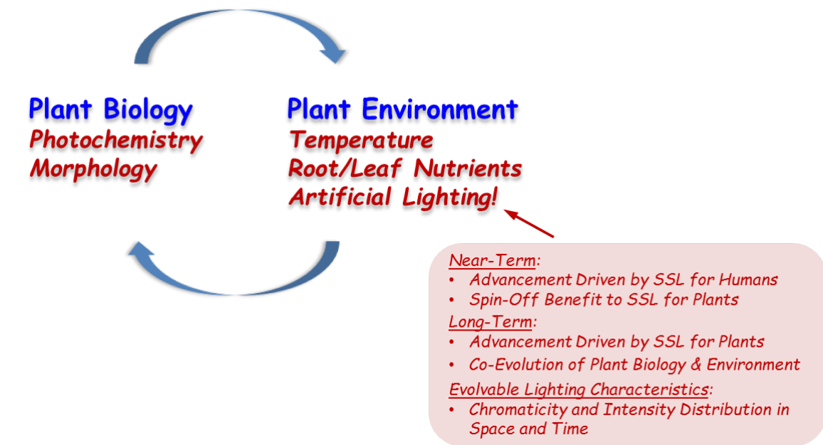
Figure 4. Schematic of how plant biology (including photochemistry and morphology) and plant environment (including temperature, root/leaf nutrients and artificial lighting) might co-evolve. Artificial lighting, in turn, will evolve in response to the needs of both SSL for humans and SSL for plants.
