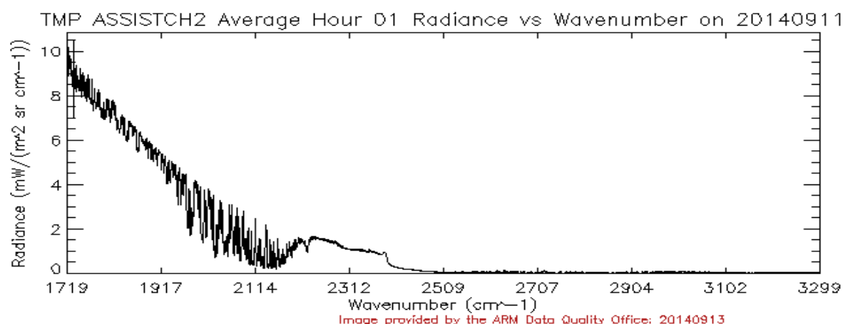
Figure 2. ASSIST InSb Channel 2 hourly-averaged zenith radiance for 2014-09-11.
