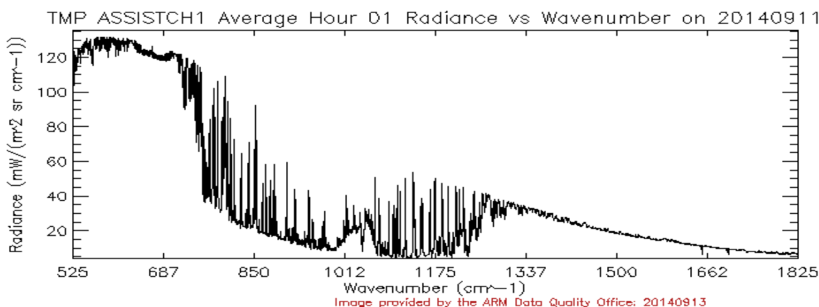
Figure 1. ASSIST MCT Channel 1 hourly-averaged zenith radiance for 2014-09-11.
