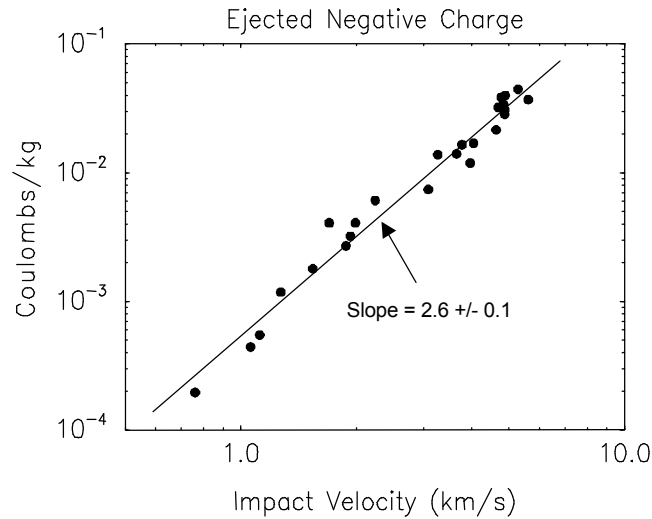
Fig. 1. Negative charge per unit projectile mass ejected by impacts of spherical aluminum projectiles into granular carbonate (dolomite) targets vs. impact velocity, from [1].
