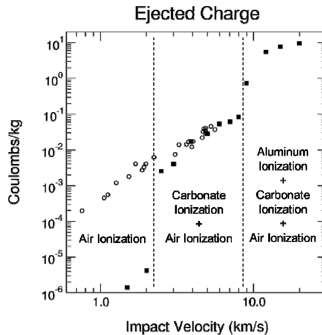
Fig. 6. Total negative charge per unit mass ejected vs. impact velocity. Experimental results from [9] are shown with open black circles. CTH simulation results using the model described in the text are shown with solid black squares. Good agreement between experiments and simulations is seen in the carbonate vaporization (and ionization) regime. The lack of agreement at low velocities, where simulations predict only air ionization to contribute, is discussed in the text.
