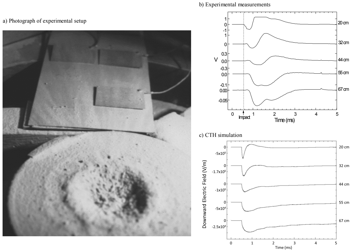
Fig. 4. Experiment to measure the electrostatic field produced by the impact of a 0.64 cm aluminum projectile into a particulate carbonate target (impact velocity: 5 km/s, vertical), from [9]. a) The impact crater (10 cm diameter) can be seen in the foreground and several of the plates located 20 and 32 cm from the impact are shown in the background. b) The voltage measured on plates distributed radially from the impact point is shown with distance from the center of the impact crater indicated. c) CTH simulation of the downward component of the electric field (V/m) at the same experimental locations and shifted in time to correspond to the experimental impact time of ~0.5 ms.
