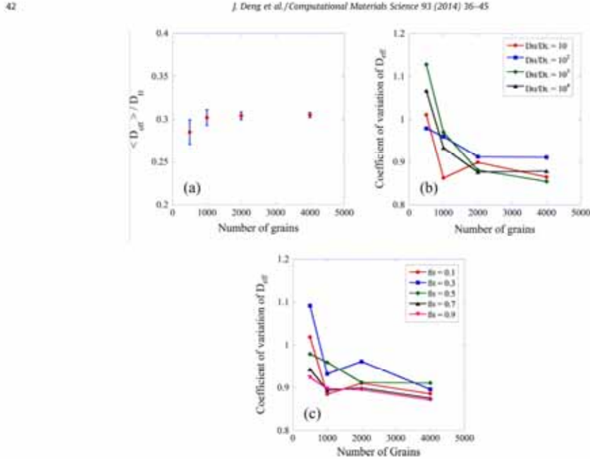
Fig. 4. (a) \langle D_{eff} \rangle with error bar (estimated by the standard deviation divided by the mean) as a function of the system size when \frac{D_H}{D_L} = 1000 and f_H = 0.5 . Coefficient of variation of D_{eff} as a function of the system size for (b) different values of \frac{D_H}{D_L} when f_H = 0.5 and (c) different values of f_H when \frac{D_H}{D_L} = 100 .
