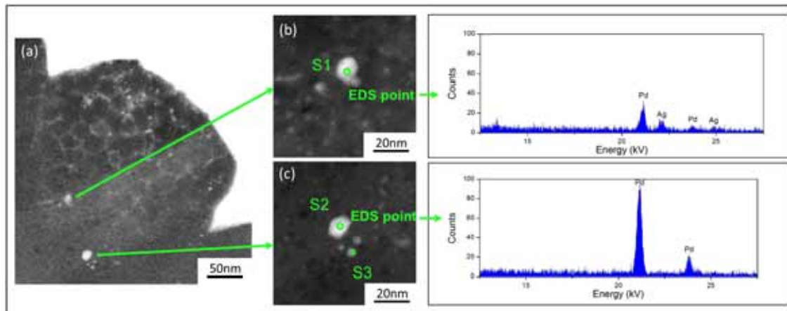
Figure 3.13 (a) Different types of nano-precipitates identified inside a SiC grain (position1 in Fig. 3.12(a)), (b) EDS spectrum indicates S1 is a Pd-Ag precipitate and (c) EDS spectrum indicates S2 is a Pd-rich precipitate.
