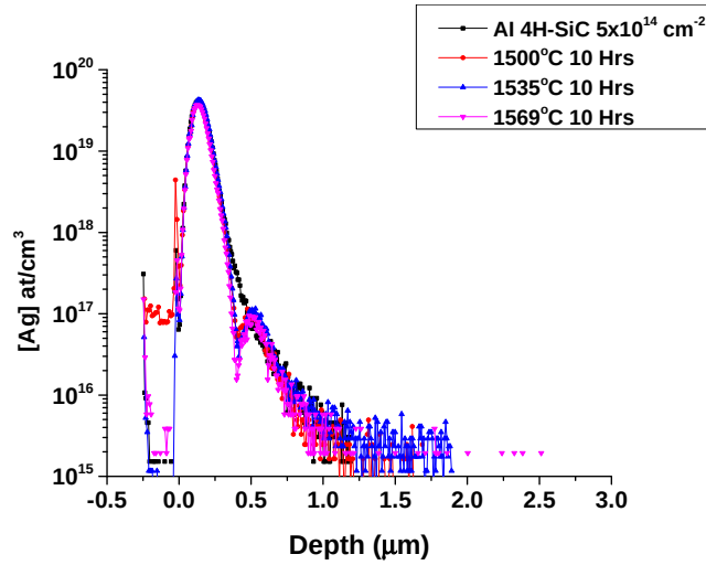
Figure 2.6 SIMS depth profiles of Ag in SiC for single crystal 4H-SiC (dose of 5 \times 10^{14} ions/cm 2 ) in AI condition followed by 1500-1569°C 10 hours isochronal exposures identifying redistribution of Ag past the primary implantation peak.
