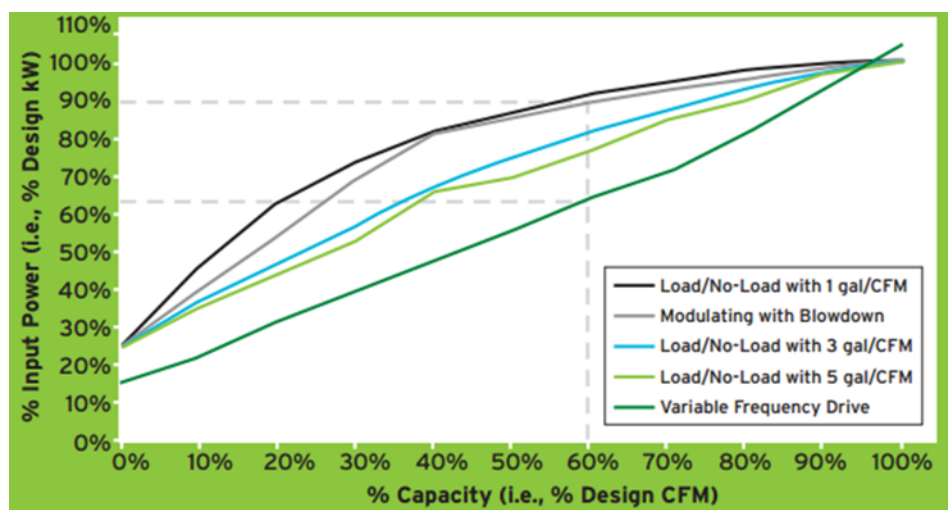
Figure 4. Input power at partial load by compressor type for various compressed-air systems
