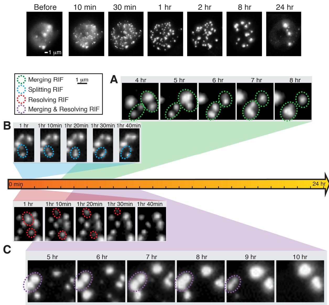
Fig. 3. RIF dynamics in live cell imaging shows elastic and inelastic collisions. Immortalized non-malignant MCF10A human breast cells expressing 53BP1-mCherry [84] were imaged at different time points after IR (2.3 Gy). Following time-lapse, Z-stacks were collapsed to a 2D image set using maximum intensity projection, and registered to correct for nuclear motions. RIF movements are highlighted in zoomed sub-panels that illustrate various collision scenarios where RIFs merge (inelastic collision, (A)), split (B) or simply resolve (C). Notably, merged RIFs get larger, brighter and take longer to get resolved.
