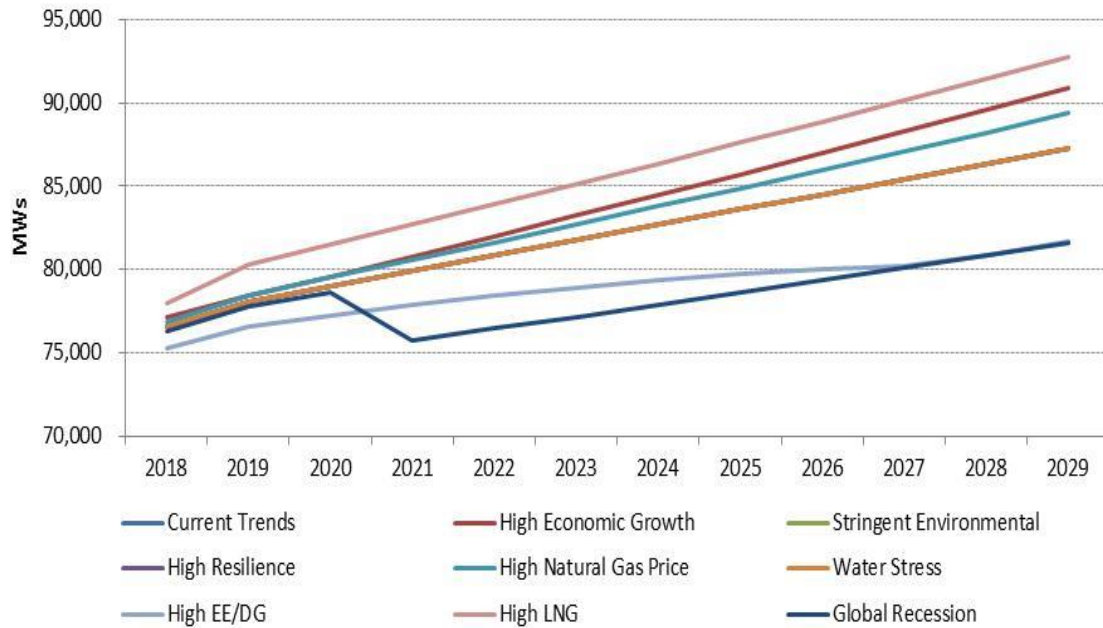
Fig. 11. Peak load forecasts for ERCOT long-term system assessment scenarios. Source: ERCOT.
