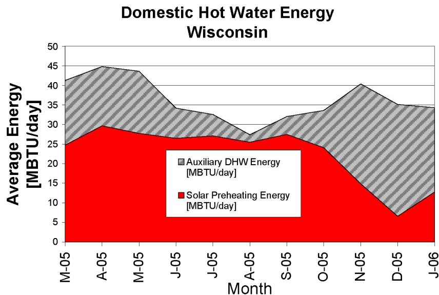
Figure 2. Performance summary of hot water systems in a Wisconsin home
