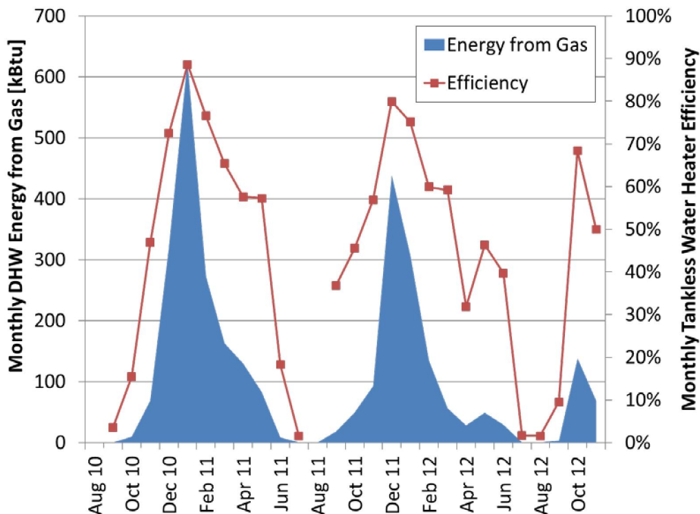
Figure 7. Thermal energy from the gas tankless water heater and water-heater efficiency
