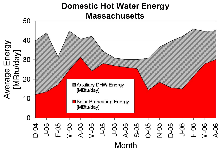
Figure 1. Performance summary of hot water systems in a Massachusetts home
