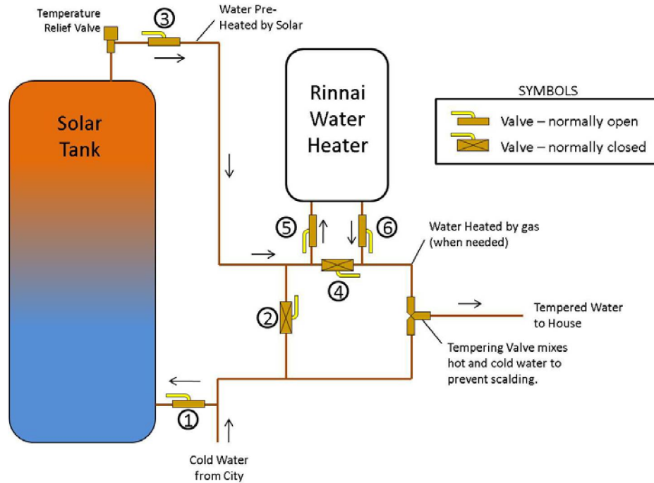
Figure 4. Schematic of water-heating system from homeowner's manual
