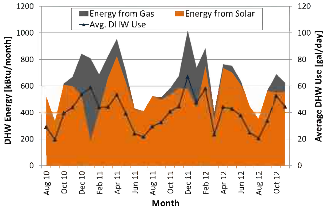
Figure 6. Overview of DHW consumption and water-heating energy
