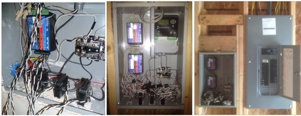
Figure 8. Panel containing time clock-contactors-CTs for switchback and monitoring
