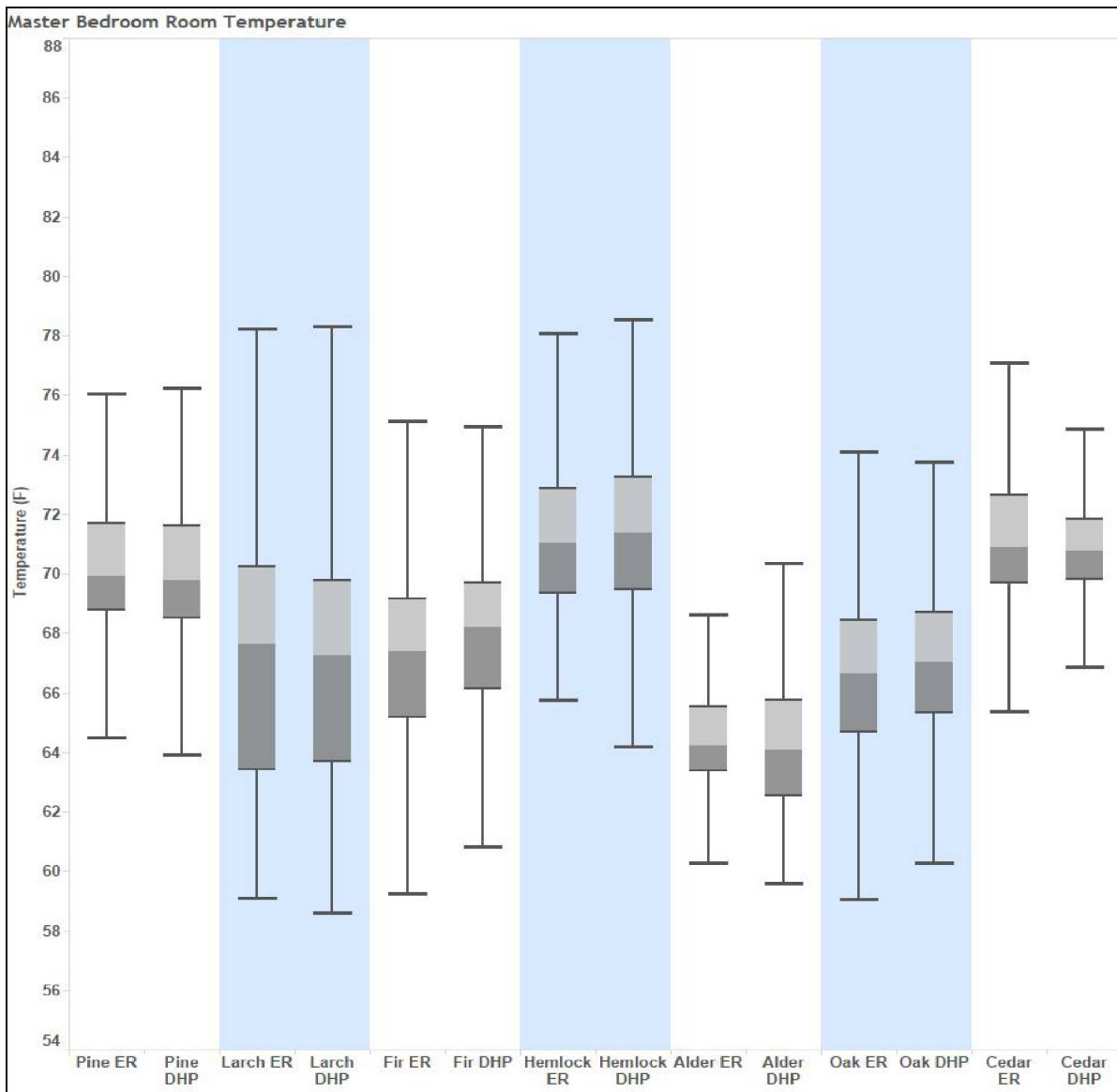
Figure 19. Master bedroom indoor temperatures for each house in ER and DHP heating modes
