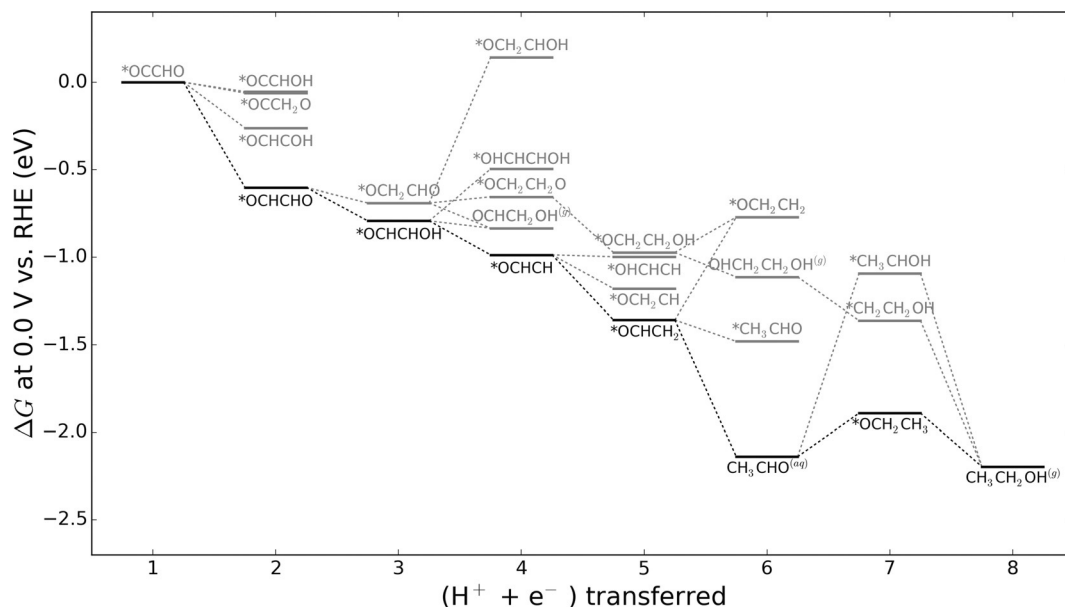
Figure 4. Free energy diagram for reduction of C–C coupled intermediate ^*\text{OCCHO} on Cu(211). The free energy for \text{CH}_3\text{CH}_2\text{OH}^{(a)} was calculated at 1 bar and the free energy of \text{CH}_3\text{CHO}^{(aq)} was calculated at a concentration of 100\ \mu\text{M} . The steps marked with black represent the thermodynamically most favorable pathway. The gray represent other potential intermediates of higher energy.
