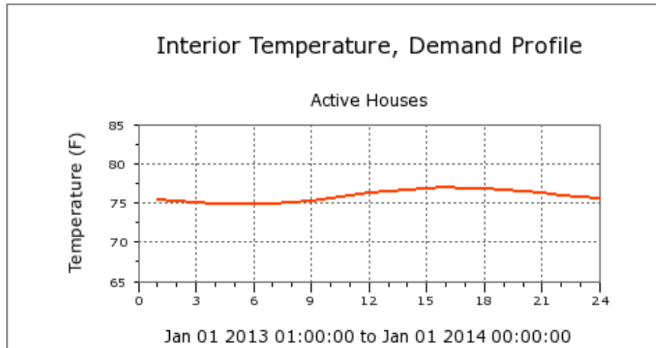
Figure 93. Average interior temperature profile during 2013
