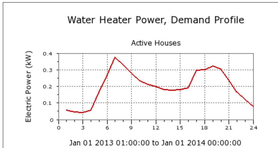
Figure 63. Average water heater load shape during 2013
