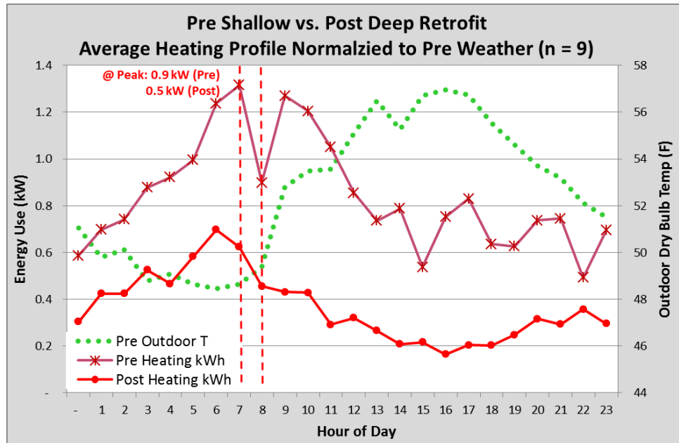
Figure 51. Pre- retrofit (shallow) versus post-retrofit (deep) hourly space heating profile, pre-retrofit weather-normalized
