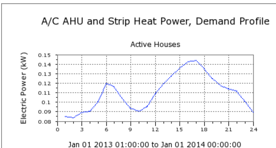
Figure 57. Average AHU and strip heat electricity load shape during 2013
