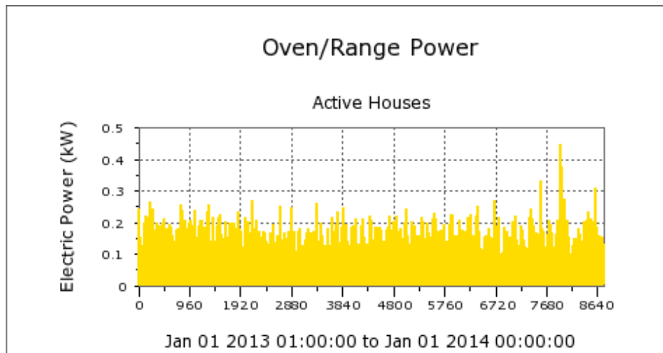
Figure 68. Average hourly oven/range electricity in overall sample
