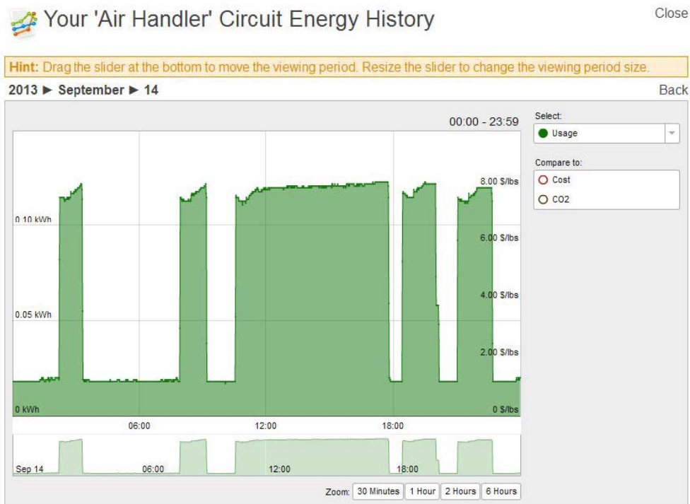
Figure 130. Site 40 AHU operation reflecting Stage 2 only condition
