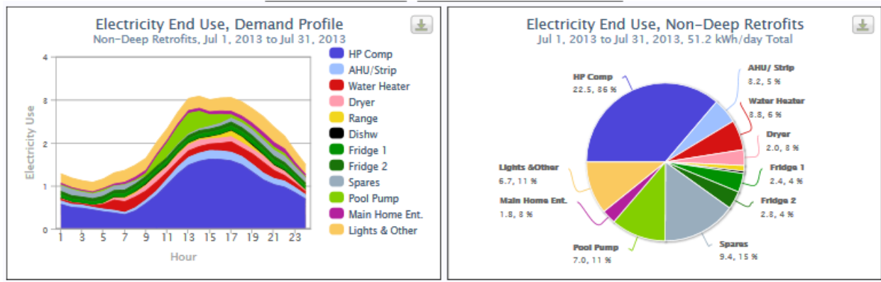
Figure 104. Electricity end uses, July loads
