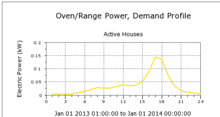
Figure 69. Average range/oven load shape during 2013
