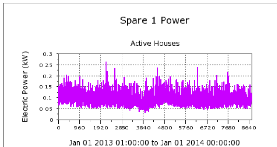
Figure 80. Average hourly Spare 1 electricity in overall sample
