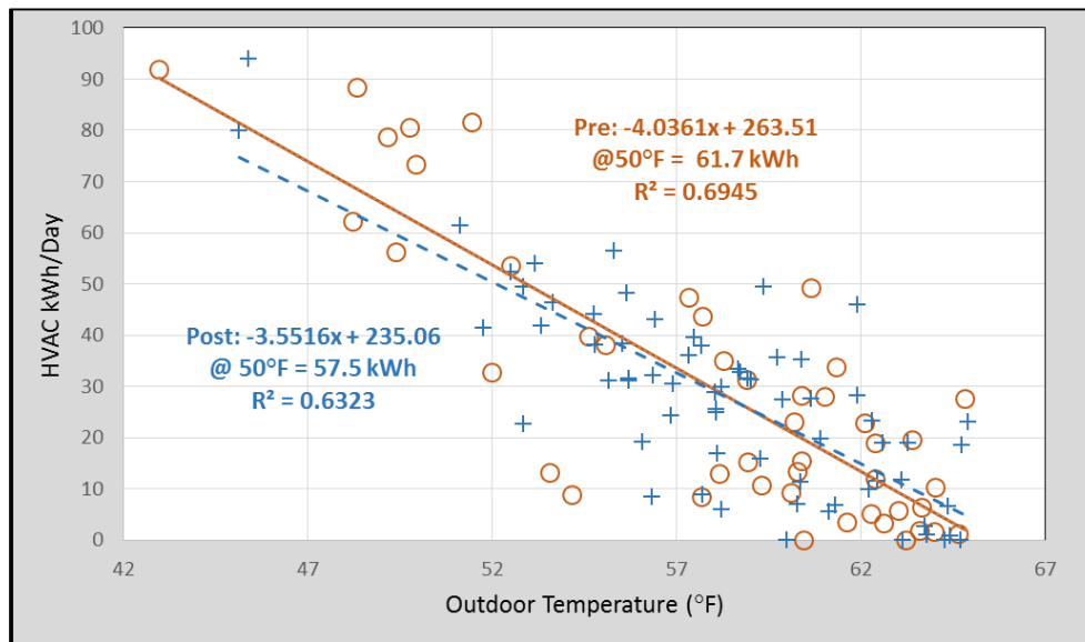
Figure 24. Site 23 pre- and post-window retrofit daily average space heating consumption versus outdoor temperature
