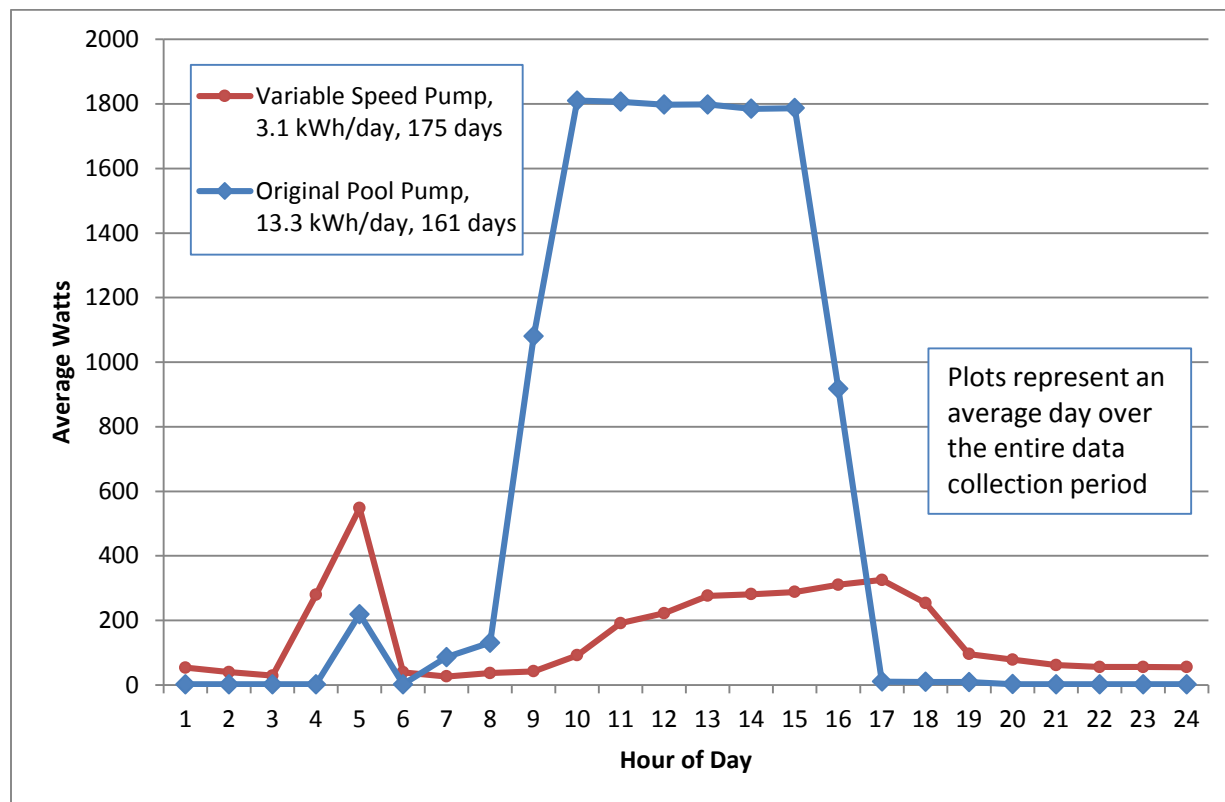
Figure 53. Average time-of-day pool pump demand at Site 50 as originally found (blue) and after variable speed pump retrofit (red)
