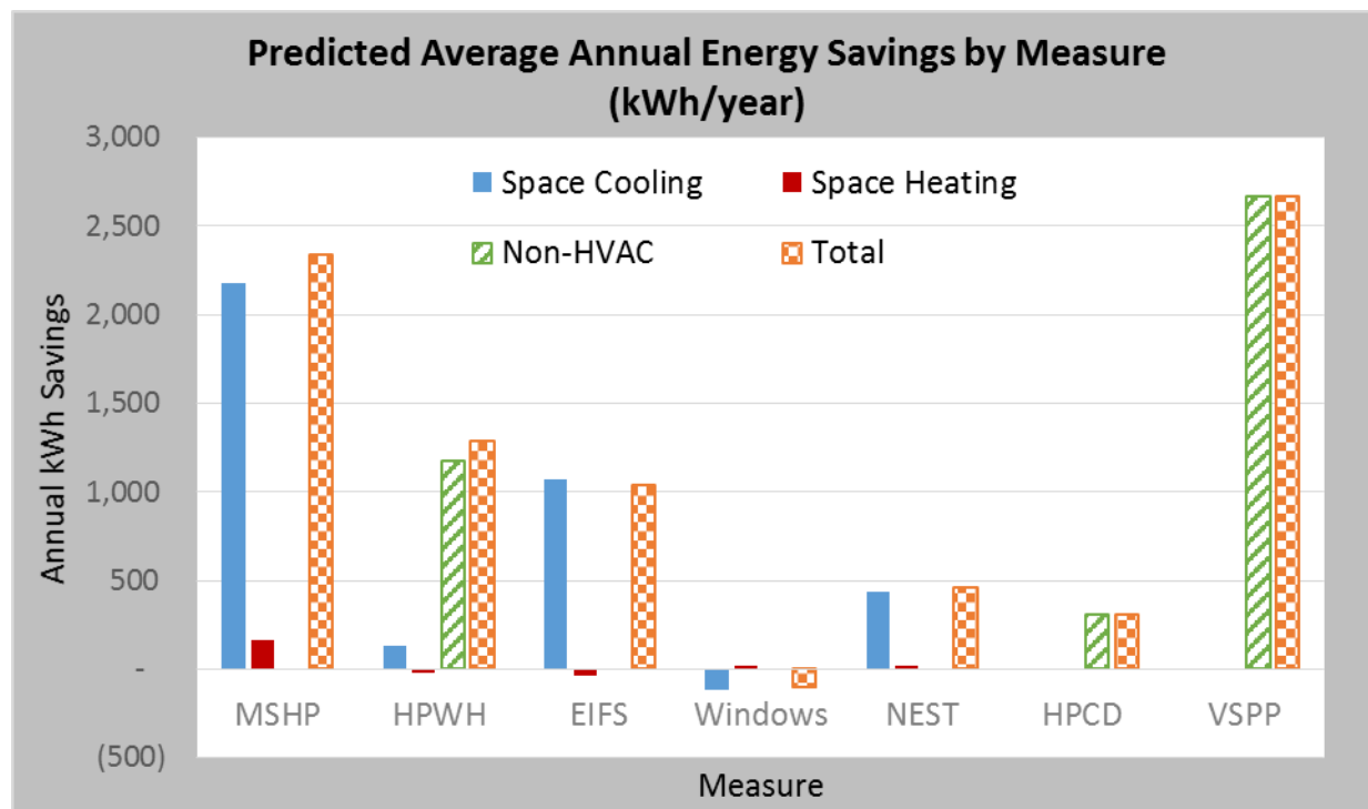
Figure ES-1. Average annual energy savings for the Phased Deep Retrofit Phase II evaluation measures
