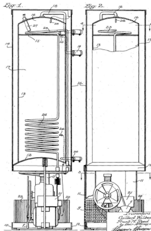
Figure 21. First patented HPWH. Image from Wilkes and Reed 1937.
