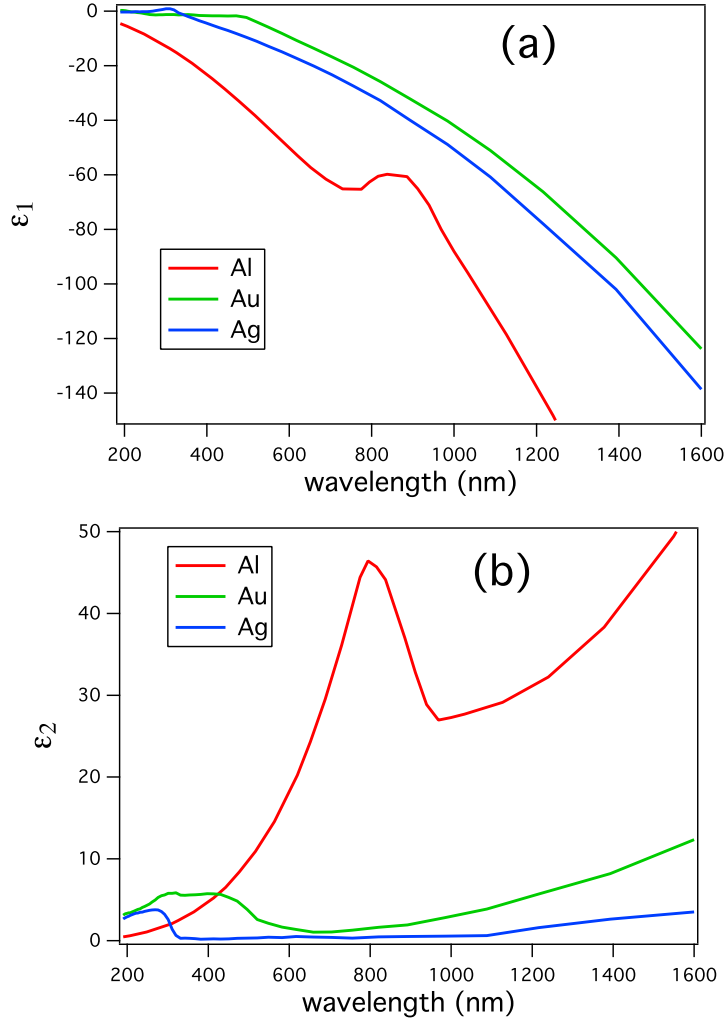
Figure 1. Real part (a) and imaginary part (b) of the dielectric functions for aluminium, gold and silver. Data from [29] (for Al) and from Johnson and Christy [30] (for Au and Ag).
