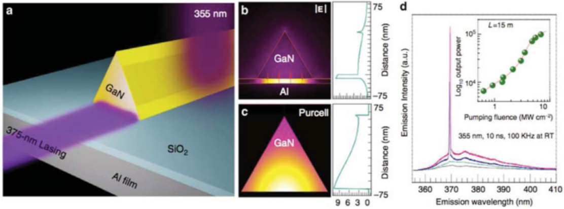
Figure 7. Ultraviolet plasmonic nanolaser. (a) Schematic of the structure. (b) Finite-element method calculation of the absolute electric field |E| around the device at \lambda = 370 nm, showing the high degree of energy confinement inside the insulator layer. Red arrows indicates the electric field direction. (c) Calculated Purcell factor distribution inside the GaN nanowire. (d) Experimental characterization of the laser emission: power-dependent emission spectra of the device, showing the appearance of a sharp peak above the spontaneous emission background. Inset: integrated emission as a function of the pumping intensity. Reprinted from [67] by permission from Macmillan Publishers Ltd, copyright 2014.
