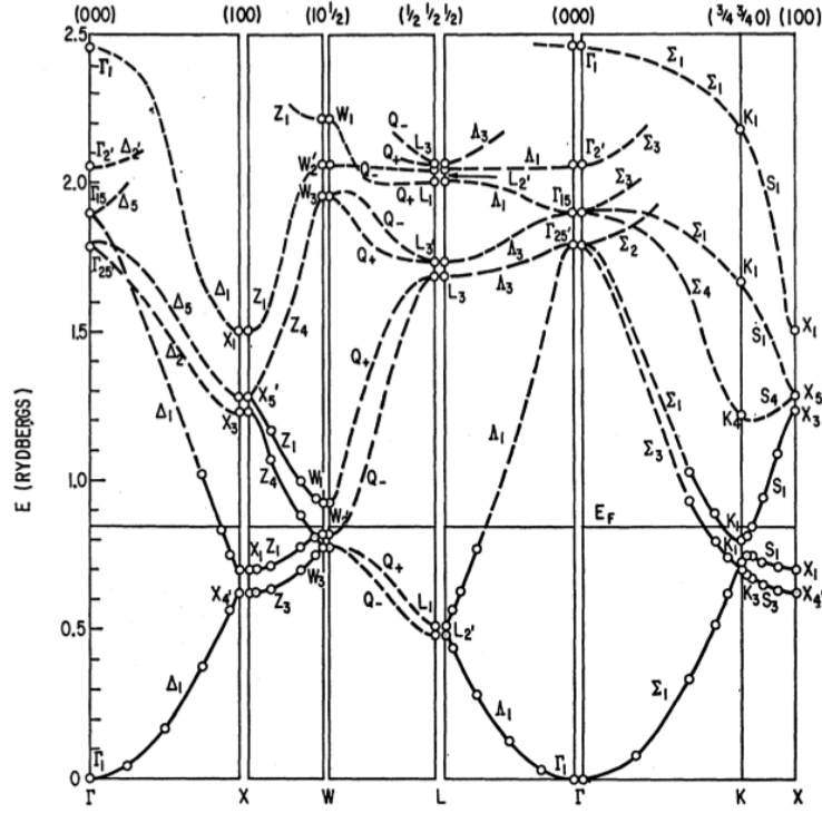
Figure 2. Calculated band structure of aluminium along the symmetry axes. Reprinted from [32]. Copyright 1963 by the American Physical Society.
