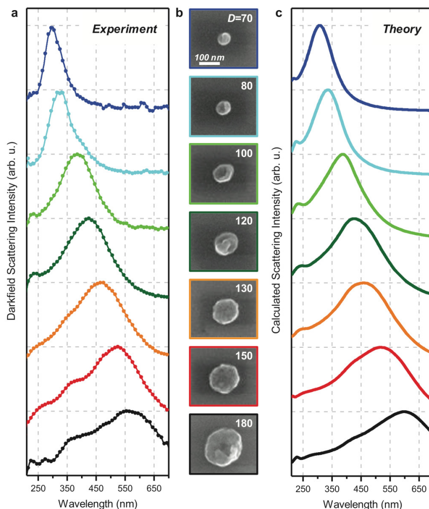
Figure 4. Tuning of the LSP resonance of Al nanodisks fabricated using e-beam lithography. (a) Experimental scattering spectra of individual nanodisks with varying diameters. ( D = 70, 80, 100, 120, 130, 150, 180 nm) (b) SEM images of the corresponding nanodisk structures. Scale bar is 100 nm. (c) Finite-difference time-domain (FDTD) simulations of the scattering spectra, assuming a 3 nm surface oxide and a \text{SiO}_2 substrate. Reprinted with permission from [17]. Copyright 2014 American Chemical Society.
