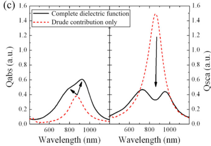
Figure 5. Calculated absorption cross-section (left panel) and scattering cross-section (right panel) of Al nanorods, using Eq. 4. Adapted with permission from [40]. Copyright 2014 American Chemical Society.
