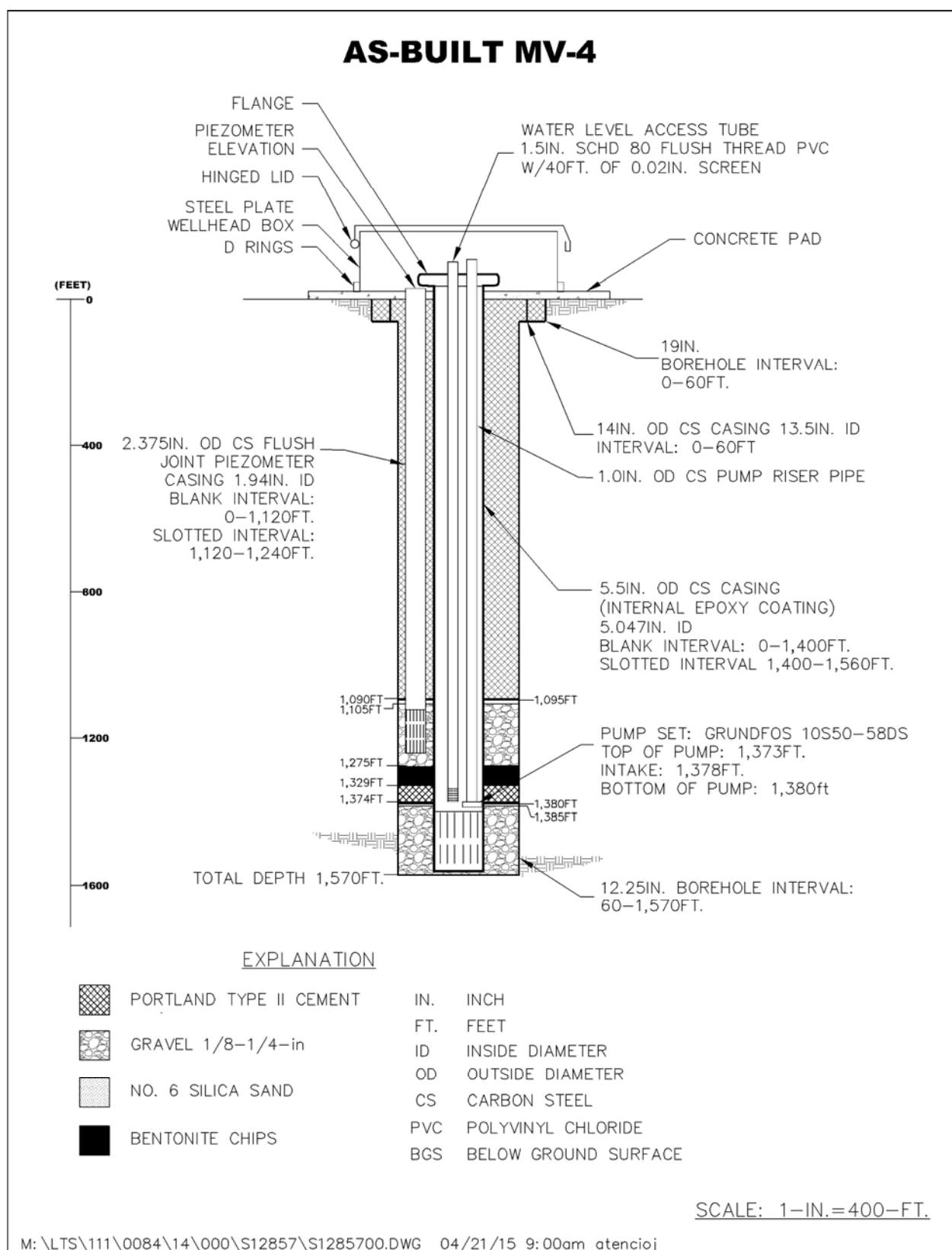
Figure 8. As-Built Completion Diagram of MV-4
